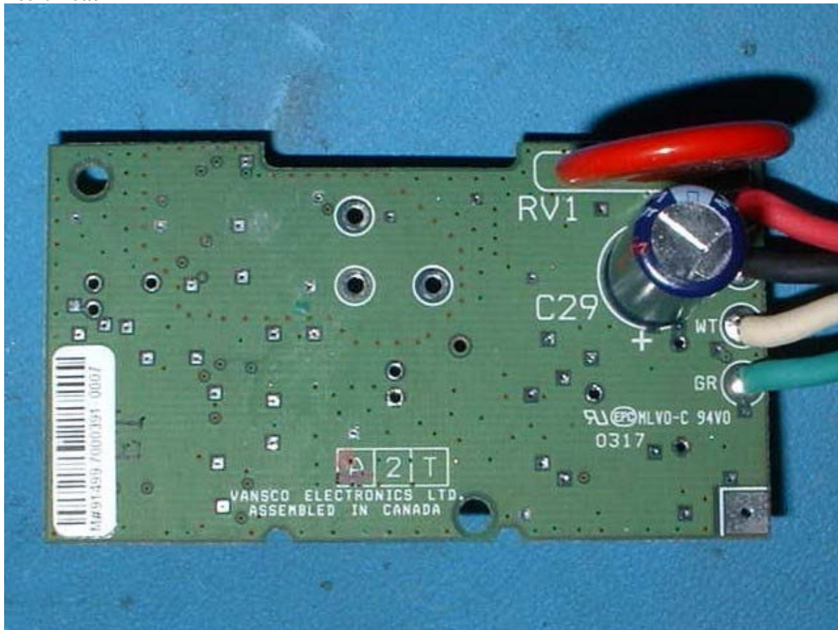
Board Bottom
