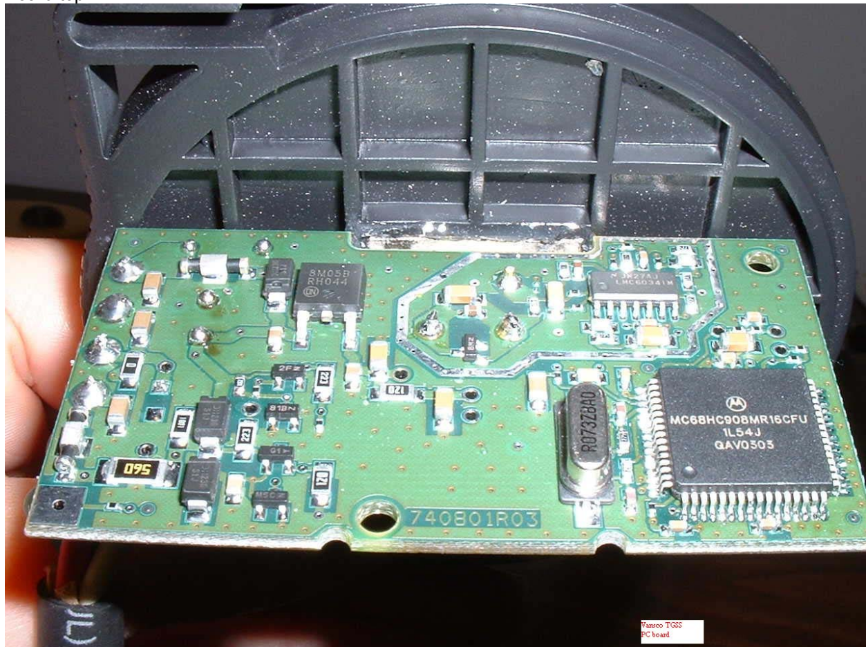
Board top
