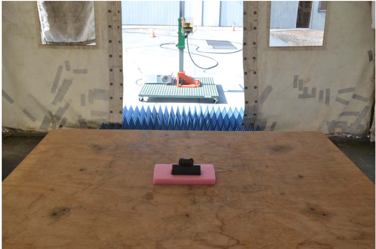
Radiated Emissions Setup (>1 GHz) Model: i750TC | NS118111
