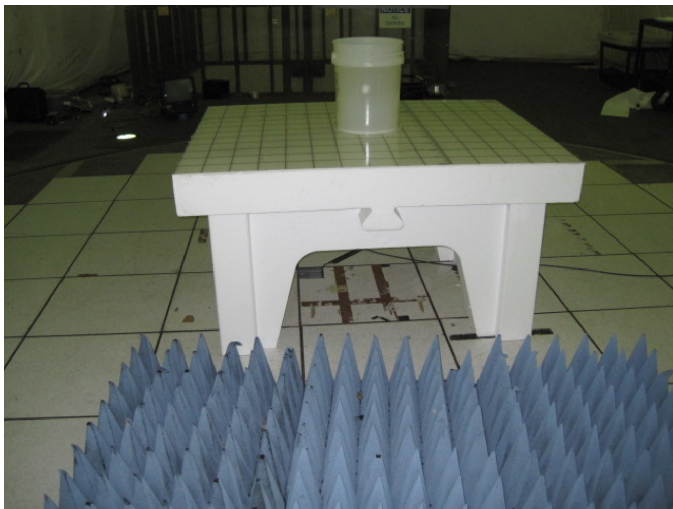
Test-setup photo(s): Radiated emissions above 1 GHz
