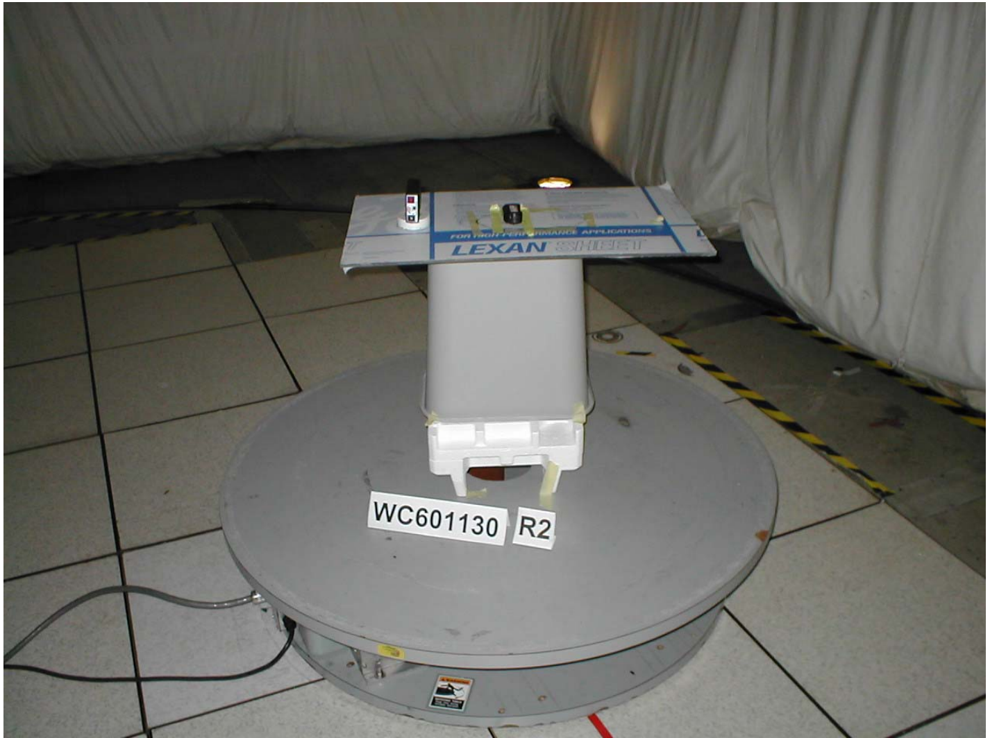
Test setup photo, radiated emissions Repeater RPT-910-3
