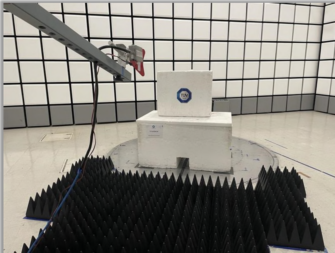
Radiated Emissions Test Setup (1GHz to 18GHz)
