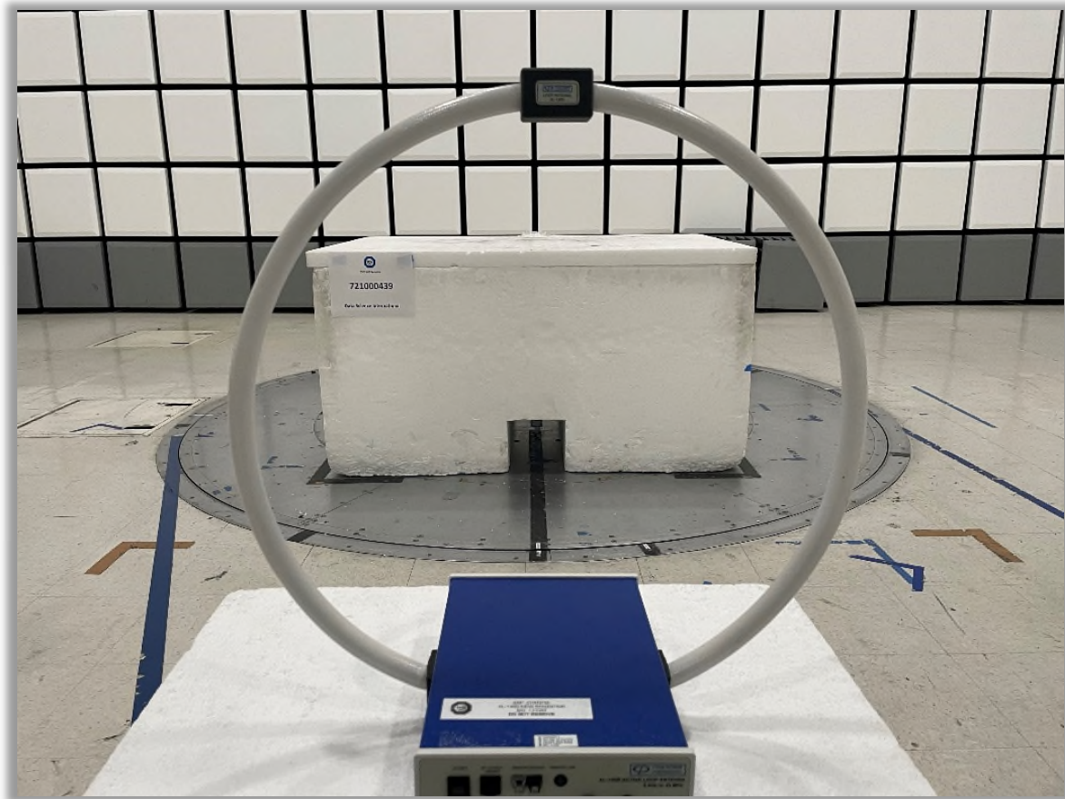
Radiated Emissions Test Setup (9kHz to 30MHz)
