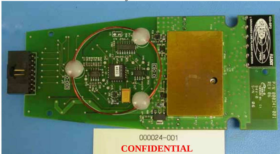
Front Side of Circuit Assembly 000024-001
