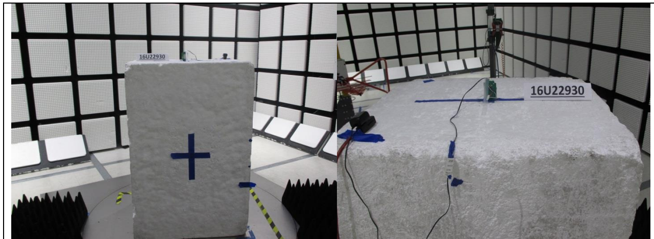
RADIATED FRONT PHOTO (ABOVE 1 GHz)
