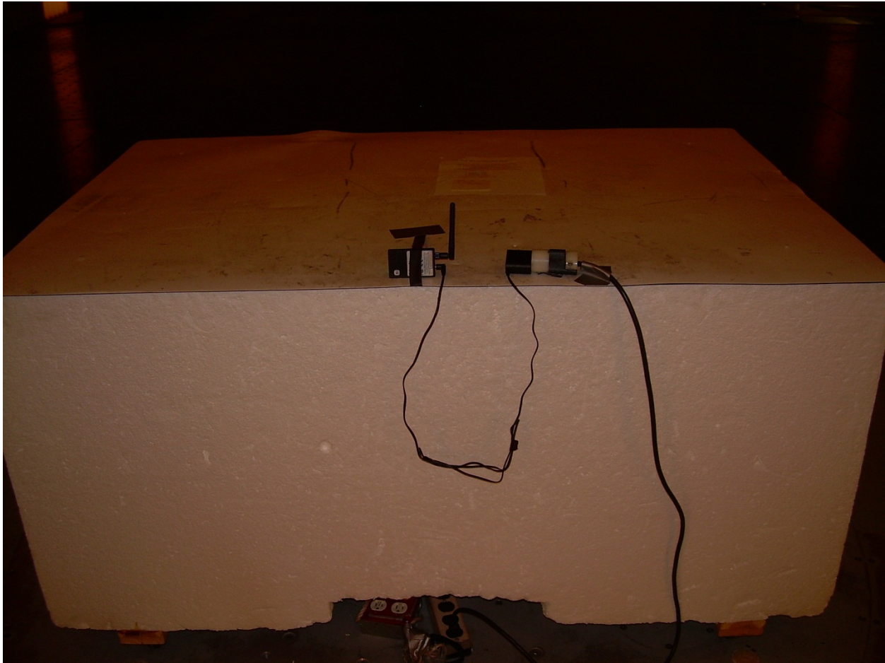
Photograph 4 – Back View Radiated Disturbance – On Edge Configuration
