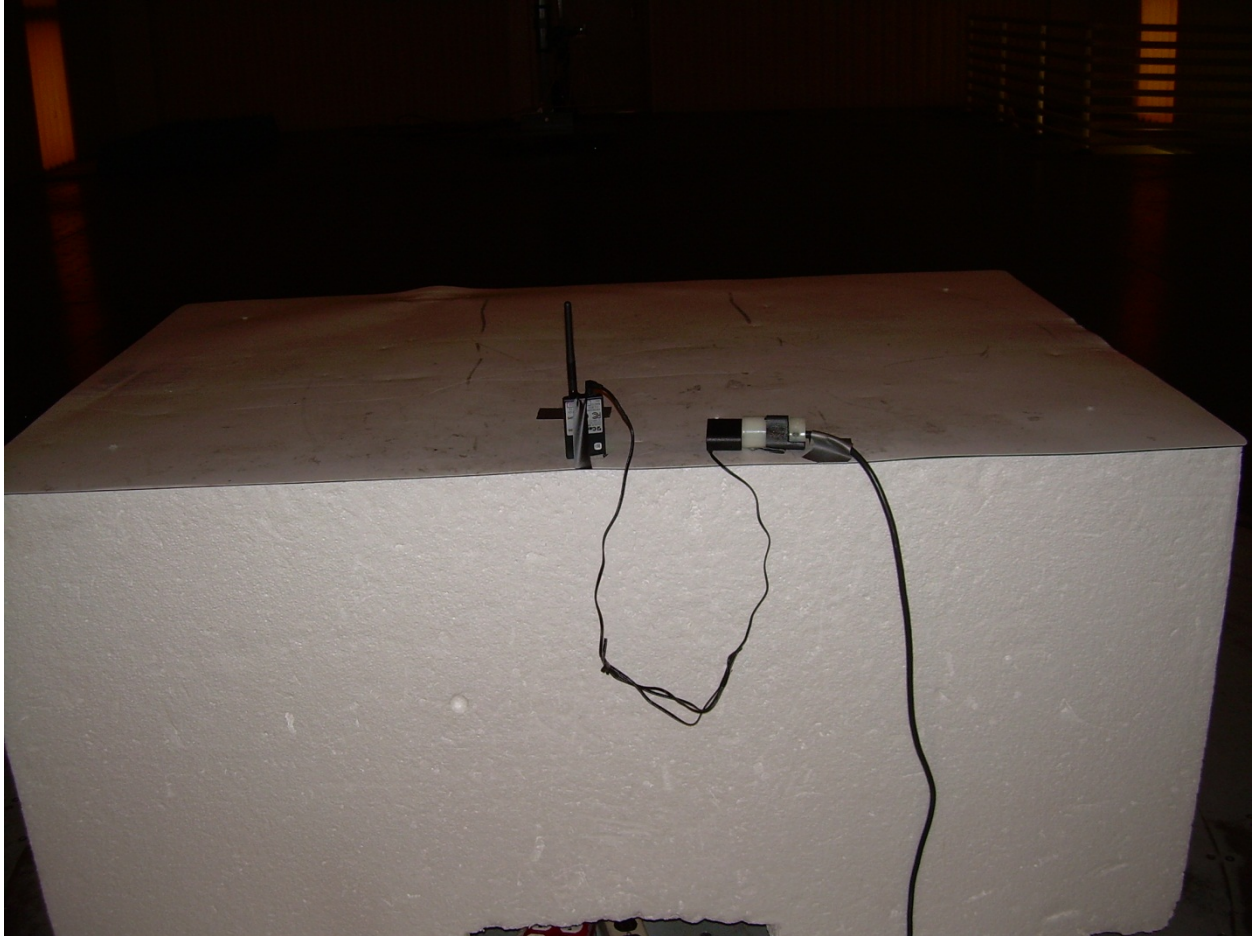
Photograph 2 – Back View Radiated Disturbance Worst Case Configuration – Vertical
