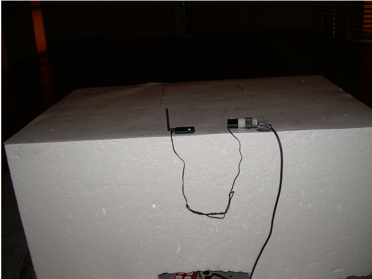
Photograph 3 – Back View Radiated Disturbance – Horizontal Configuration
