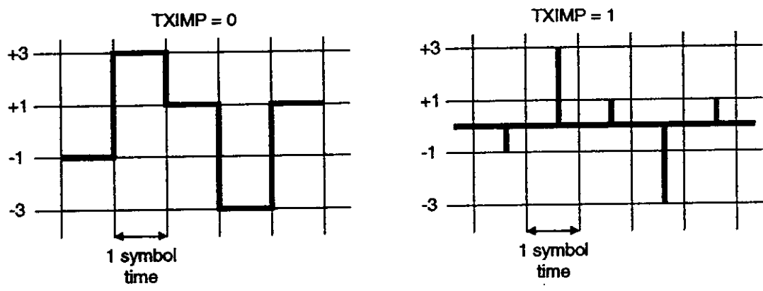
Figure 16: Input Signal to RRC Filter in Tx Mode for TXIMP = 0 and 1
