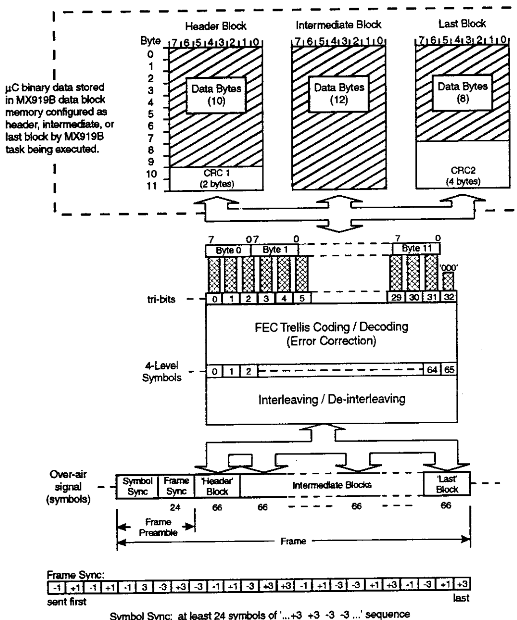
Figure 7: Over-Air Signal Format
