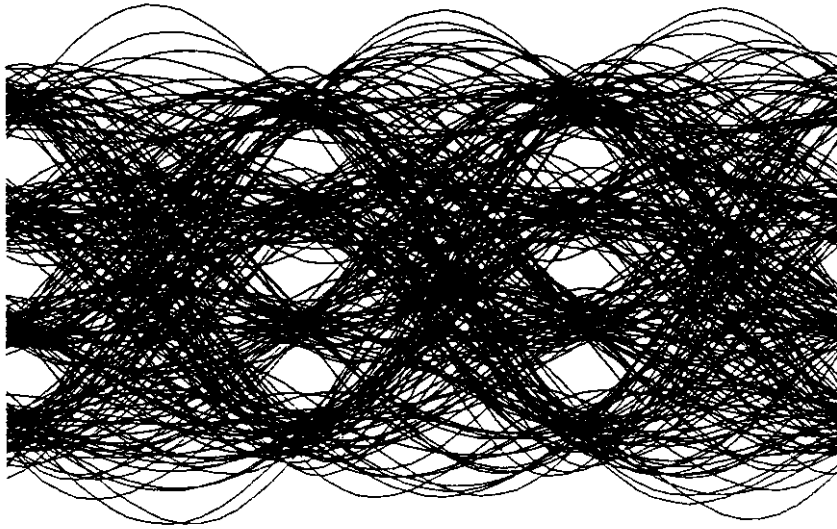
Figure 18: Tx Signal Eye TXIMP = 1
