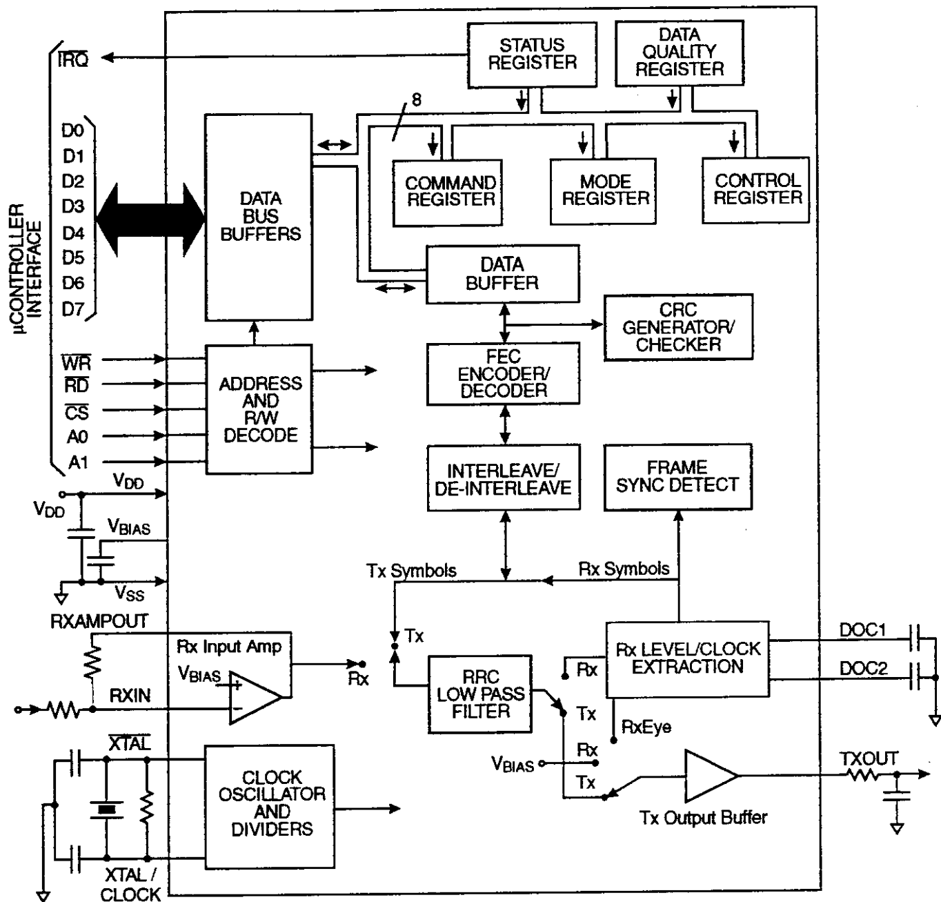
Figure 1: Block Diagram
