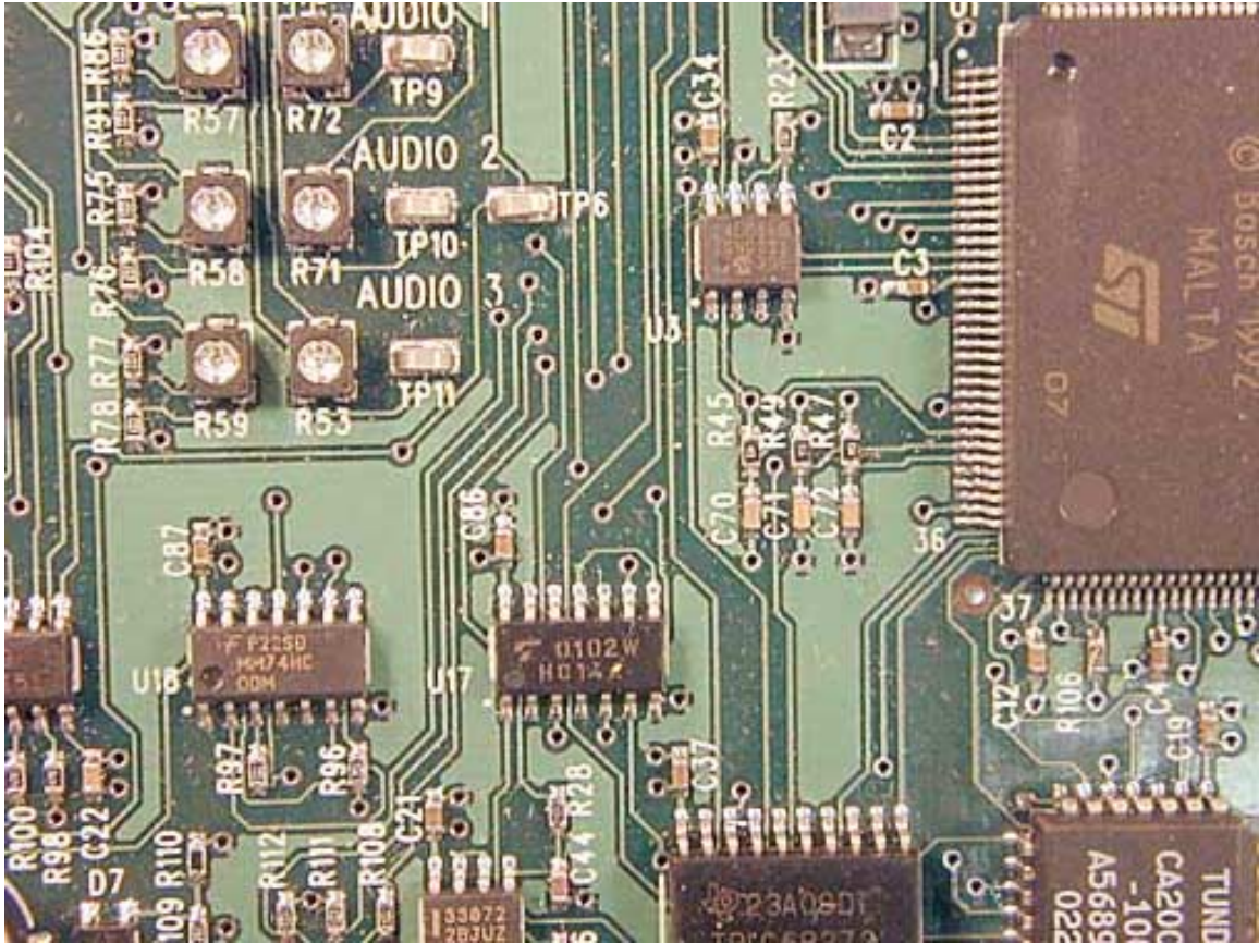
System Board PCB Top Close-Up 5
