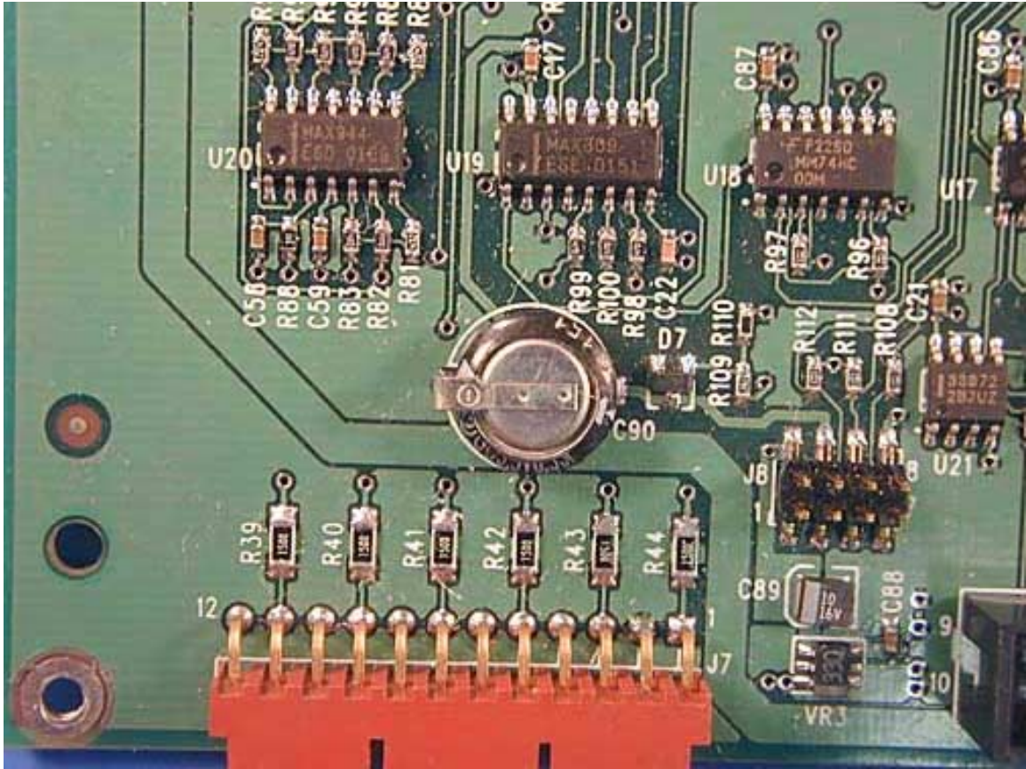
System Board PCB Top Close-Up 3
