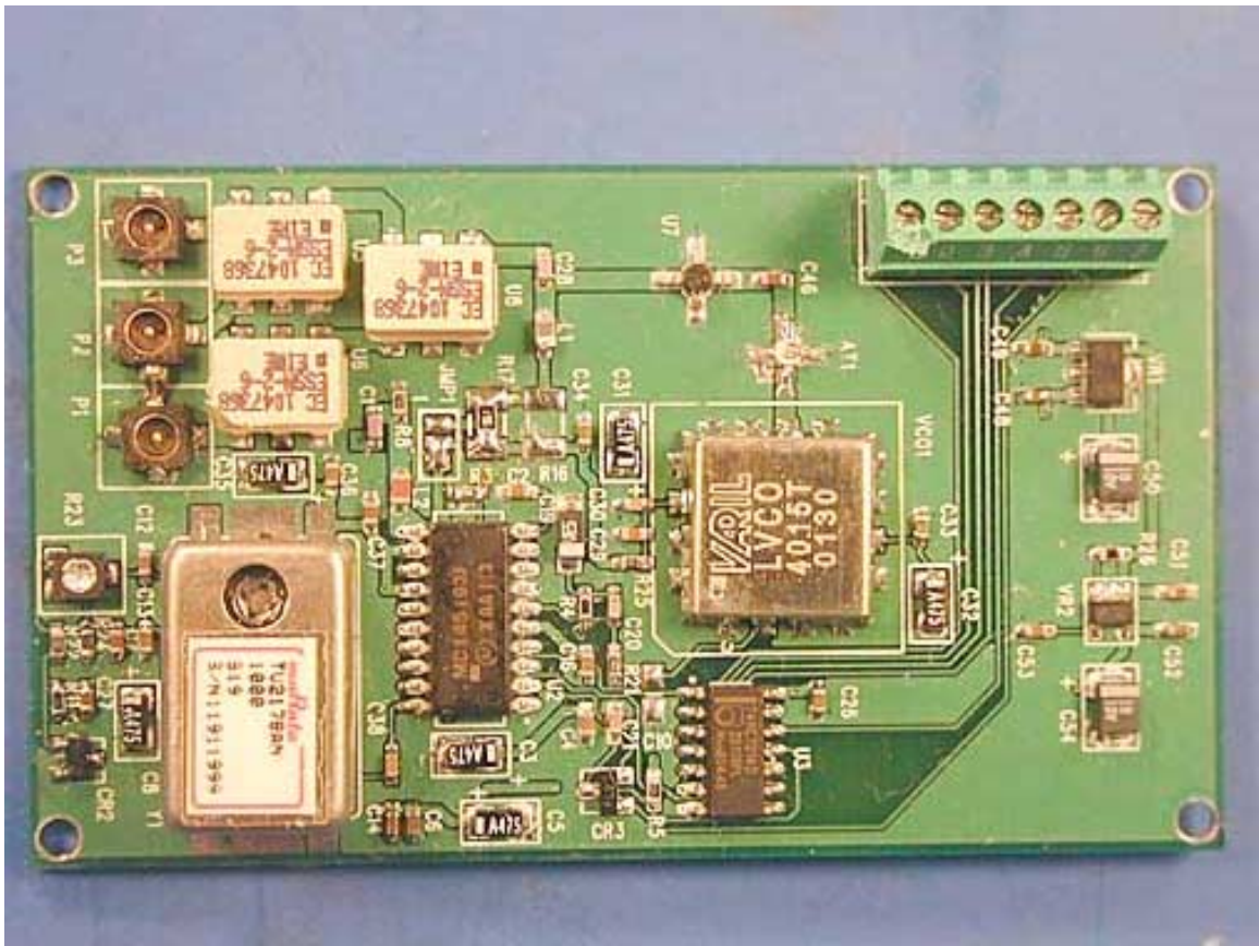
RX Injection PCB - Top
