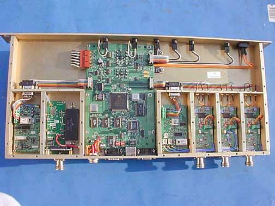
EUT Cover Removed
