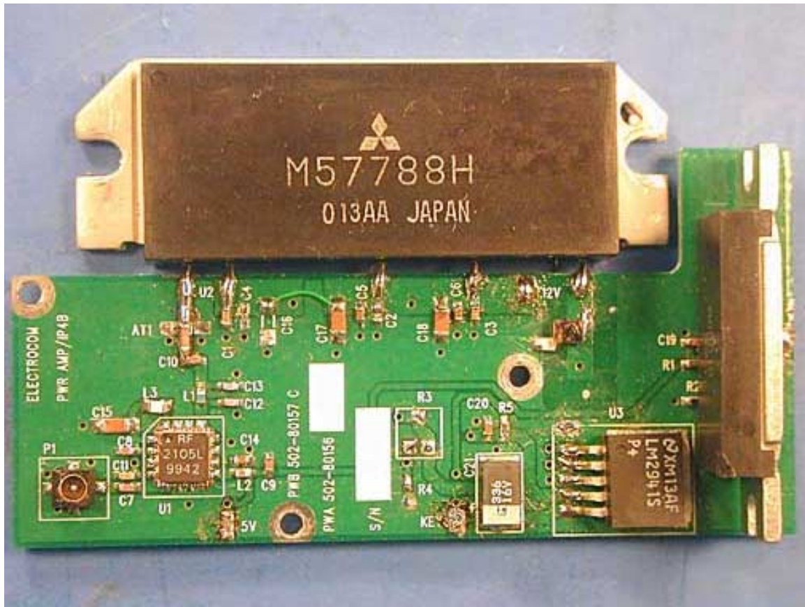
Power Amp PCB – 469 MHz Top
