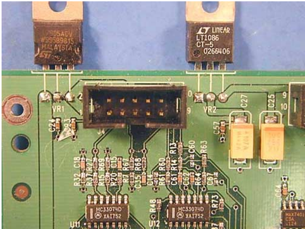
System Board PCB Top Close-Up 1
