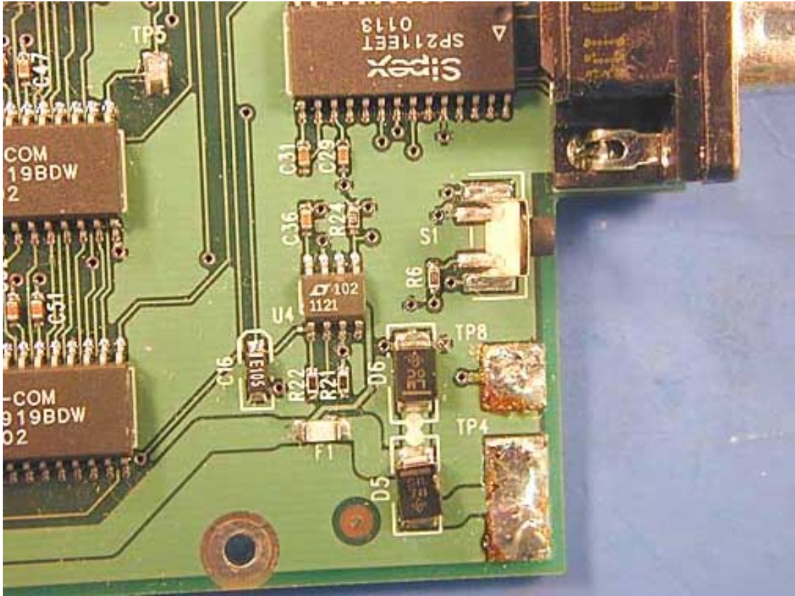
System Board PCB Top Close-Up 11
