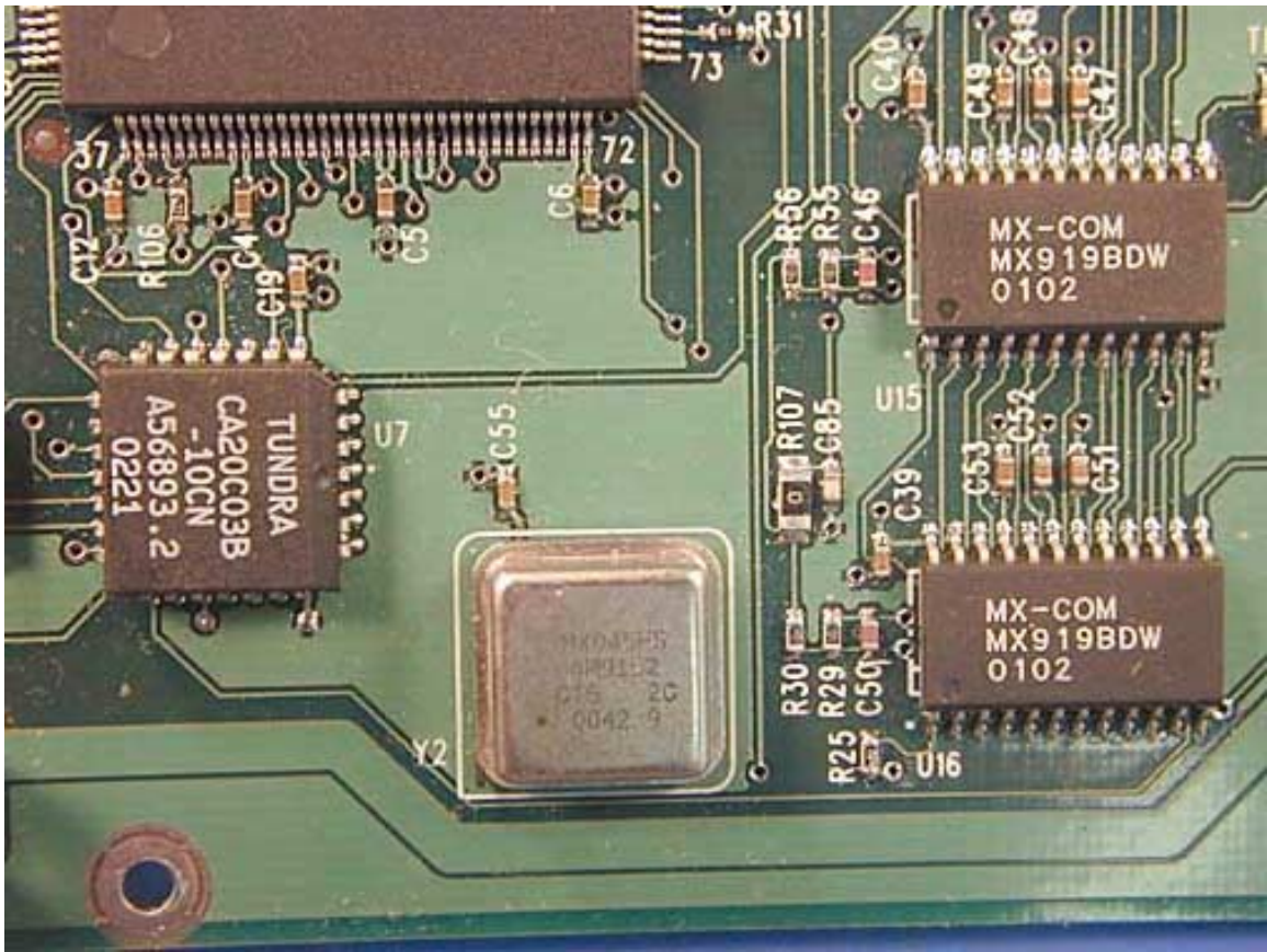
System Board PCB Top Close-Up 10
