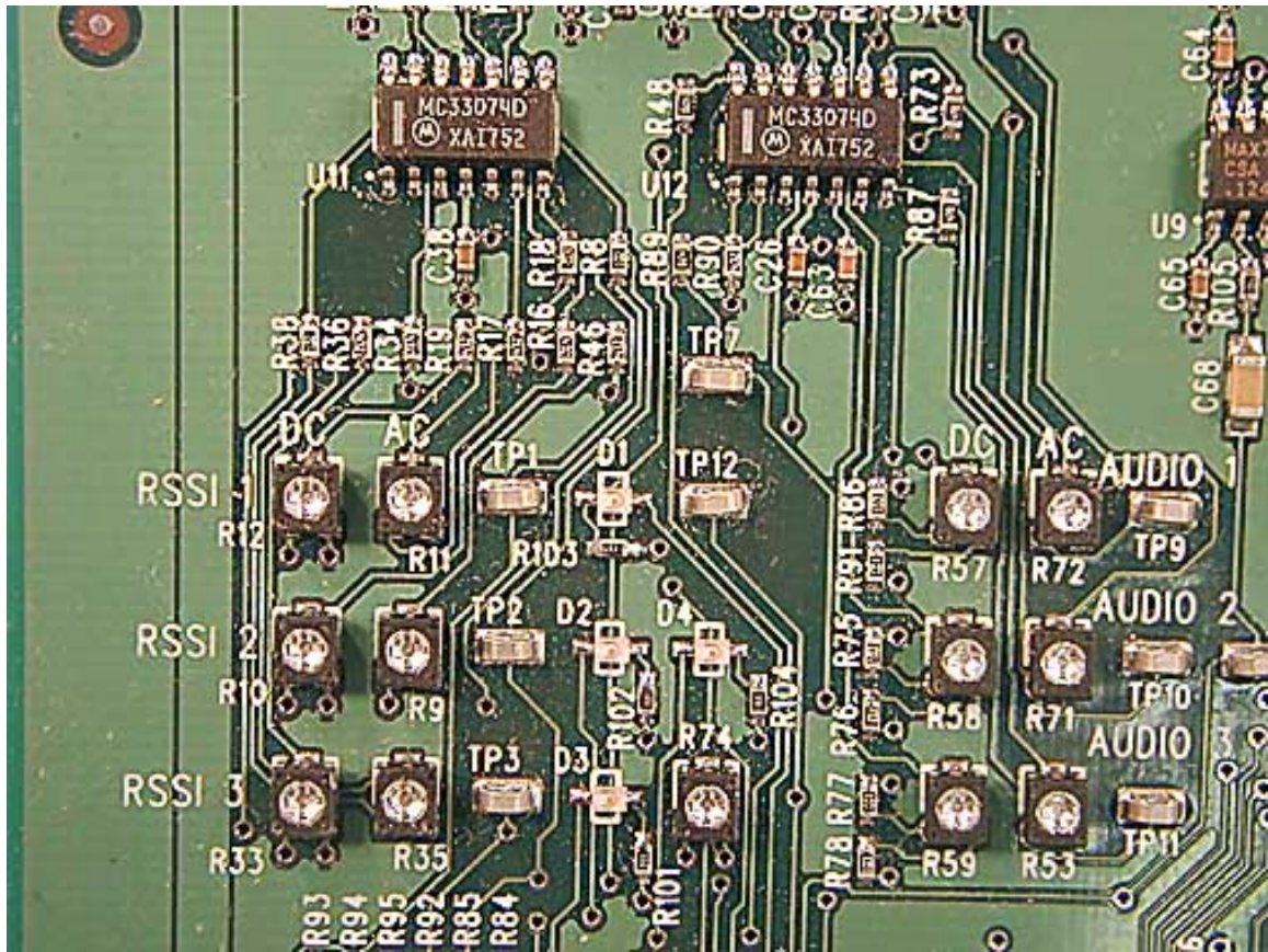
System Board PCB Top Close-Up 2
