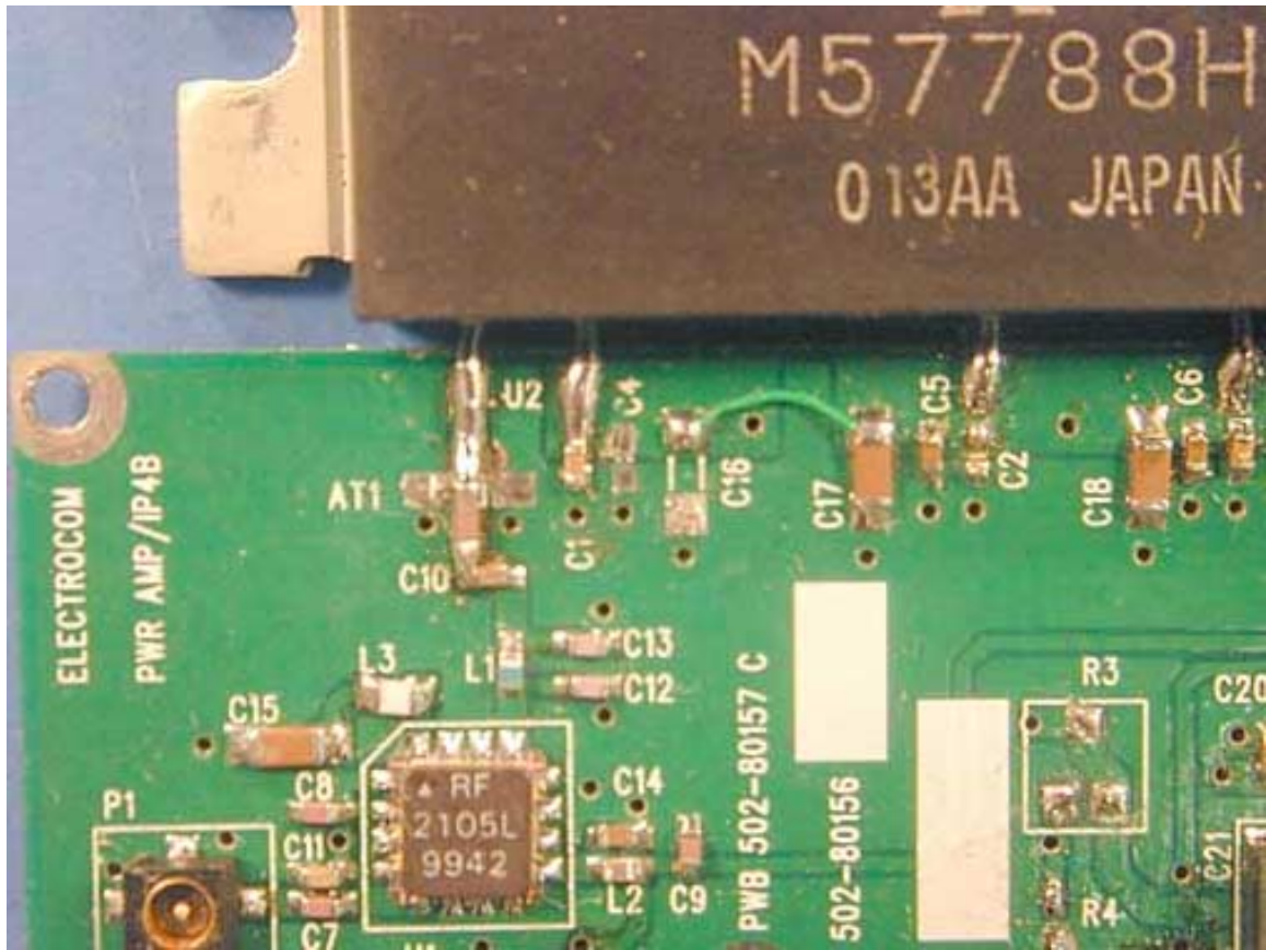
Power Amp – 469 MHz Component
