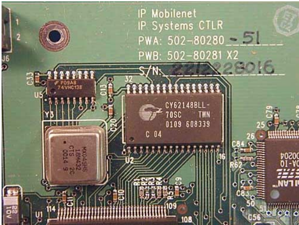
System Board PCB Top Close-Up 8
