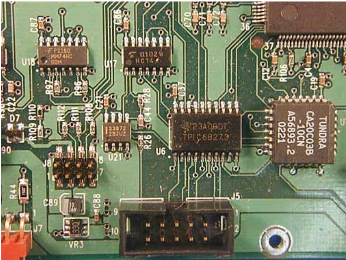
System Board PCB Top Close-Up 4
