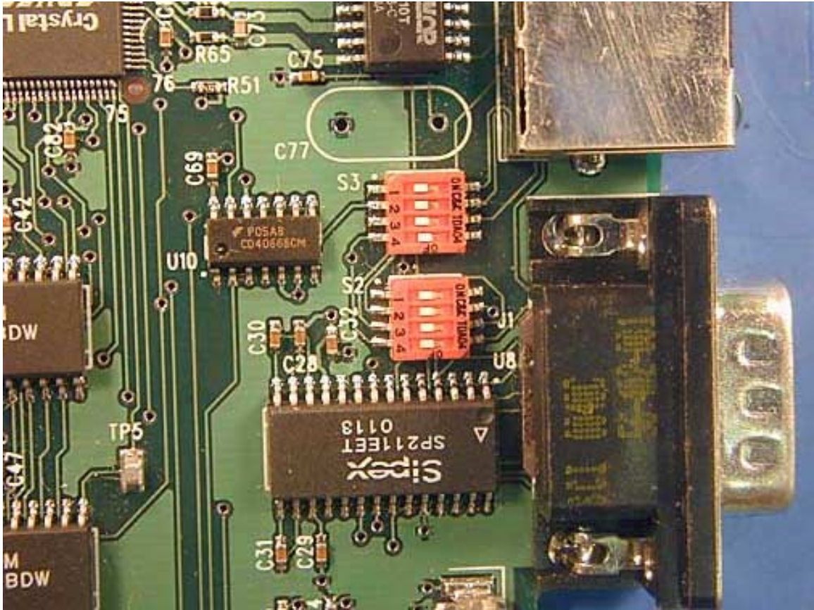
System Board PCB Top Close-Up 12
