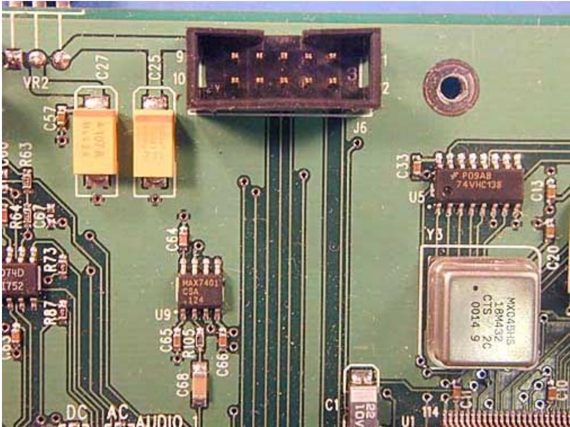
System Board PCB Top Close-Up 7
