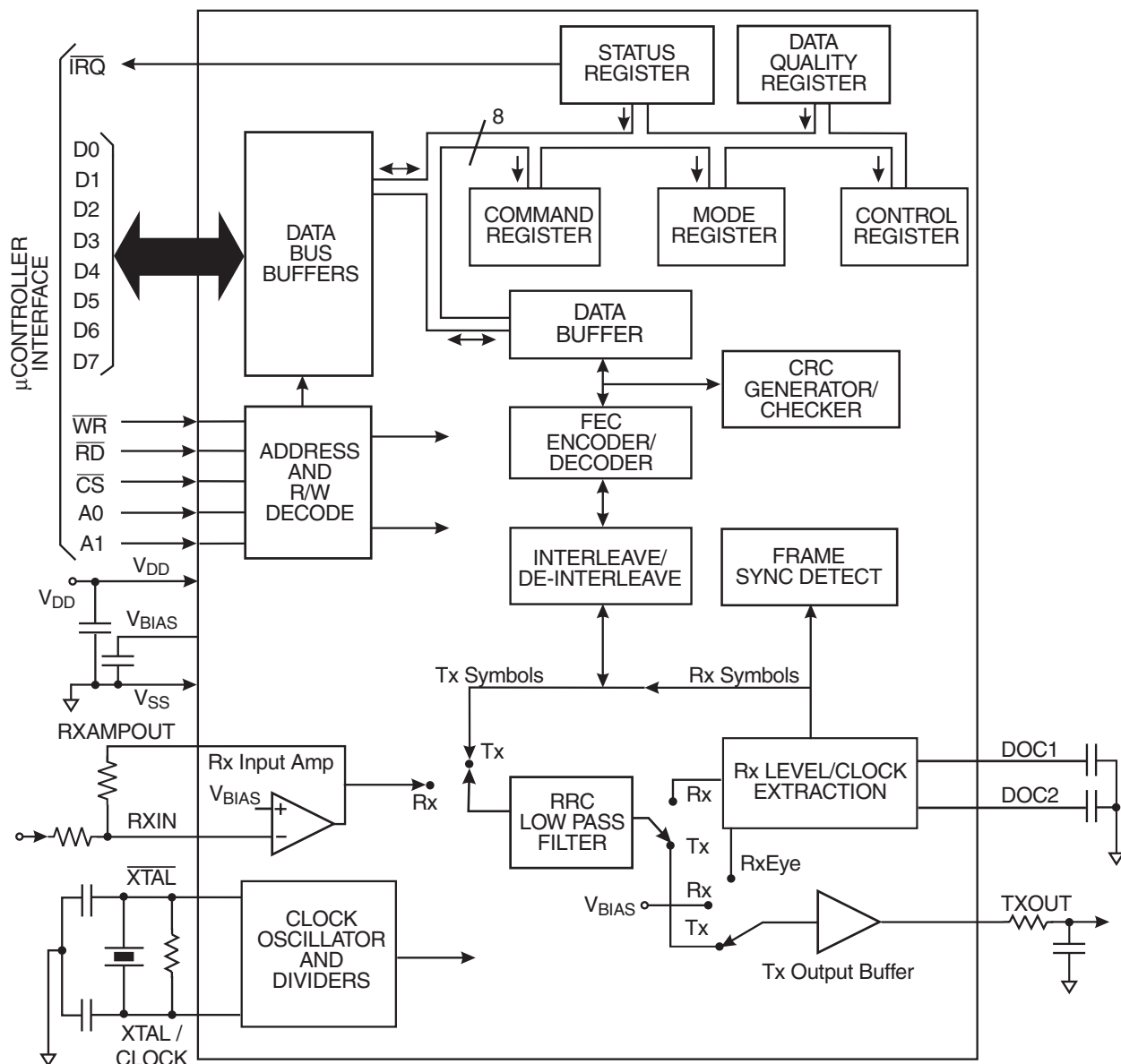
Figure 1: Block Diagram
