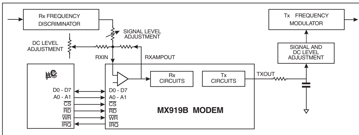
Figure 26: Typical Connections between Radio and MX919B
