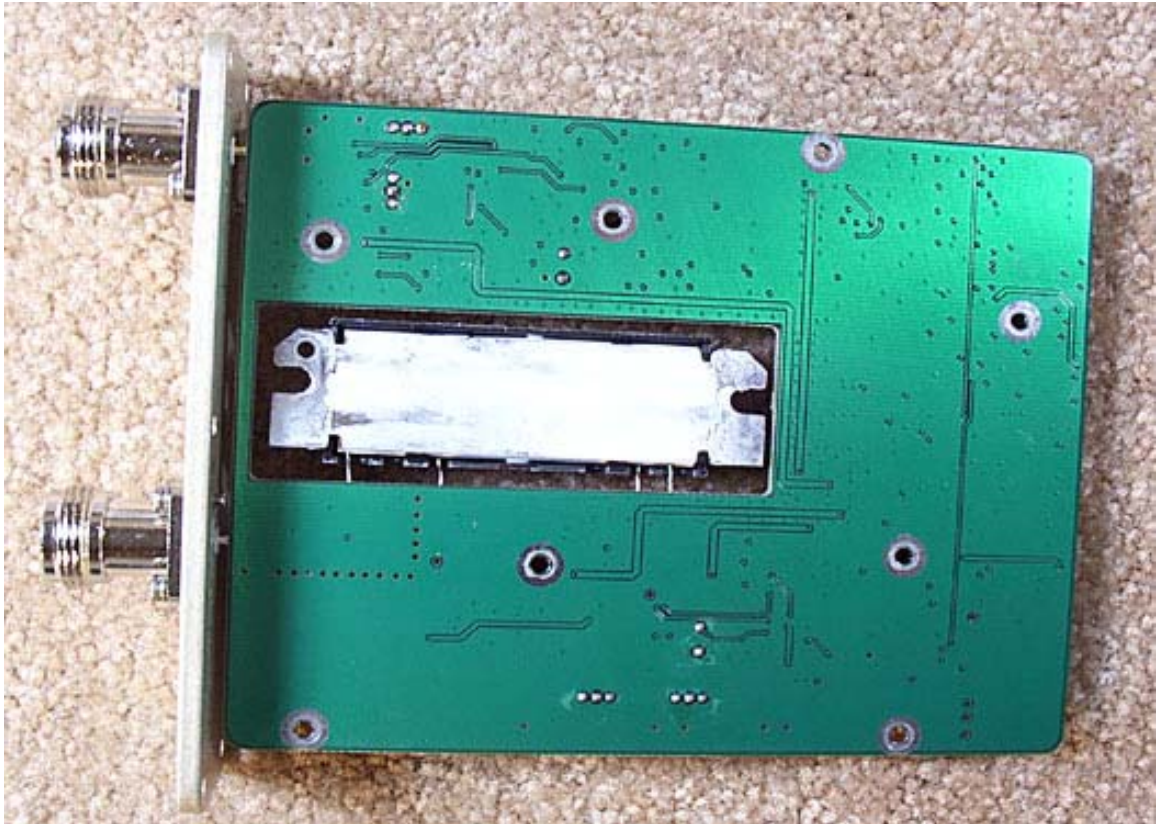
Back PCB Back Side
