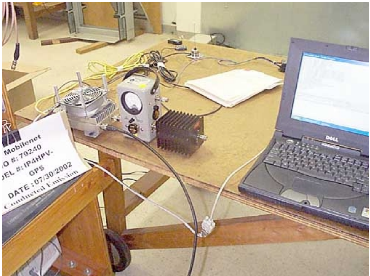
PHOTOGRAPH SHOWING CONDUCTED EMISSIONS FCC 15.111
