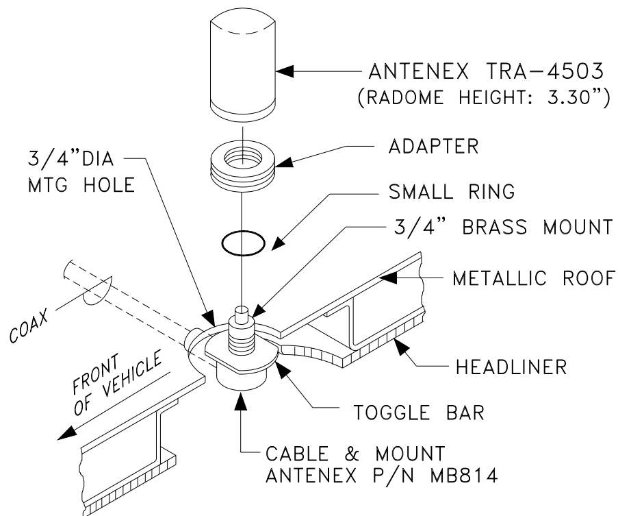
DETAIL A
