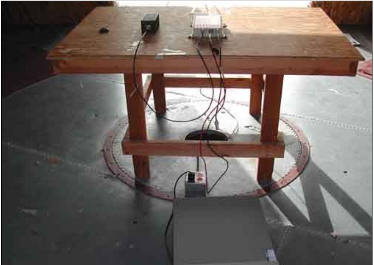
PHOTOGRAPH SHOWING RADIATED EMISSIONS
