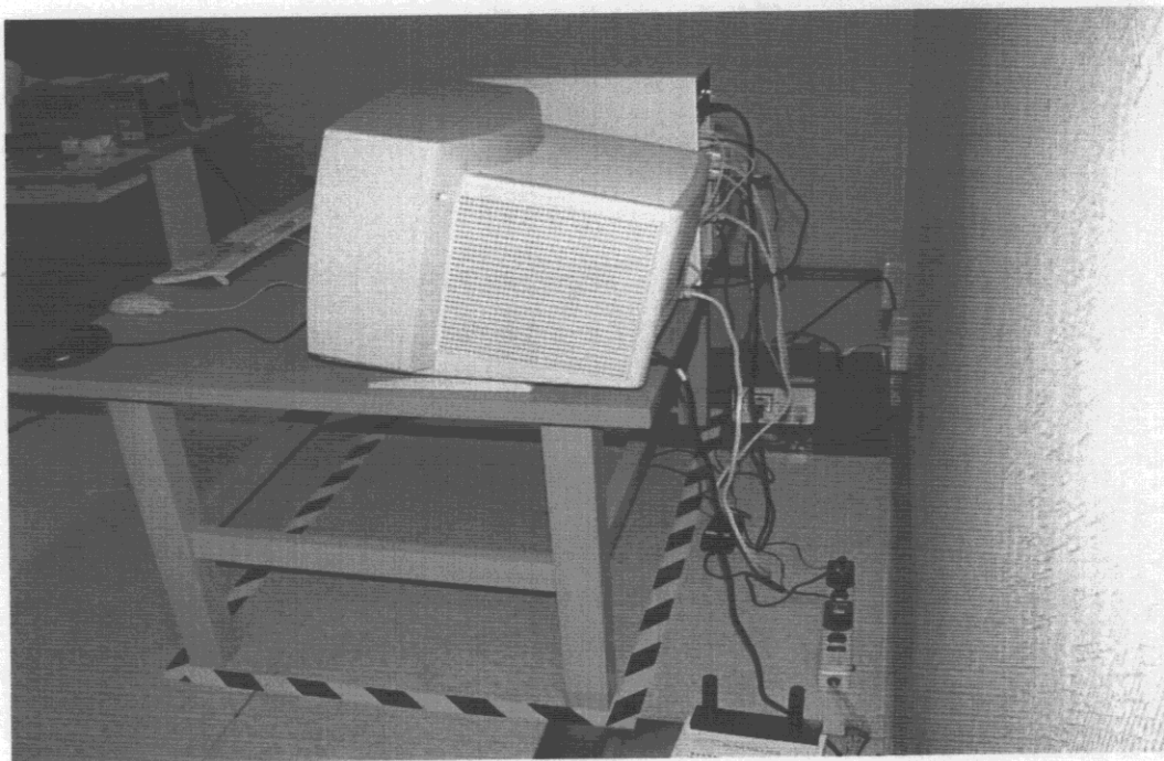
Back View of Conducted Test ( Maximum Testing Configuration)
