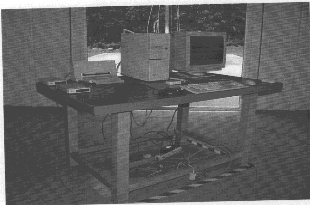
Front View of Radiated Test ( Maximum Testing Configuration)
