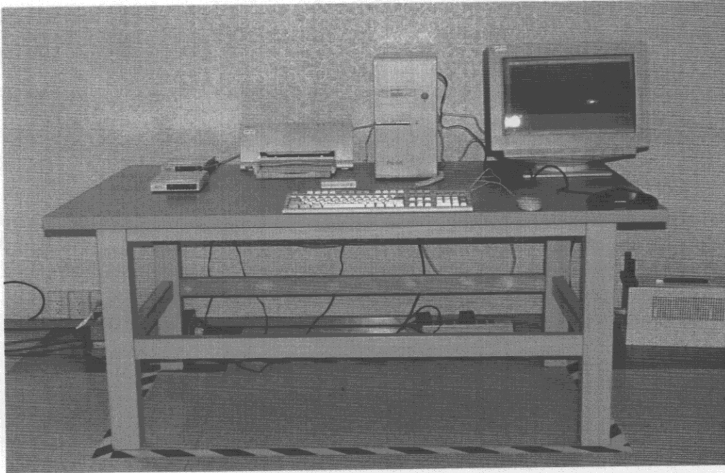
Front View of Conducted Test ( Maximum Testing Configuration)
