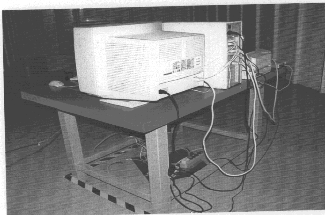
Back View of Radiated Test ( Maximum Testing Configuration)
