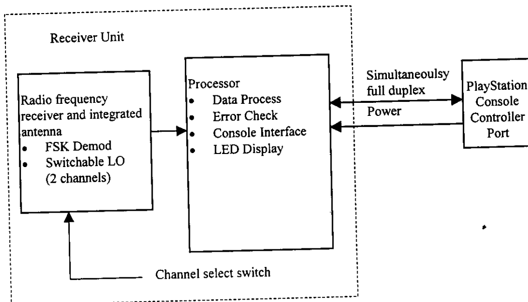
Figure 2. Receiver Unit Block Diagram
