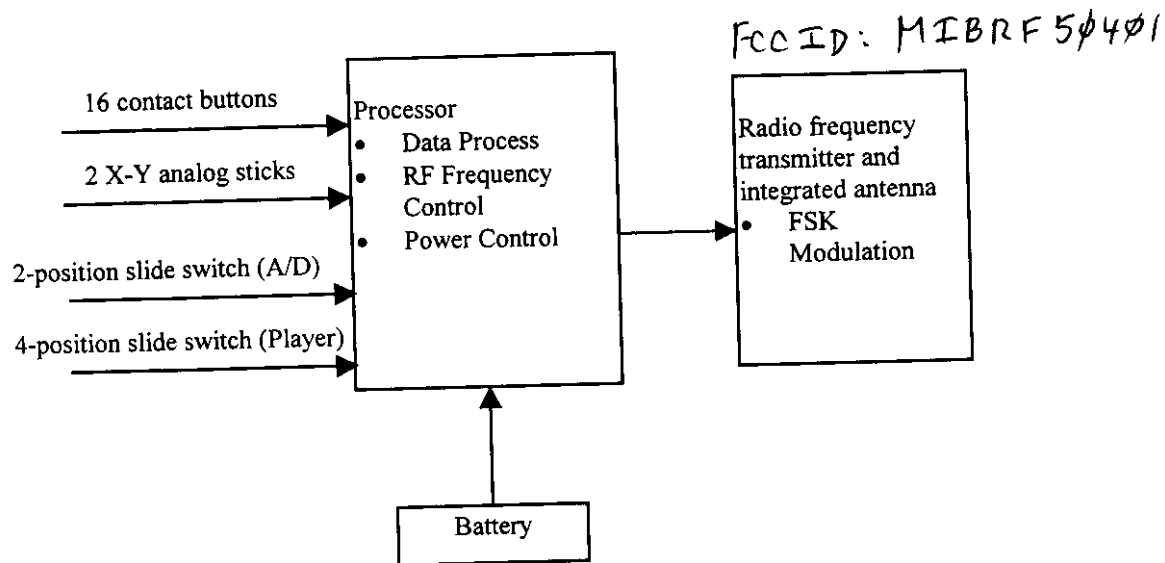
Figure 1. Transmitter Unit Block Diagram
