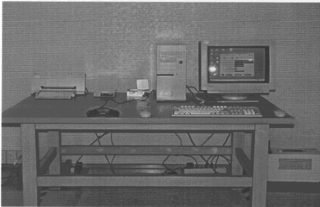
Front View of Fundamental Radiated Test ( Maximum Testing Configuration)
