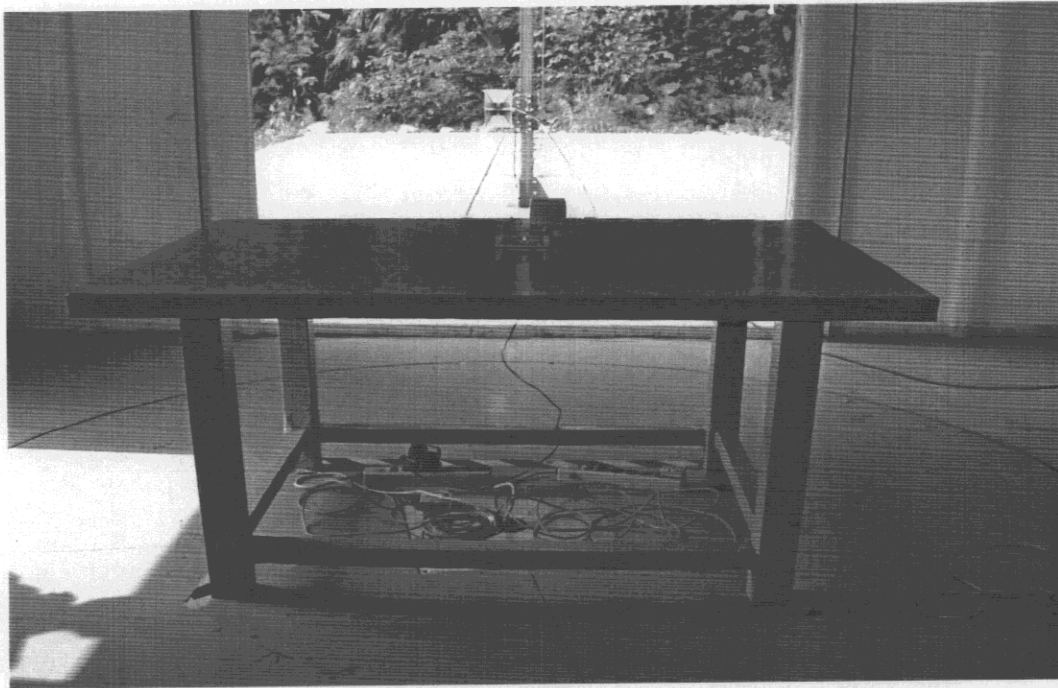
Back View of Spurious Radiated Test ( Maximum Testing Configuration)
