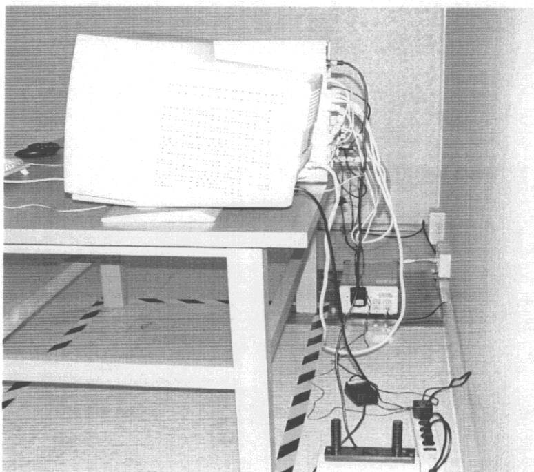
Front View of Fundamental Radiated Test ( Maximum Testing Configuration)
