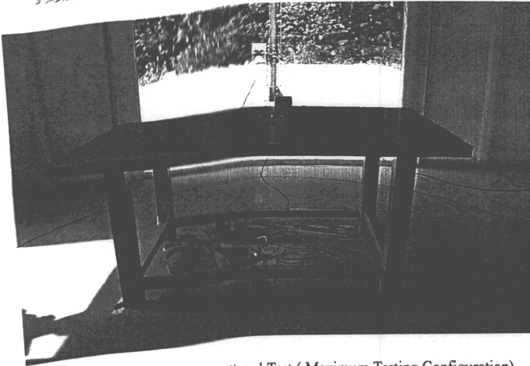
Back View of Spurious Radiated Test ( Maximum Testing Configuration)
