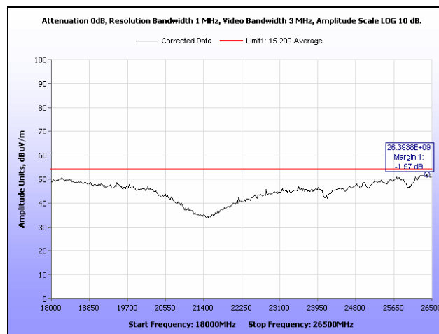
Plot 18. Radiated Spurious Emissions, Mid Channel, 18 GHz – 26.5 GHz, Peak Under Average
