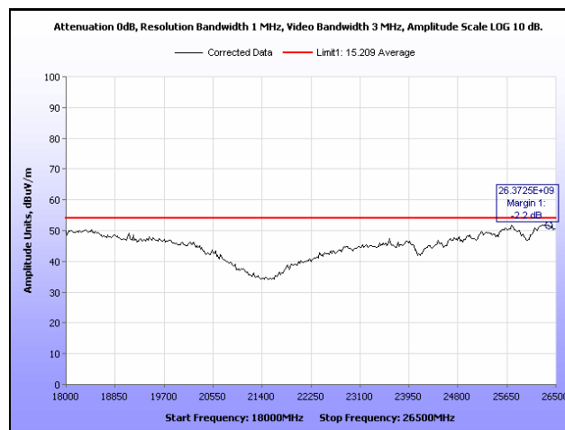
Plot 12. Radiated Spurious Emissions, Low Channel, 18 GHz – 26.5 GHz, Peak Under Average
