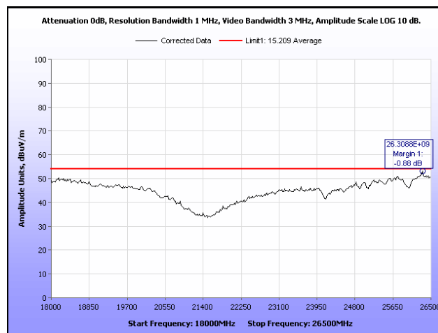
Plot 24. Radiated Spurious Emissions, High Channel, 18 GHz – 26.5 GHz, Peak Under Average
