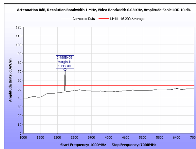
Plot 20. Radiated Spurious Emissions, High Channel, 1 GHz – 7 GHz, Average
