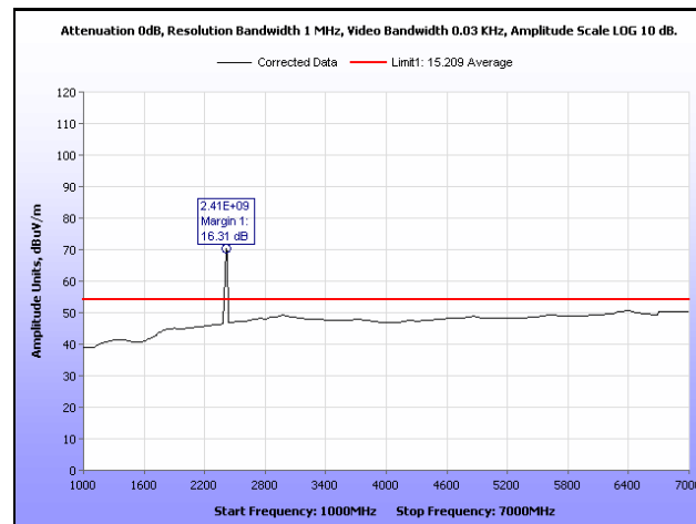
Plot 8. Radiated Spurious Emissions, Low Channel, 1 GHz – 7 GHz, Average
