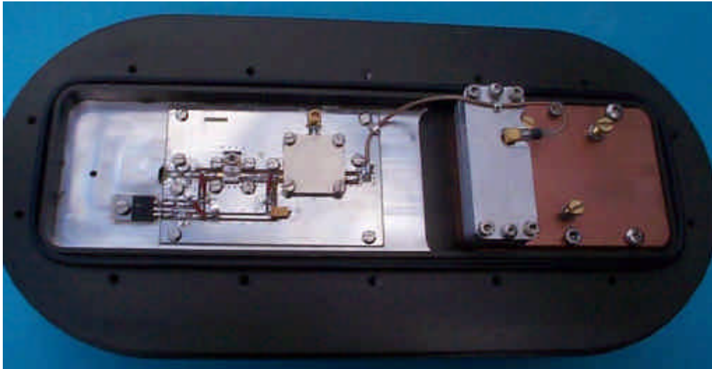
Figure A2. Plate showing layout of components within AD510 base. The interdigital filter and LNA are to the right, the circulator and TX amplifier and ancillary components are mounted on the PCB centre left (see figure A3 for detail).
