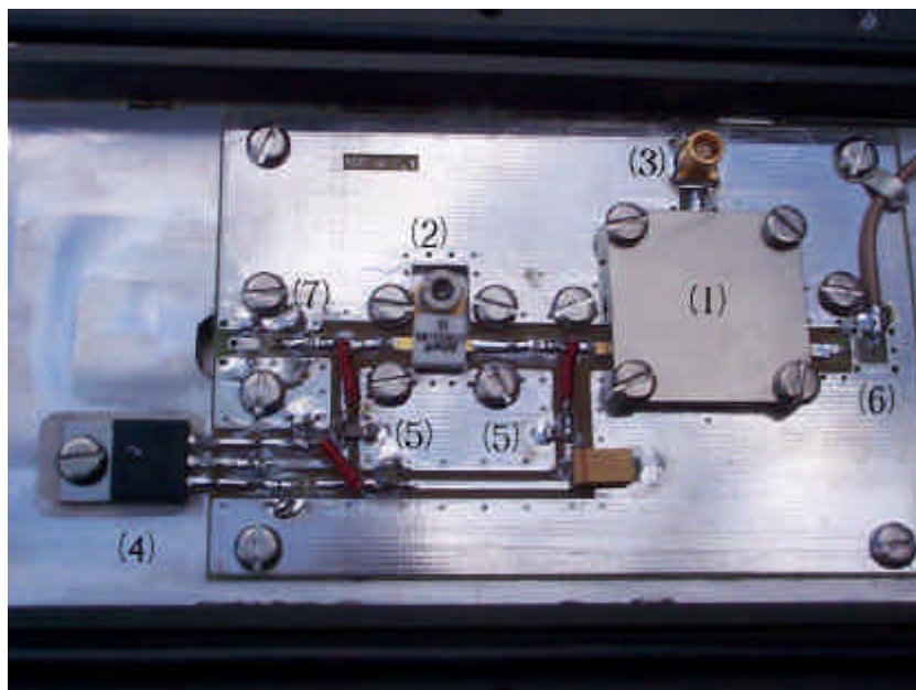
Figure A3. Plate showing circuit board with circulator (1) and transmit amplifier (2). DC power for the amplifier is fed from the MCX input/output connector (3), through the circulator to a LM317T voltage regulator (4). RF is blocked by LC components (5). The
