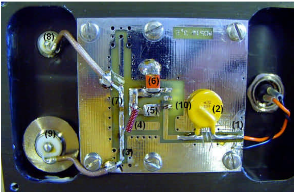
Figure A4. Plate showing circuit board carrying DC voltage regulator and ancillary components used in AD510-40. DC supply is via orange lead (1) and auto-reset fuse (2) to the voltage regulator pin input (10). The voltage regulator is a standard package (Texas Instruments PT5102A) and mounted on the reverse of the board. The stabilised supply is connected to 50 Ohm strip-line (3) with a coil inductor (4). (5), (6) are and (7) are capacitors, the latter providing a DC block to the Iridium handset connected via TNC (8). (9) is an N-type connector for the 40m antenna down-lead.
