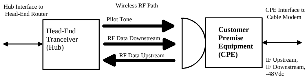
Figure 3.0-1 CPE Functional Interface
