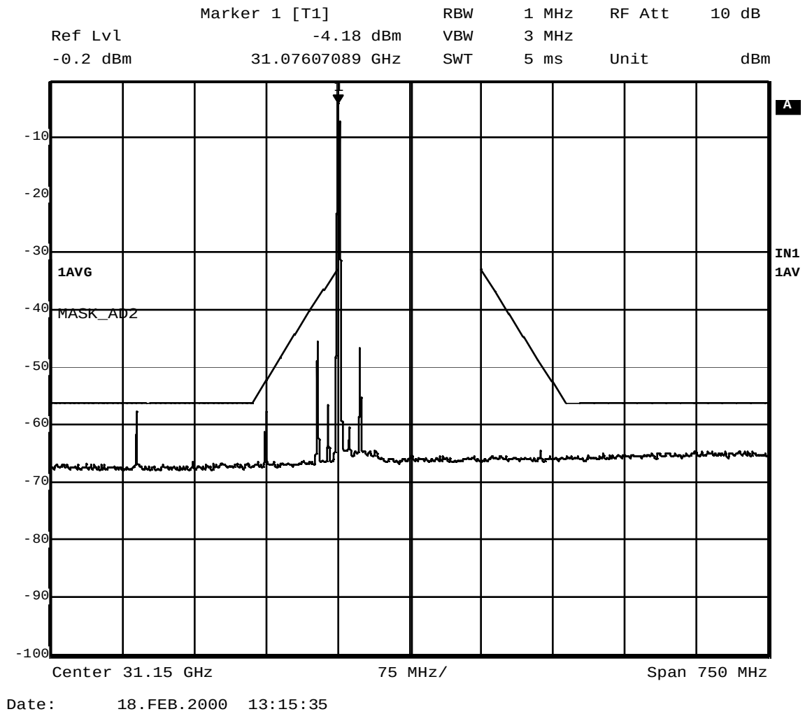
Figure A – 6 Emission Mask; 31.076 GHz; 16 QAM 0.384 MS/s
