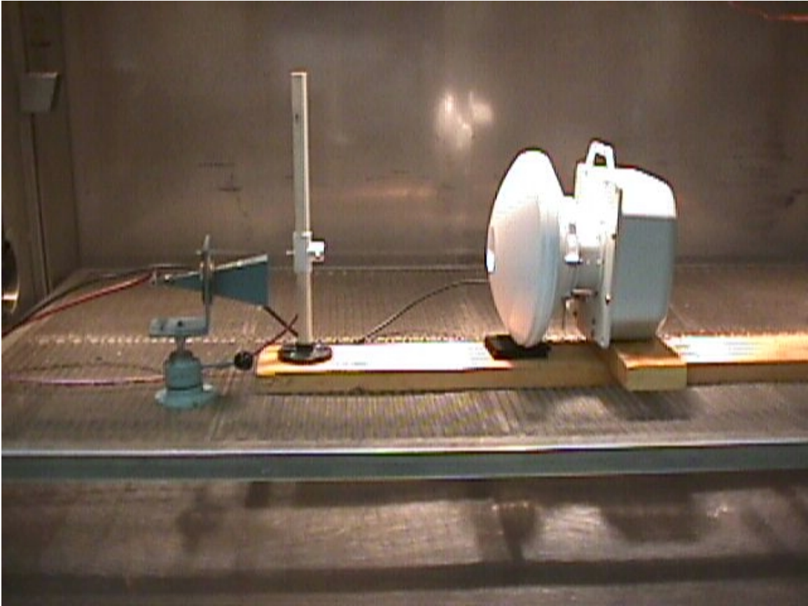
Figure C – 2 Test Setup, Frequency Stability Testing of the Motorola ODU
