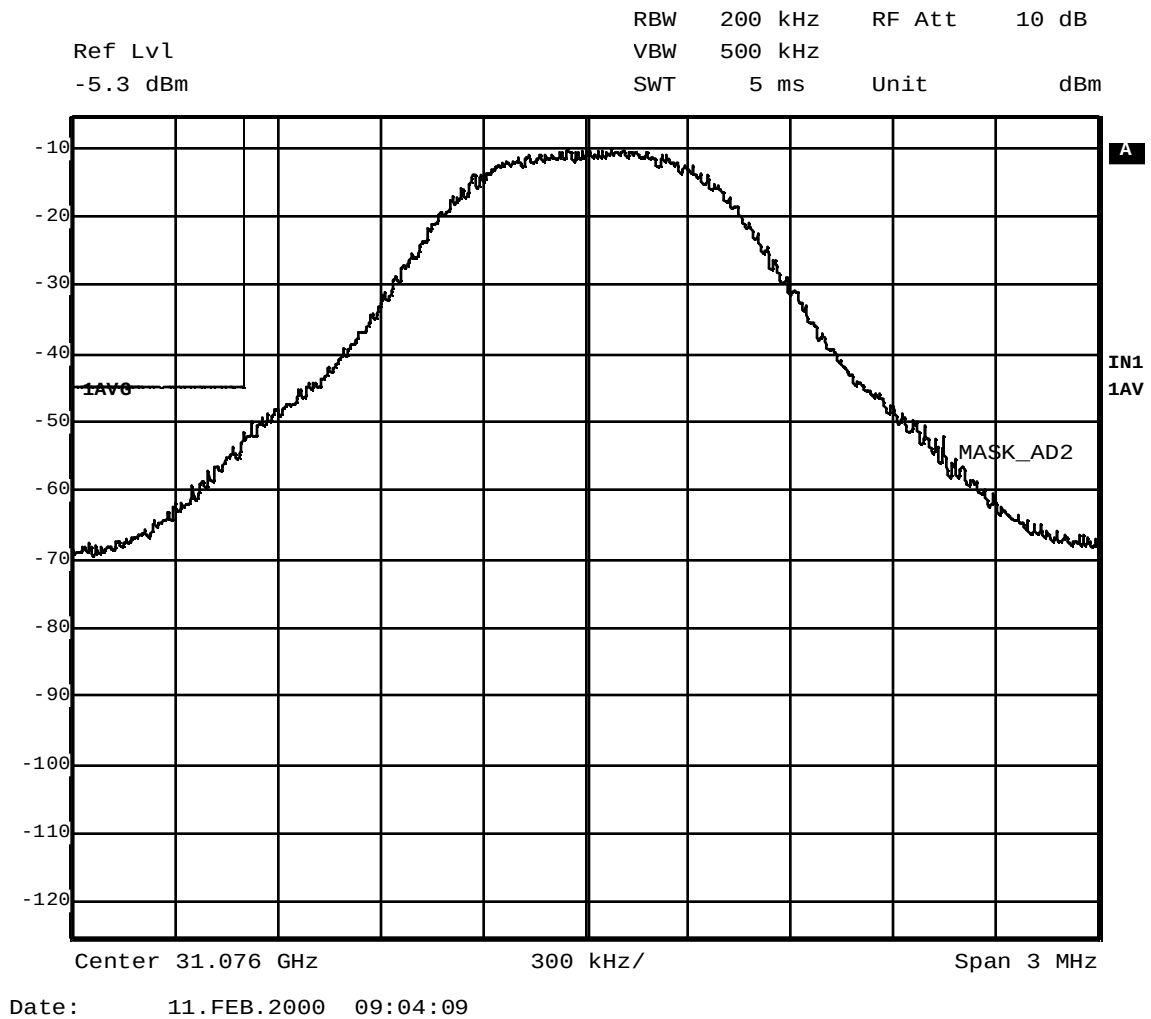
Figure A – 3 Emission Mask; 31.076 GHz; QPSK 0.64 MS/s
