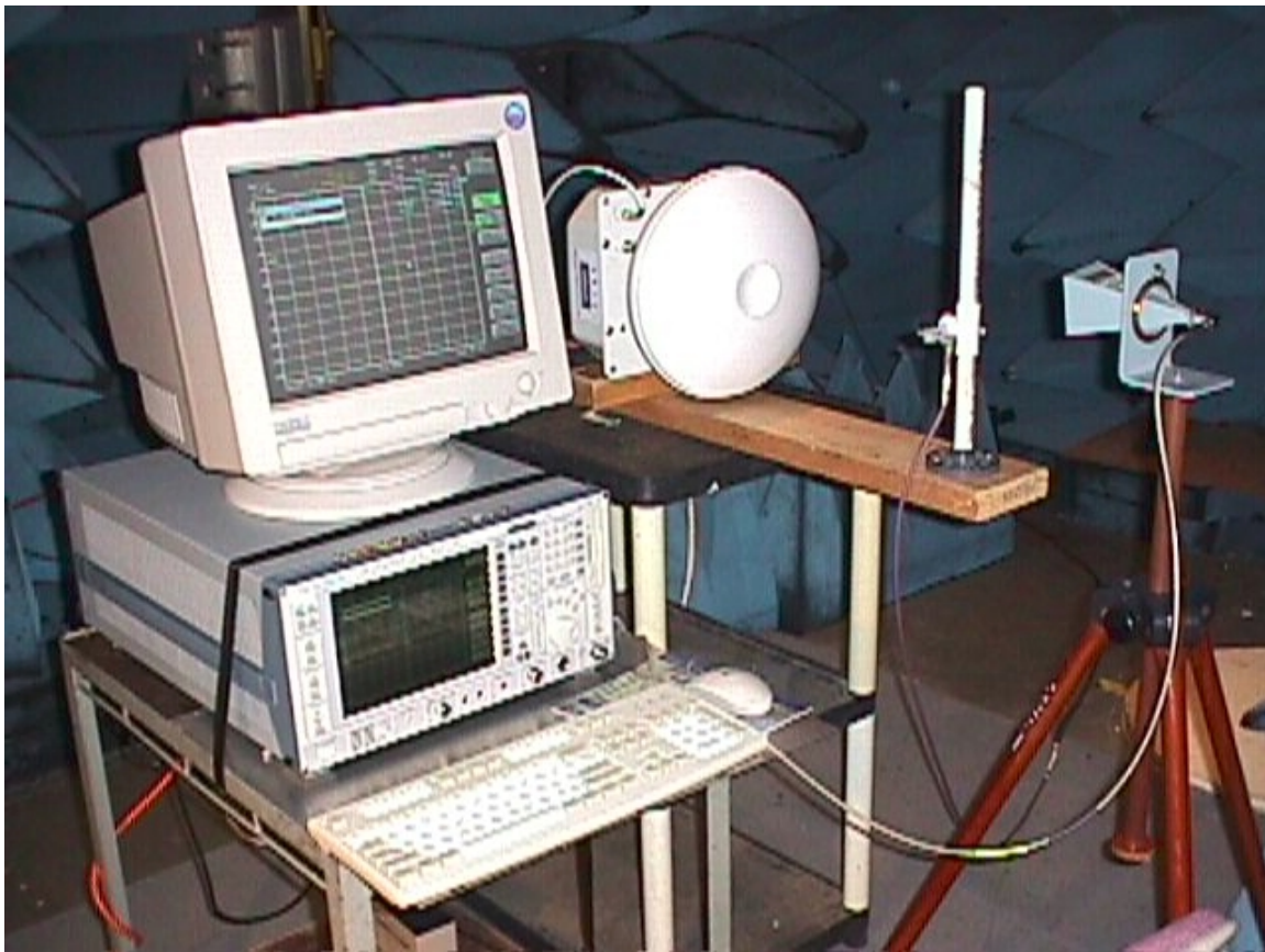
Figure A – 8 Test Setup; Emission Mask
