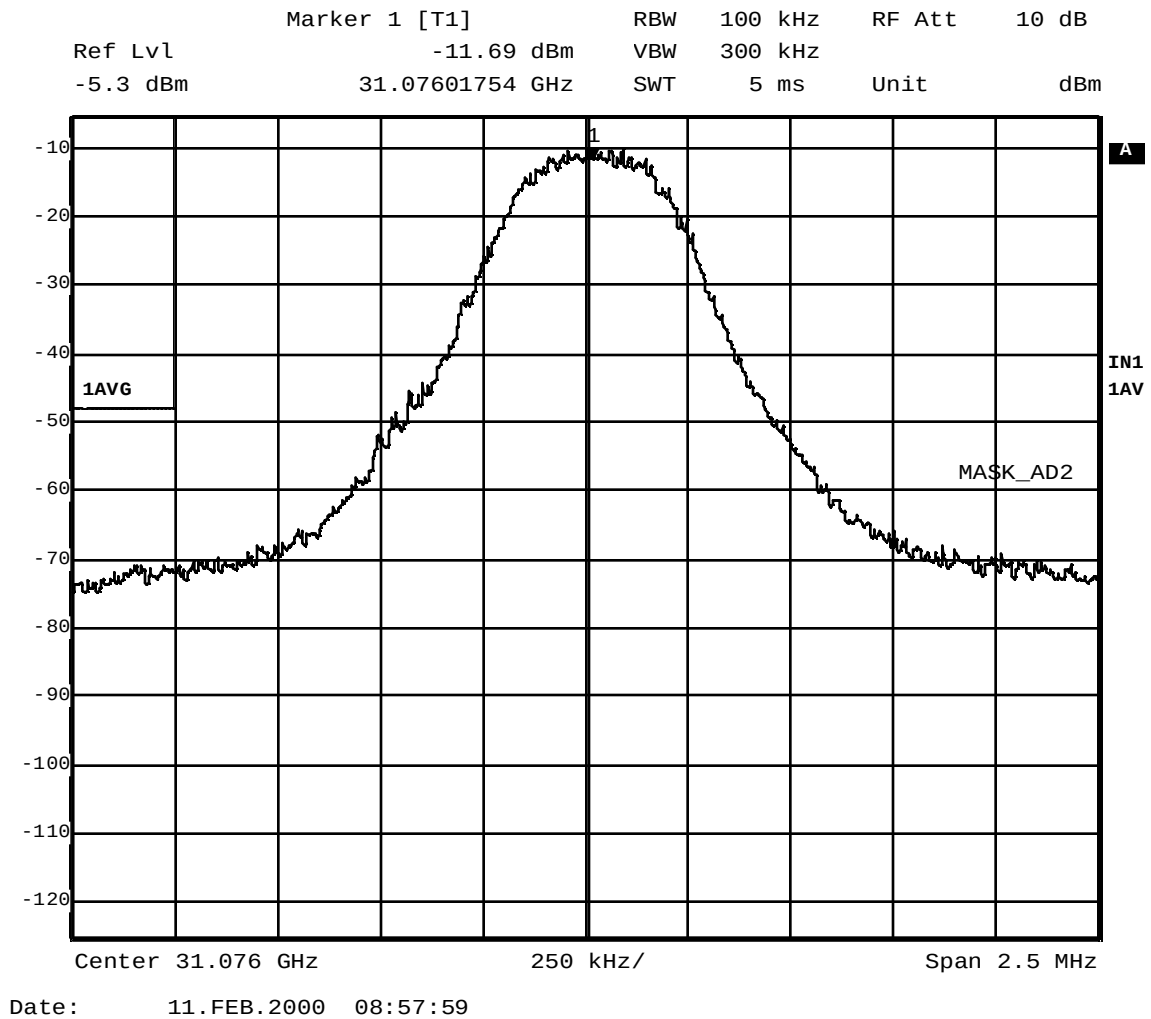
Figure A – 2 Emission Mask; 31.076 GHz; QPSK 0.32 MS/s
