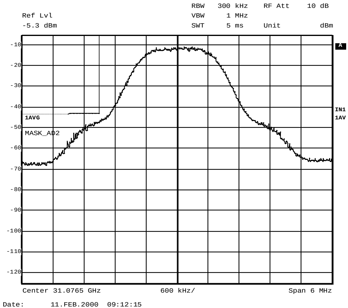
Figure A – 4 Emission Mask; 31.0765 GHz; QPSK 1.28 MS/s
