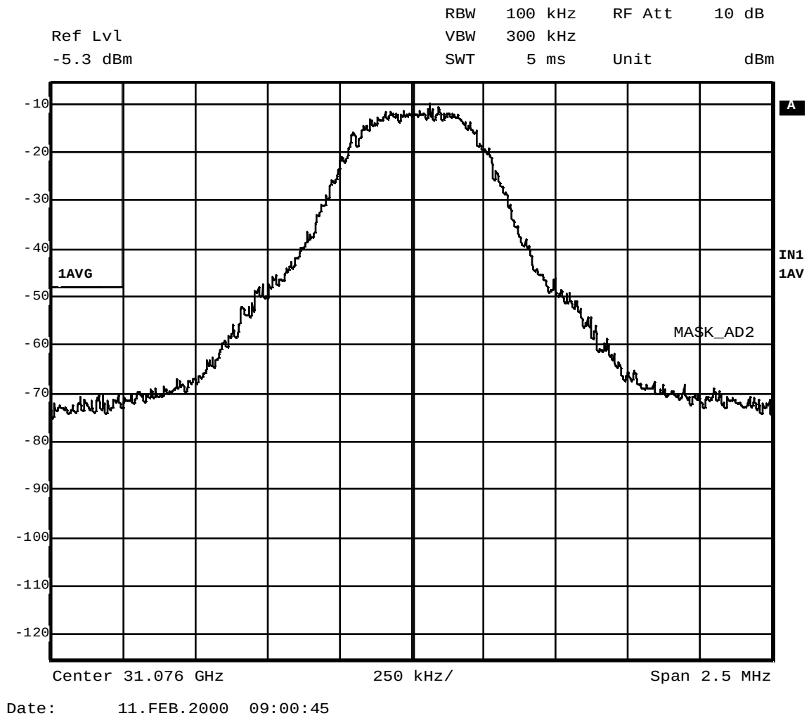
Figure A – 1 Emission Mask; 31.076 GHz; 16 QAM 0.384 MS/s
