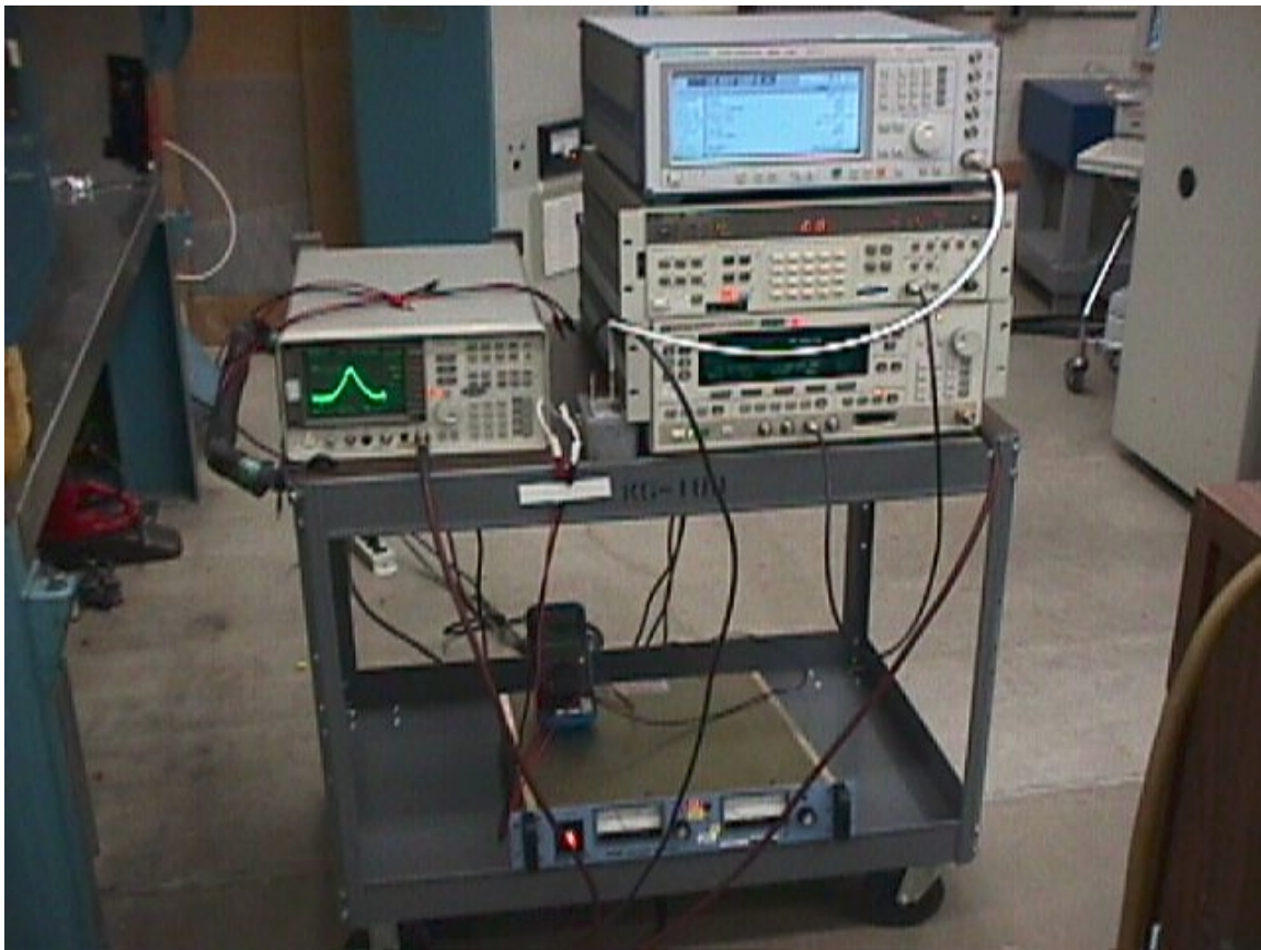
Figure C – 3 Test Setup, Frequency Stability Testing of the Motorola ODU
