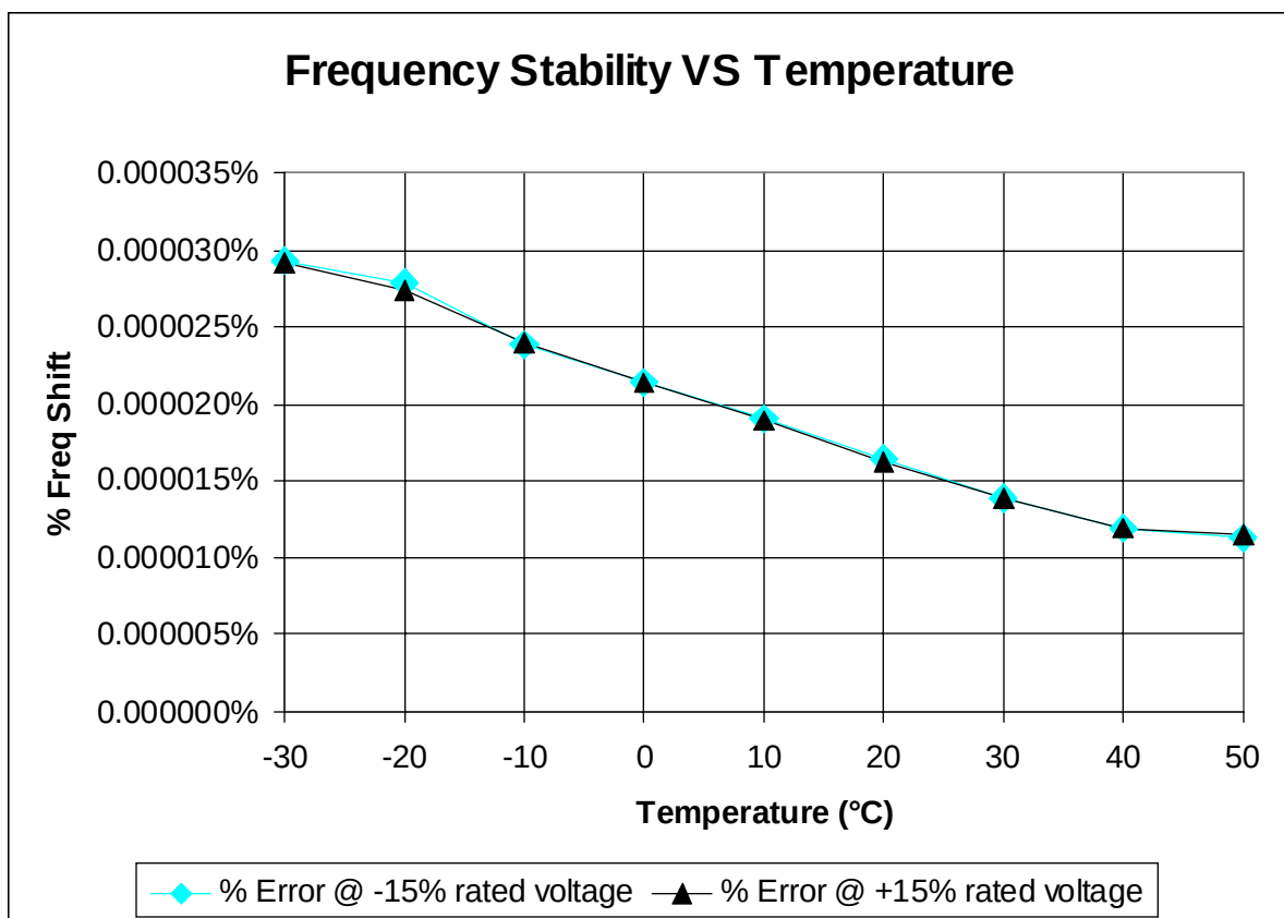
Figure C – 1 Frequency Stability Graph
