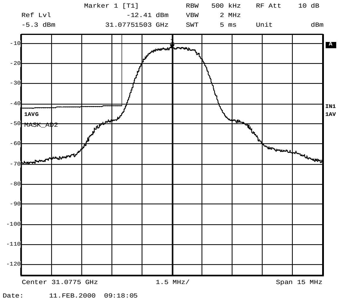
Figure A – 5 Emission Mask; 31.0775 GHz; QPSK 2.56 MS/s
