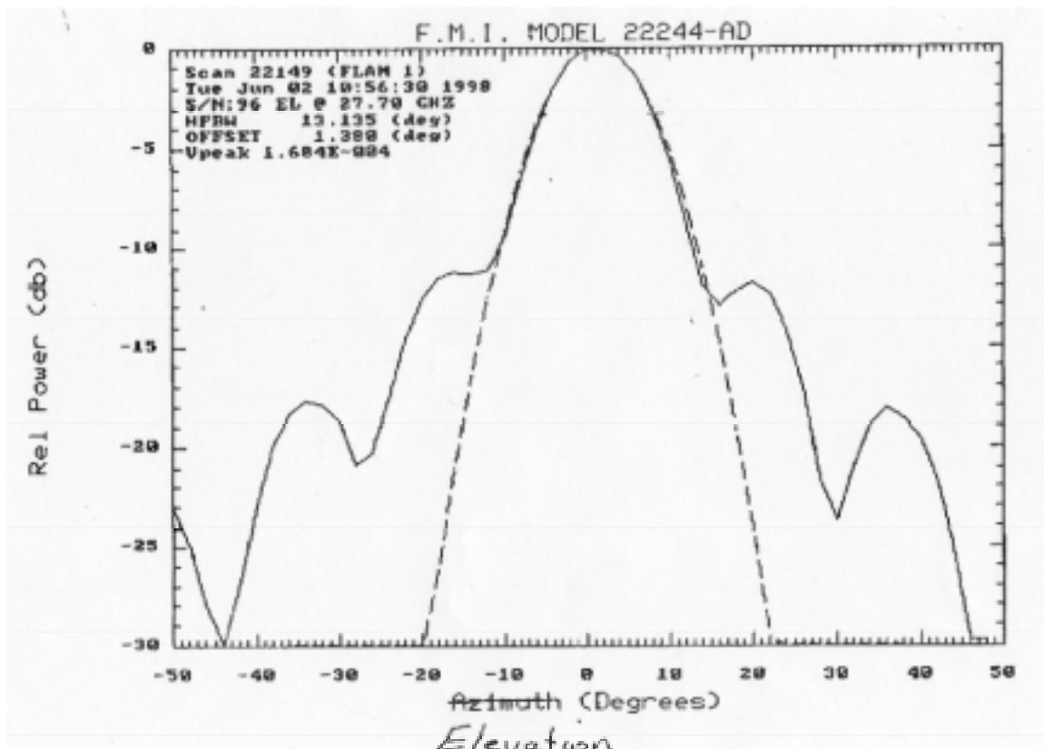
Figure 3.2-1 Elevation Beamwidth for the HUB antennas
