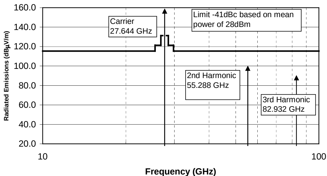
Figure 9.3-2 HUB Pilot radiated harmonic emissions
