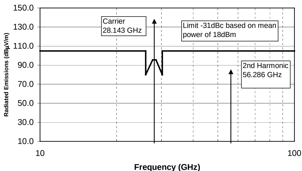
Figure 9.3-1 HUB Data radiated harmonic emissions
