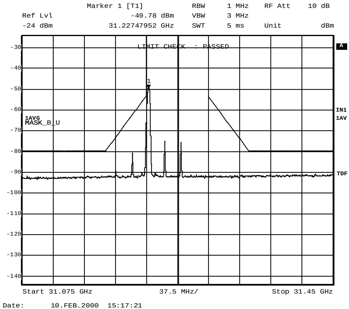
Figure 11 16 QAM data carrier at lower band edge compared to digital emission mask (101.111(a)(2)) – \pm 250\% allocated bandwidth
