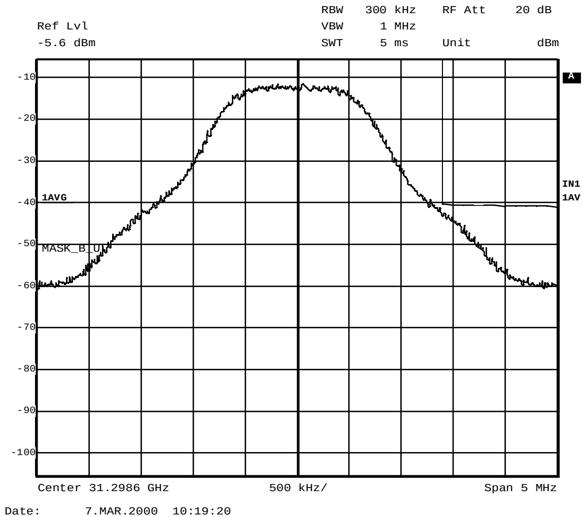
Figure 9 QPSK/ 1.28 MS/s data carrier at 31.2986 GHz compared to digital emission mask (101.111(a)(2)) – closeup of band edge
