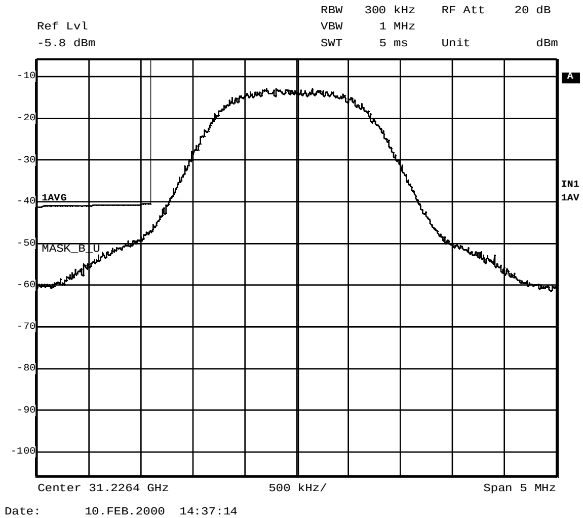
Figure 4 QPSK/ 1.28 MS/s data carrier at 31.2264 GHz compared to digital emission mask (101.111(a)(2)) – closeup of band edge
