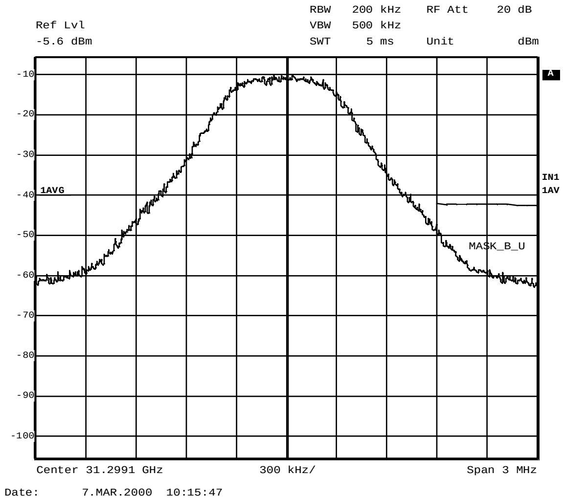
Figure 8 QPSK/ 0.64 MS/s data carrier at 31.2991 GHz compared to digital emission mask (101.111(a)(2)) – closeup of band edge
