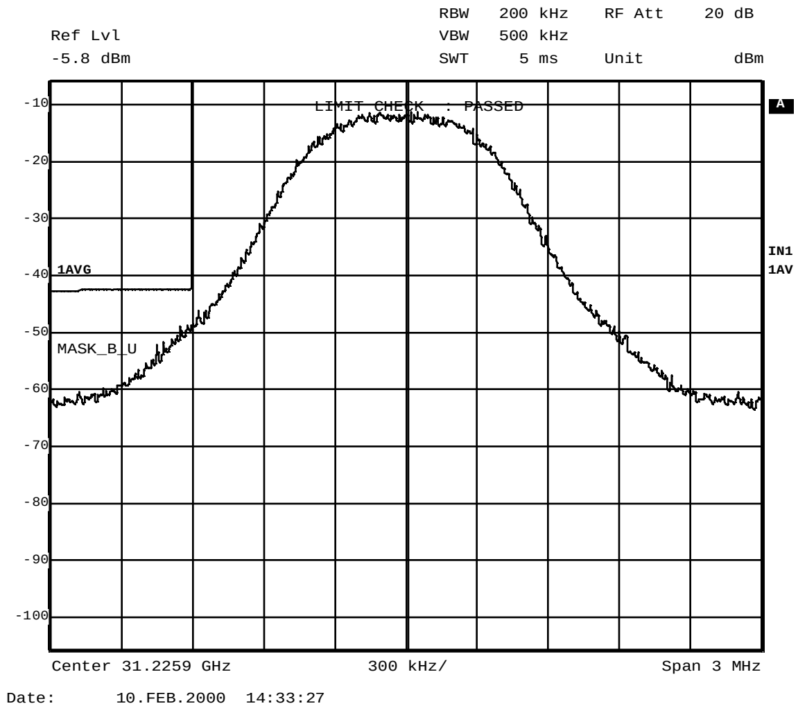
Figure 3 QPSK/ 0.64 MS/s data carrier at 31.2259 GHz compared to digital emission mask (101.111(a)(2)) – closeup of band edge
