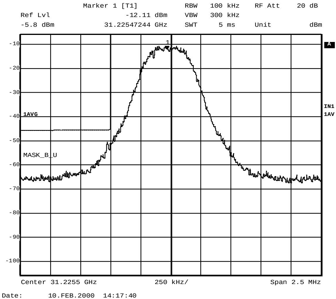
Figure 2 QPSK/ 0.32 MS/s data carrier at 31.2255 GHz compared to digital emission mask (101.111(a)(2)) – closeup of band edge
