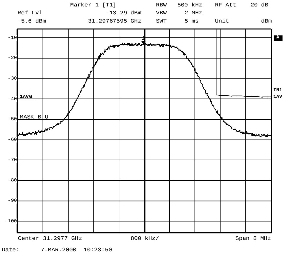
Figure 10 QPSK/ 2.56 MS/s data carrier at 31.2977 GHz compared to digital emission mask (101.111(a)(2)) – closeup of band edge
