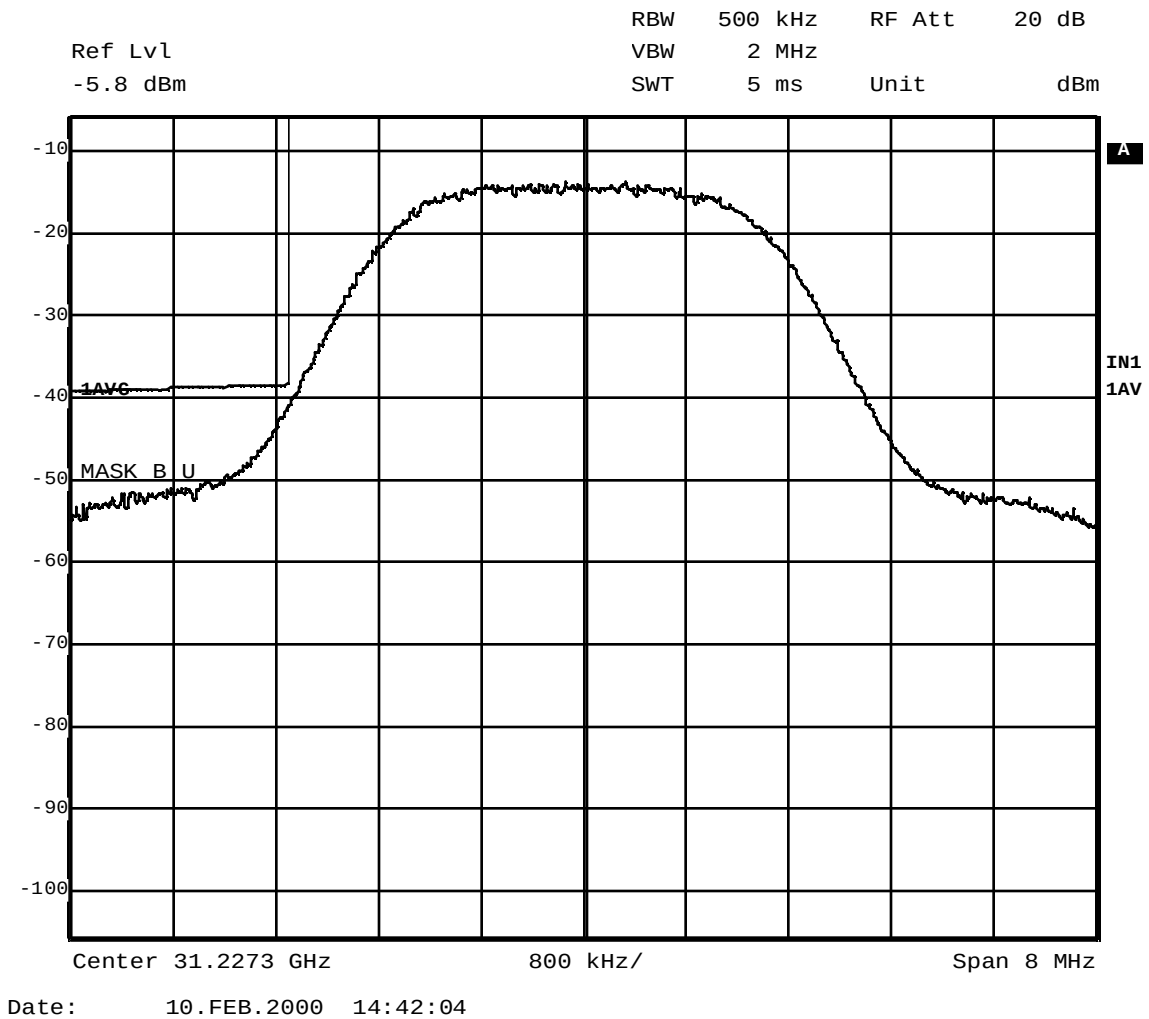
Figure 5 QPSK/ 2.56 MS/s data carrier at 31.2273 GHz compared to digital emission mask (101.111(a)(2)) – closeup of band edge
