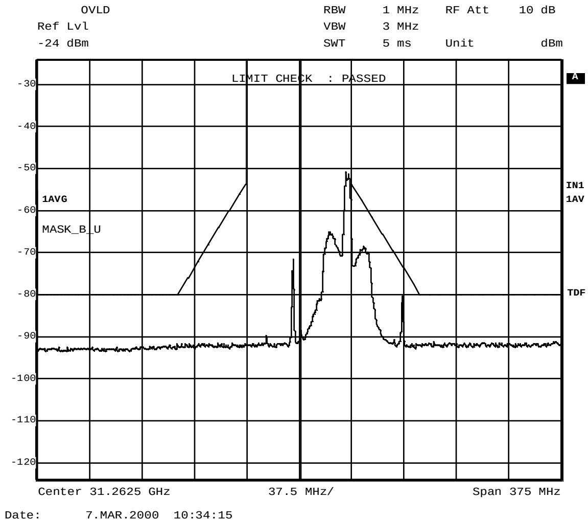
Figure 12 16 QAM data carrier at upper band edge compared to digital emission mask (101.111(a)(2)) – \pm 250\% allocated bandwidth
