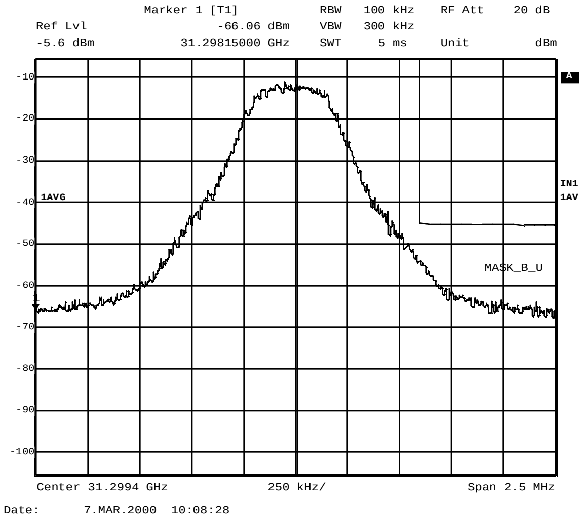
Figure 6 16 QAM data carrier at 31.2994 GHz compared to digital emission mask (101.111(a)(2)) – closeup of band edge
