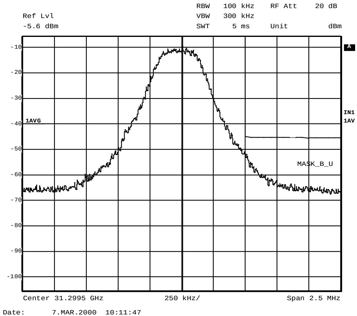
Figure 7 QPSK/ 0.32 MS/s data carrier at 31.2995 GHz compared to digital emission mask (101.111(a)(2)) – closeup of band edge
