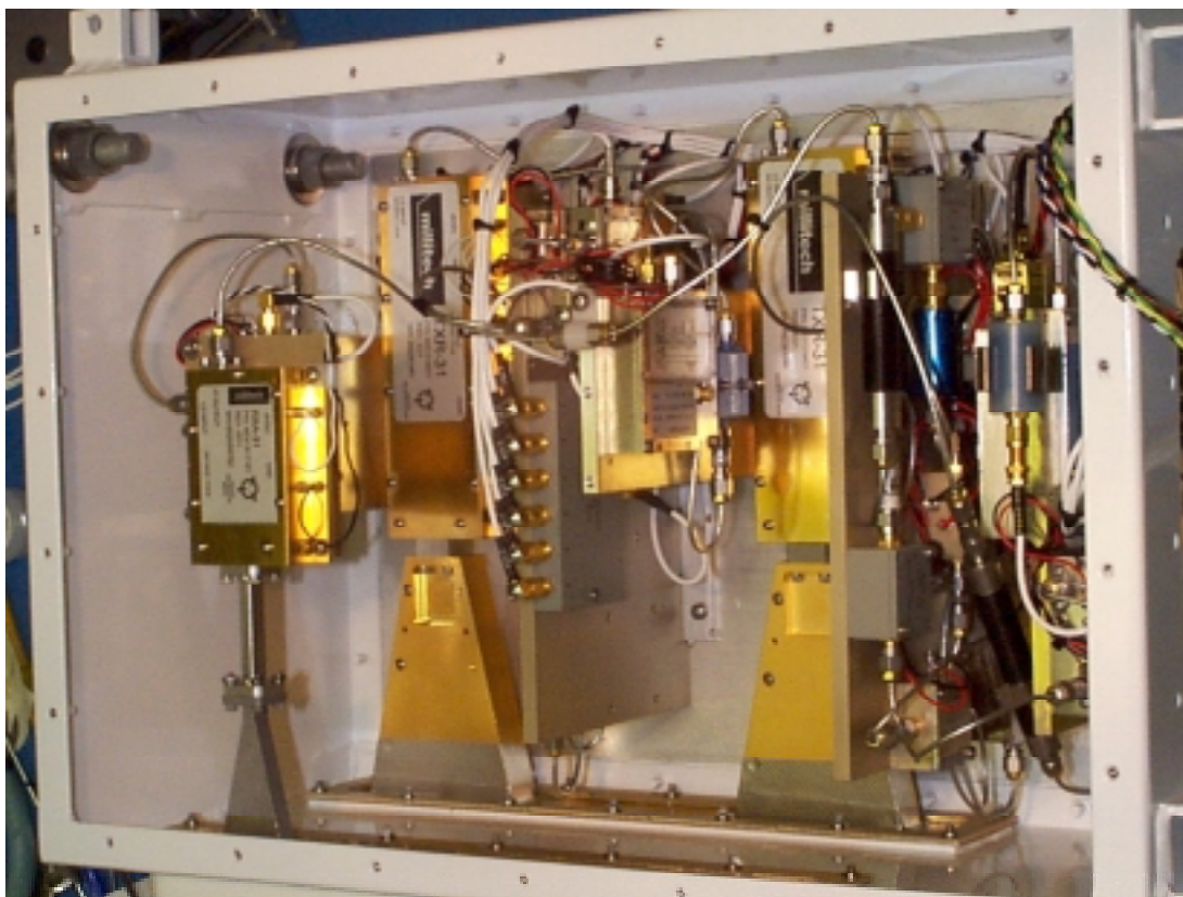
Figure 11.0-2 Internal View
