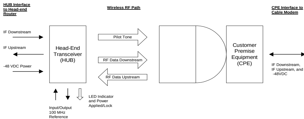
Figure 3.0-1 Major Functional Interfaces
