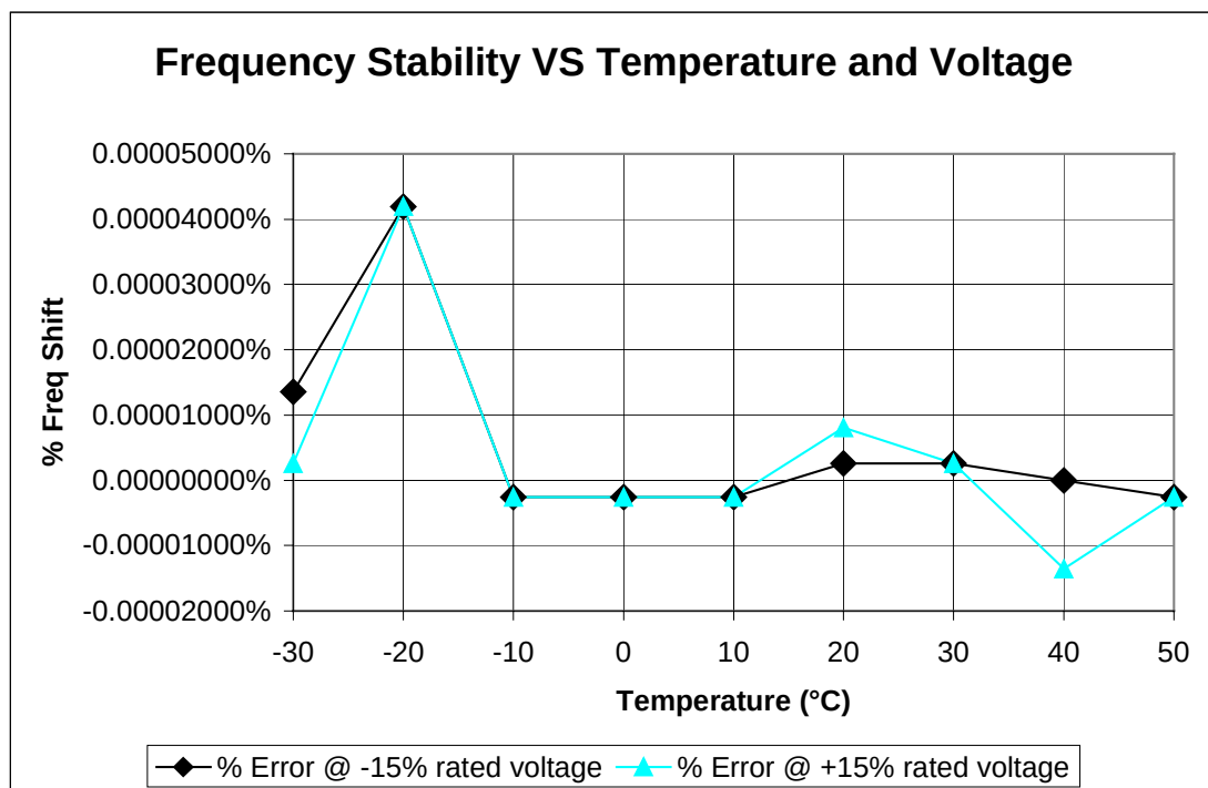
Figure 9.4-2 Frequency Stability Graph – HUB Pilot
