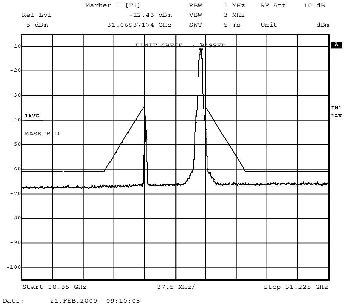
Figure 12 QPSK data carrier at 31.0694 GHz compared to digital emission mask (101.111(a)(2)) – \pm 250\% allocated bandwidth
