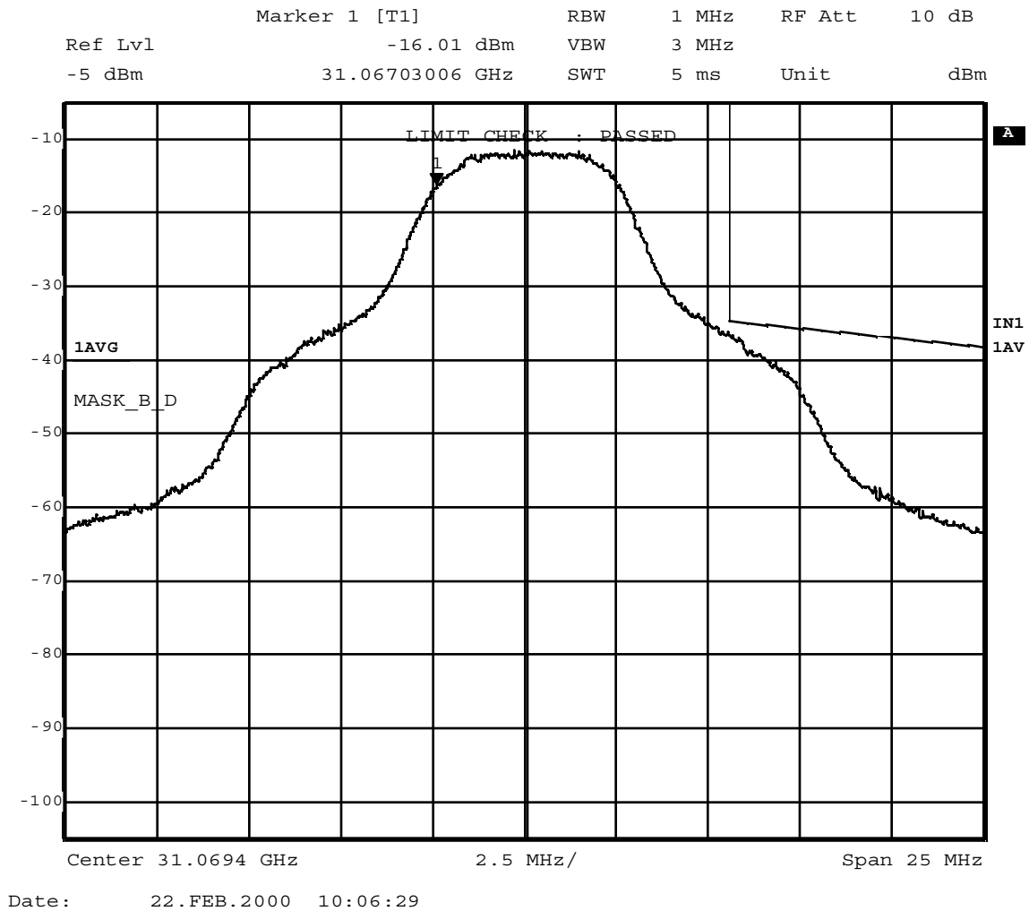
Figure 11 QPSK data carrier at 31.0694 GHz compared to digital emission mask (101.111(a)(2)) – closeup of band edge
