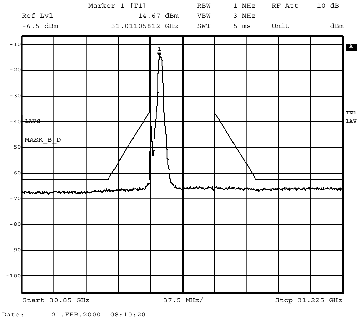
Figure 4 64 QAM data carrier at 31.012 GHz compared to digital emission mask (101.111(a)(2)) – \pm 250\% allocated bandwidth
