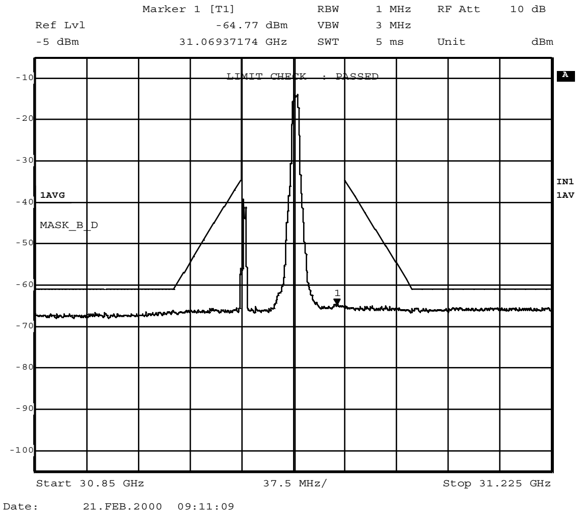
Figure 5 64 QAM data carrier at 31.039 GHz compared to digital emission mask (101.111(a)(2)) – \pm 250\% allocated bandwidth
