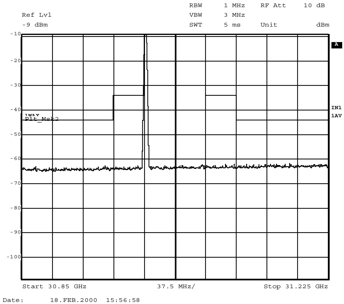
Figure 2 Pilot carrier compared to analog emission mask (101.111(a)(1)) – \pm 250 % allocated bandwidth
