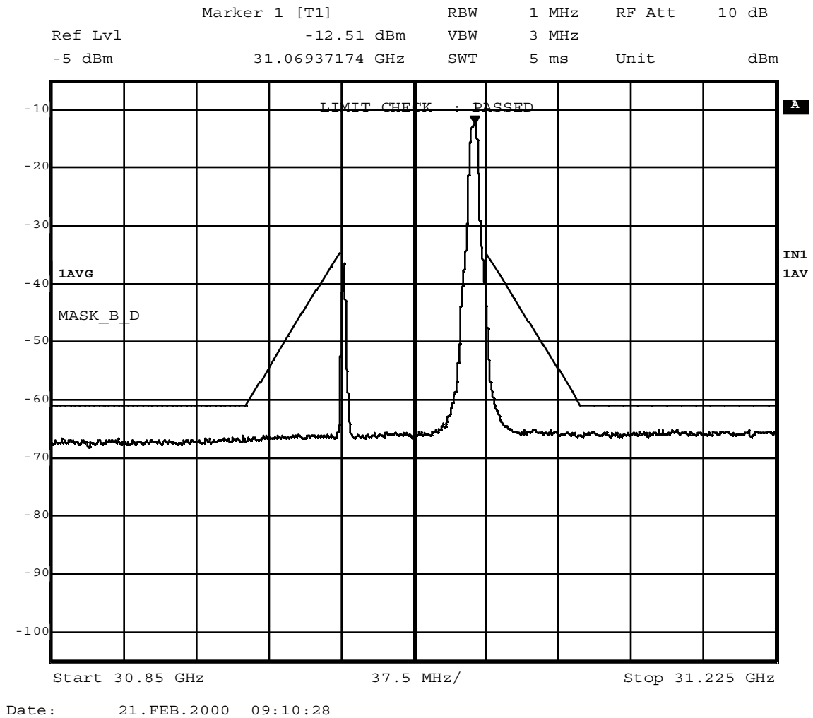
Figure 7 64 QAM data carrier at 31.0694 GHz compared to digital emission mask (101.111(a)(2)) – \pm 250 % allocated bandwidth
