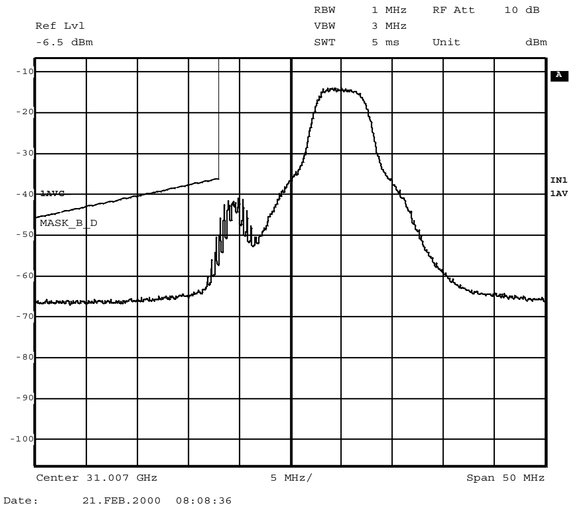
Figure 3 64 QAM data carrier at 31.012 GHz compared to digital emission mask (101.111(a)(2)) – closeup of band edge
