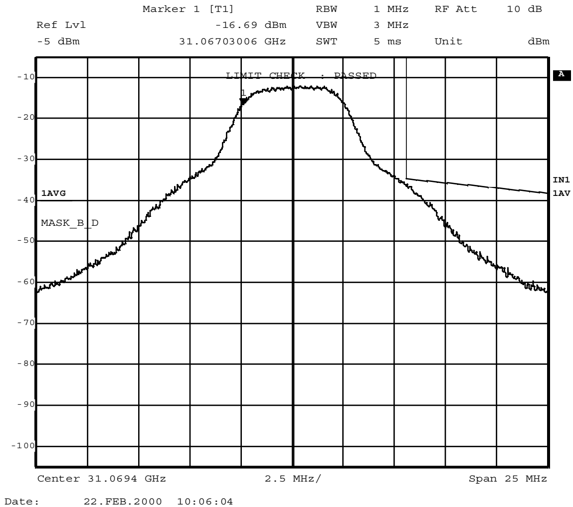
Figure 6 64 QAM data carrier at 31.0694 GHz compared to digital emission mask (101.111(a)(2)) – closeup of band edge
