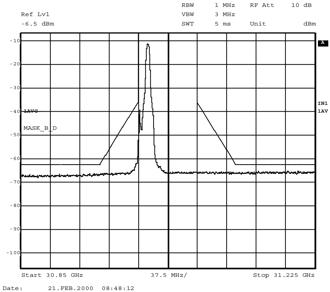
Figure 9 QPSK data carrier at 31.012 GHz compared to digital emission mask (101.111(a)(2)) – \pm 250\% allocated bandwidth
