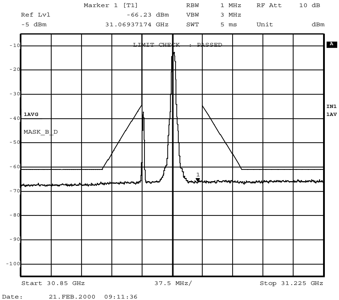
Figure 10 QPSK data carrier at 31.039 GHz compared to digital emission mask (101.111(a)(2)) – \pm 250\% allocated bandwidth
