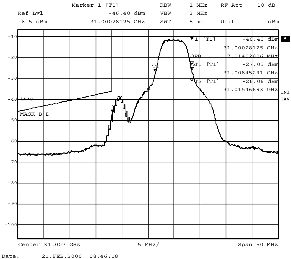
Figure 8 QPSK data carrier at 31.012 GHz compared to digital emission mask (101.111(a)(2)) – closeup of band edge
