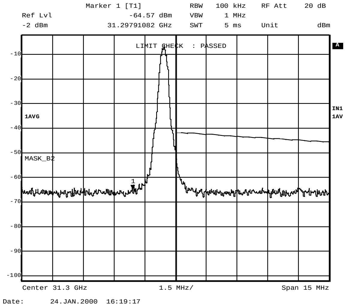
Figure B – 7 Emission Mask; 31.2994 GHz; QPSK 0.32 MS/s
