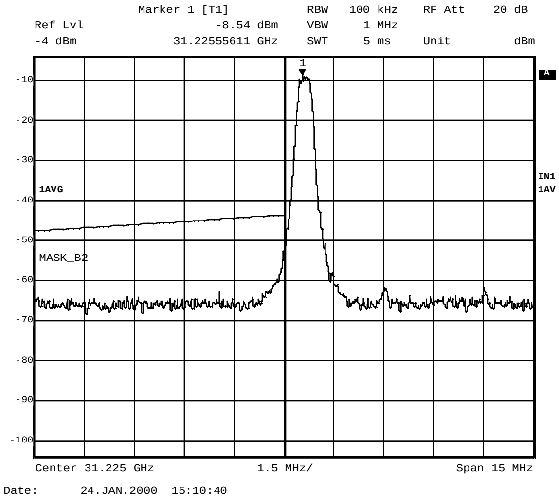
Figure B – 1 Emission Mask; 31.2255 GHz; 16 QAM 0.384 MS/s
