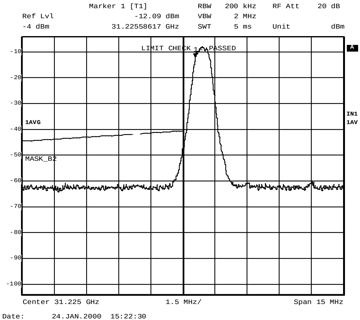
Figure B – 3 Emission Mask; 31.2259 GHz; QPSK 0.64 MS/s
