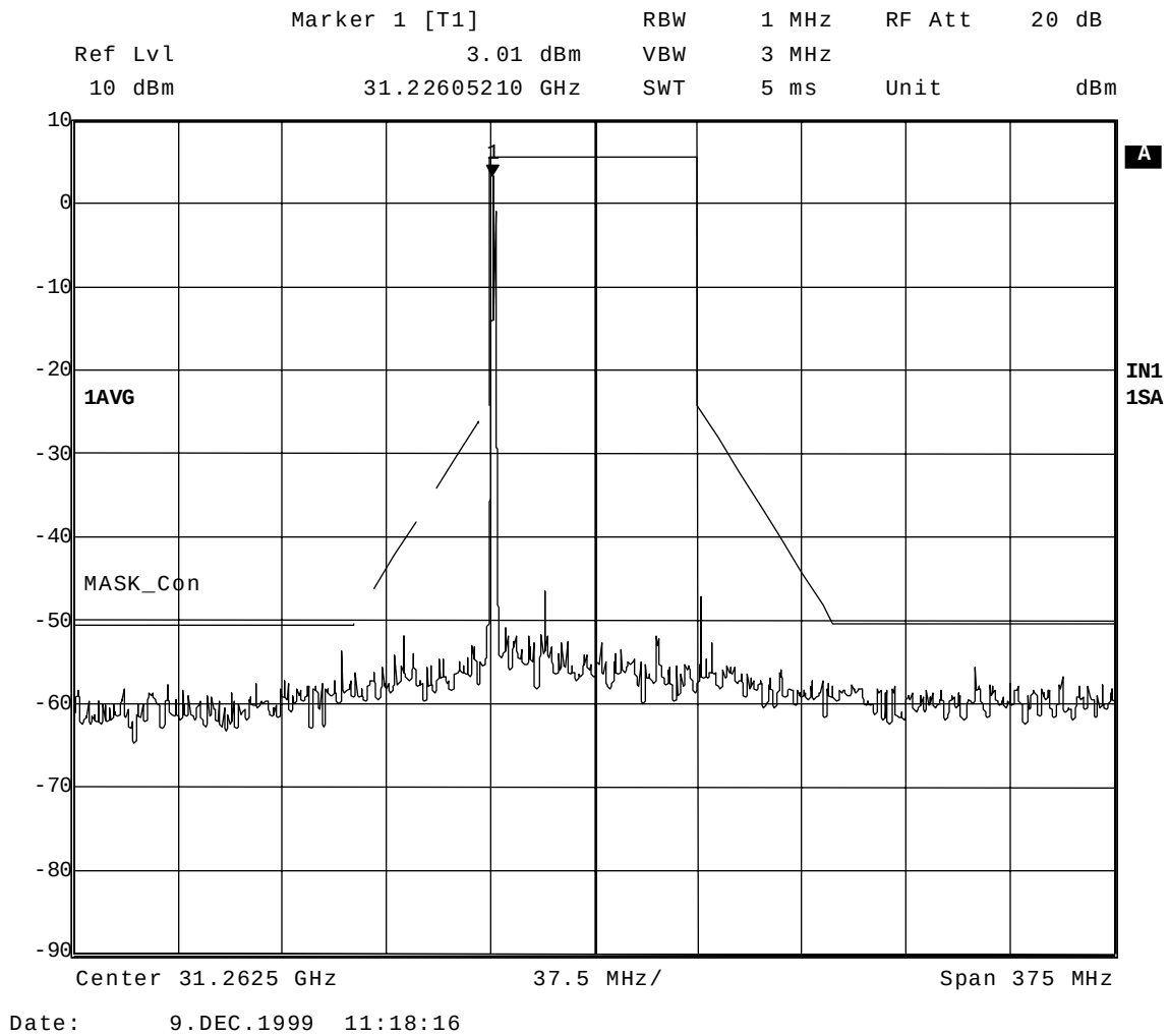
Figure B – 11 Emission Mask \pm 250\% ; 31.2255 GHz; 16 QAM 0.384 MS/s
