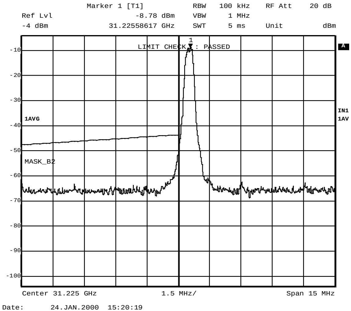
Figure B – 2 Emission Mask; 31.2255 GHz; QPSK 0.32 MS/s
