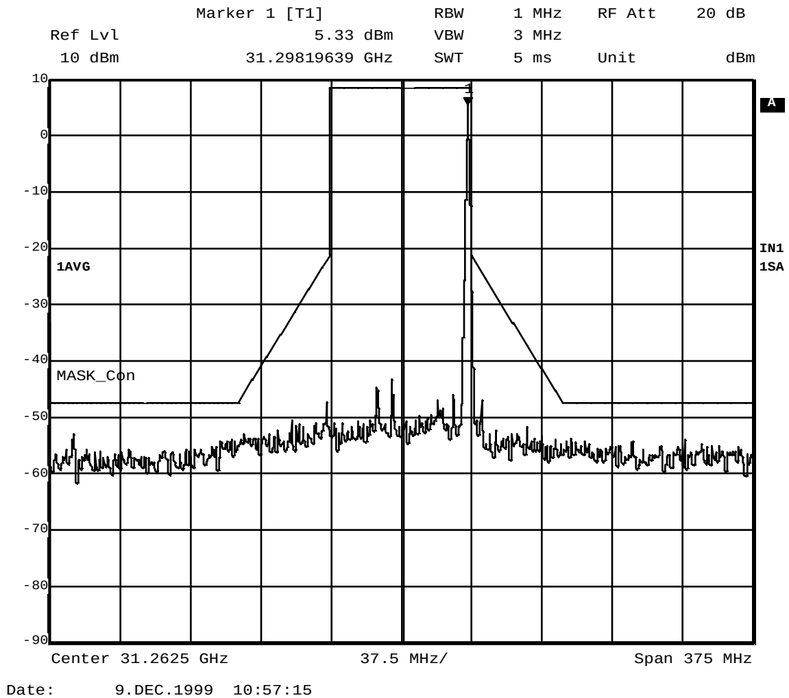
Figure B – 13 Emission Mask \pm 250\% ; 31.2994 GHz; 16 QAM 0.384 MS/s
