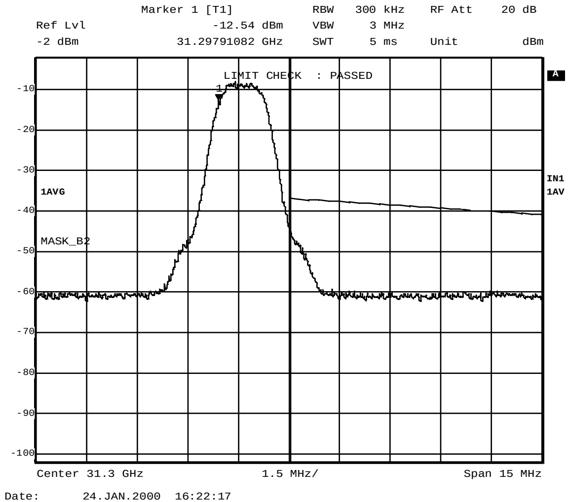
Figure B – 9 Emission Mask; 31.2986 GHz; QPSK 1.28 MS/s
