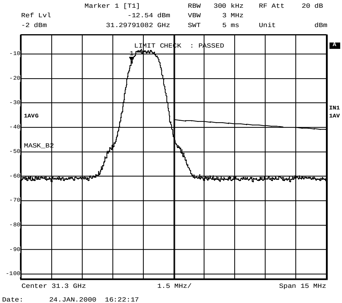
Figure B – 10 Emission Mask; 31.2977 GHz; QPSK 2.56 MS/s
