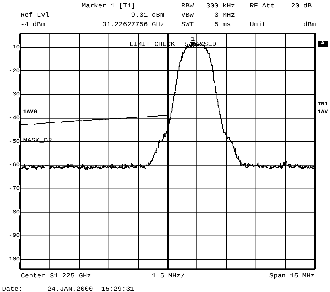
Figure B – 5 Emission Mask; 31.2274 GHz; QPSK 2.56 MS/s
