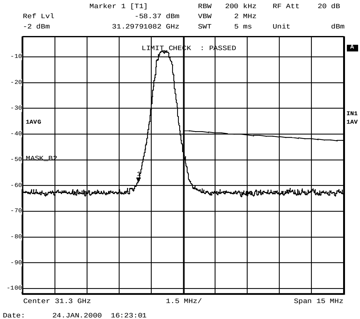
Figure B – 8 Emission Mask; 31.2991 GHz; QPSK 0.64 MS/s
