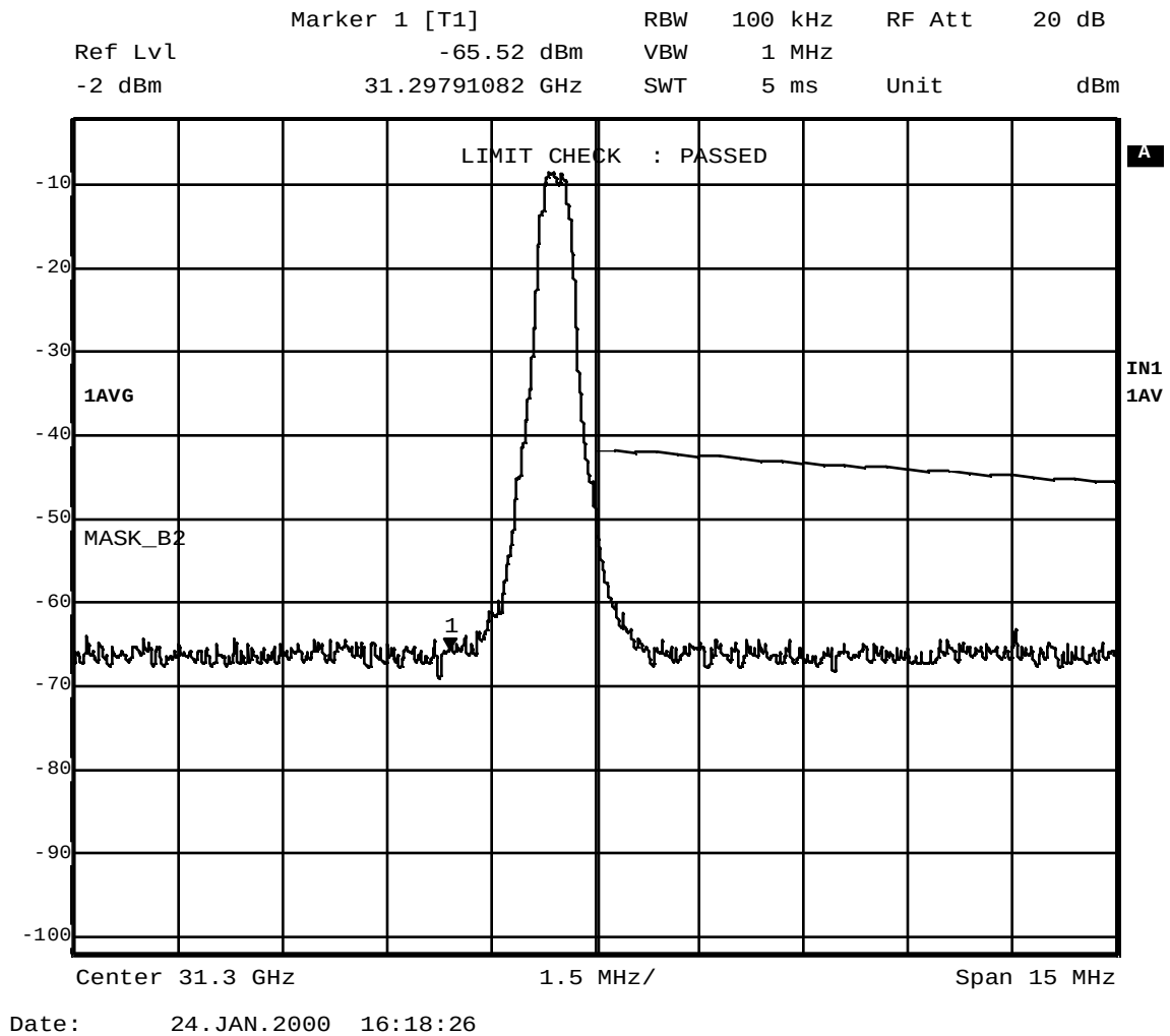
Figure B – 6 Emission Mask; 31.2994 GHz; 16 QAM 0.384 MS/s
