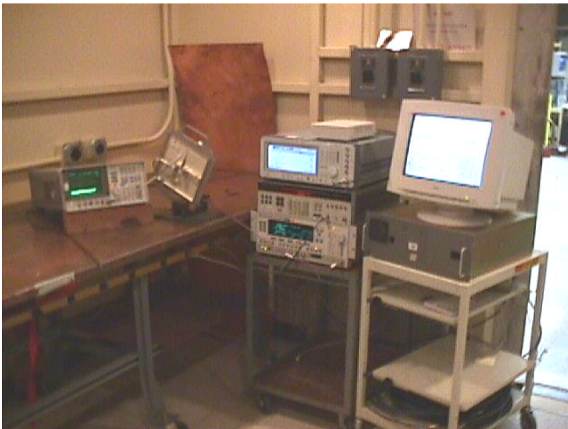
Figure 7.0-1 Conducted Emissions Test Setup
