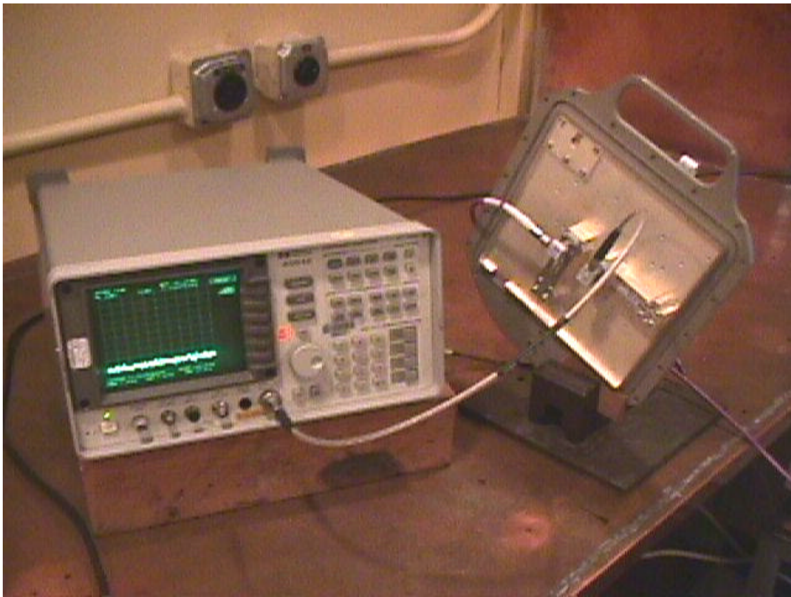
Figure 7.0-2 Conducted Emissions Test Setup (close up view)
