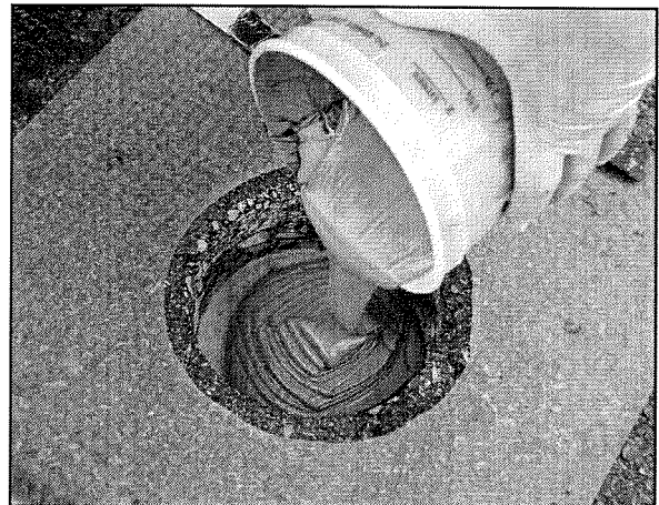
STEP 13 - Immediately pour the epoxy mixture into the hole.
