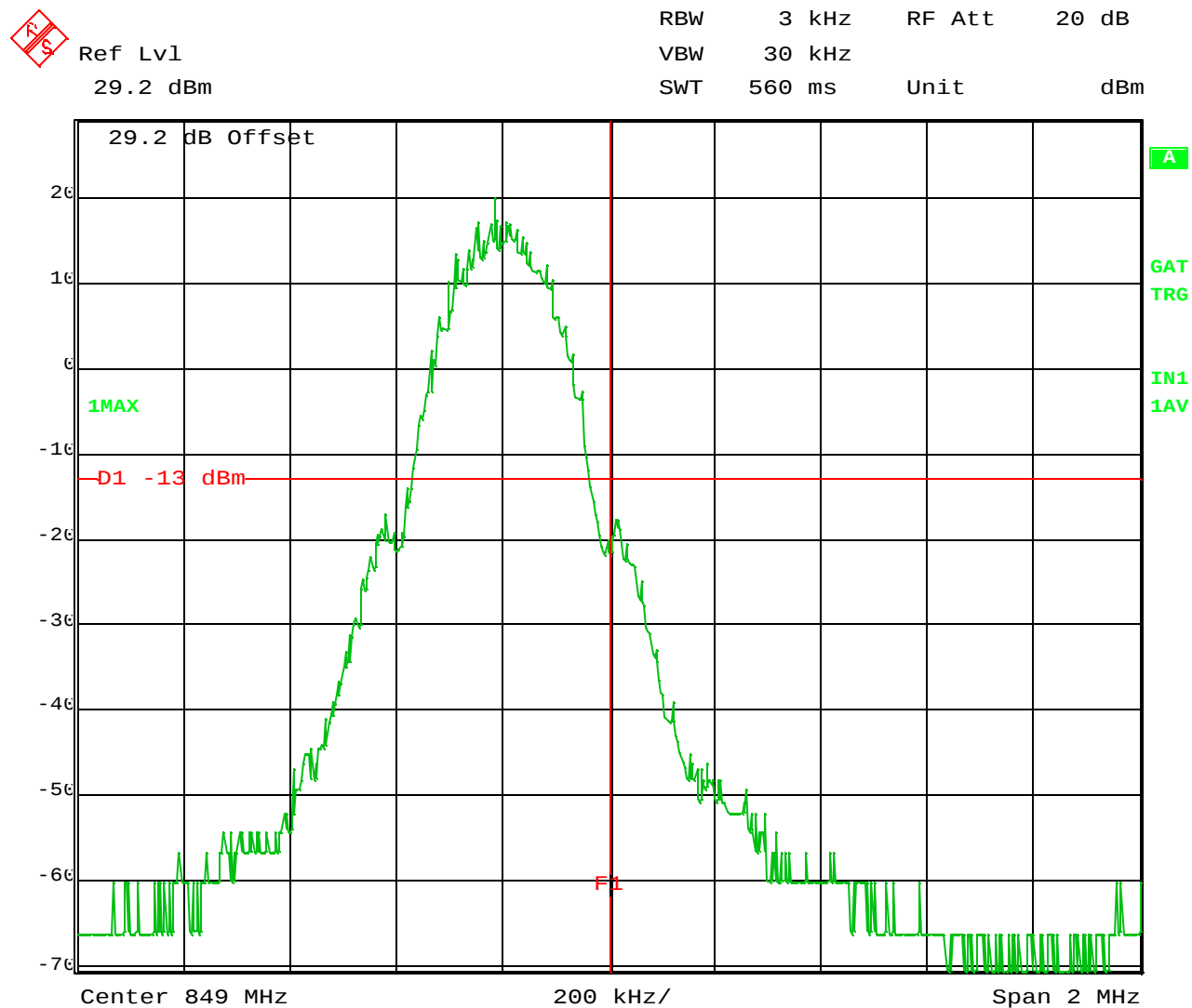
Figure 8-6: Emissions within 1 MHz of band edge, GSM 850 Upper Band Edge 1
