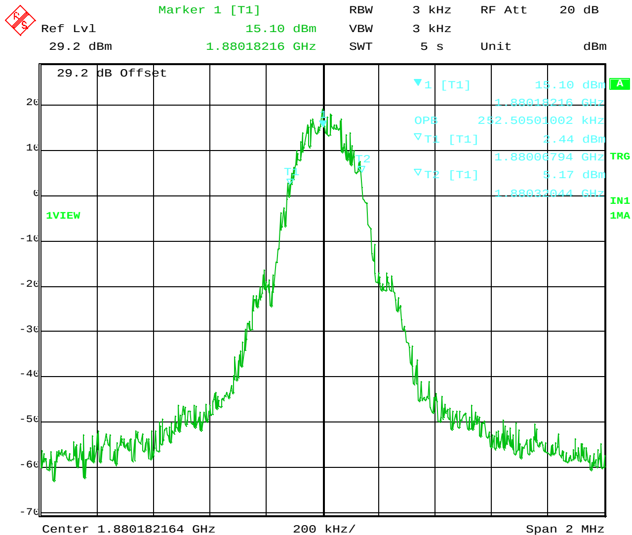
Figure 7-5: Occupied Bandwidth – GSM 662
