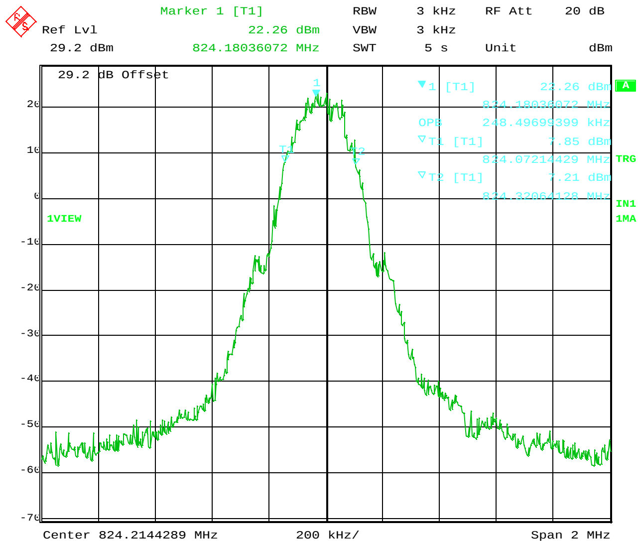
Figure 7-1: Occupied Bandwidth – GSM 128
