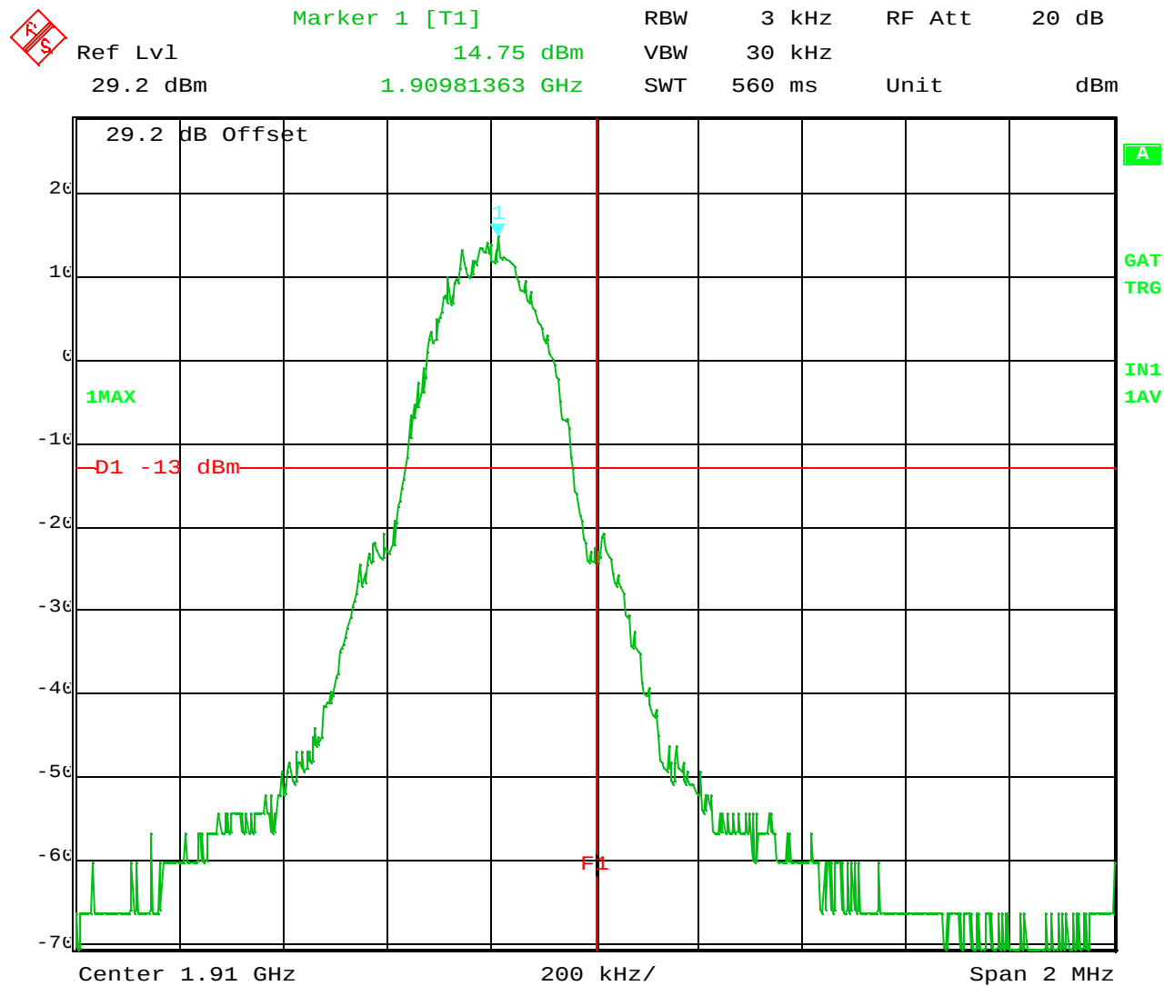
Figure 8-8: Emissions within 1 MHz of band edge, GSM 1900 Upper Band Edge
