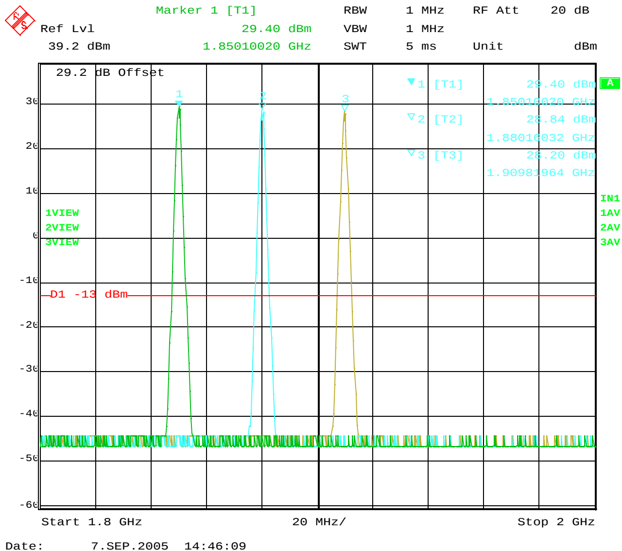
Figure 8-4: Out of band emissions at antenna terminals – GSM 1900 Channels 512, 662, 810 (Zoomed In on Carrier Frequencies)
