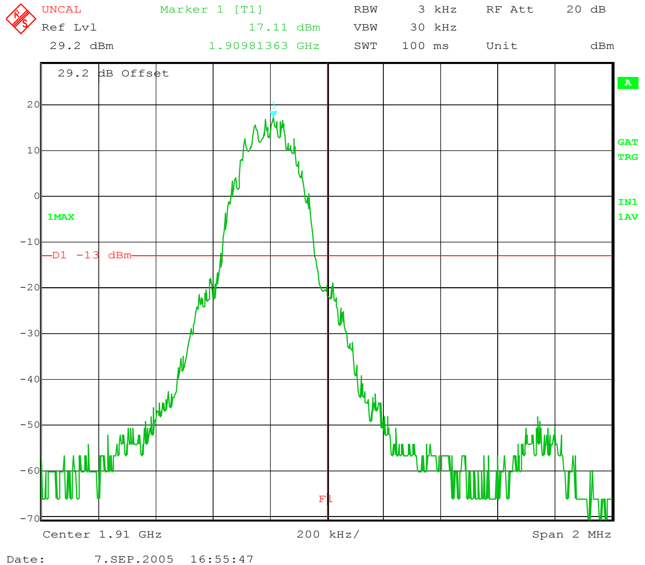
Figure 7-8: Emissions within 1 MHz of band edge, GSM 1900 Upper Band Edge
