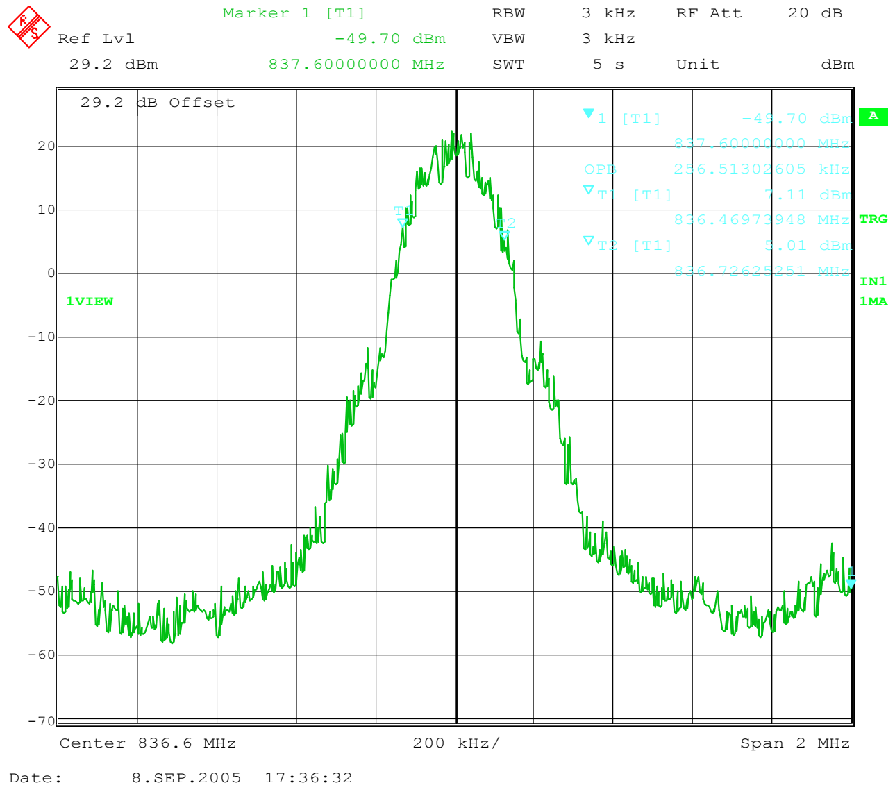
Figure 6-2: Occupied Bandwidth – GSM 190
