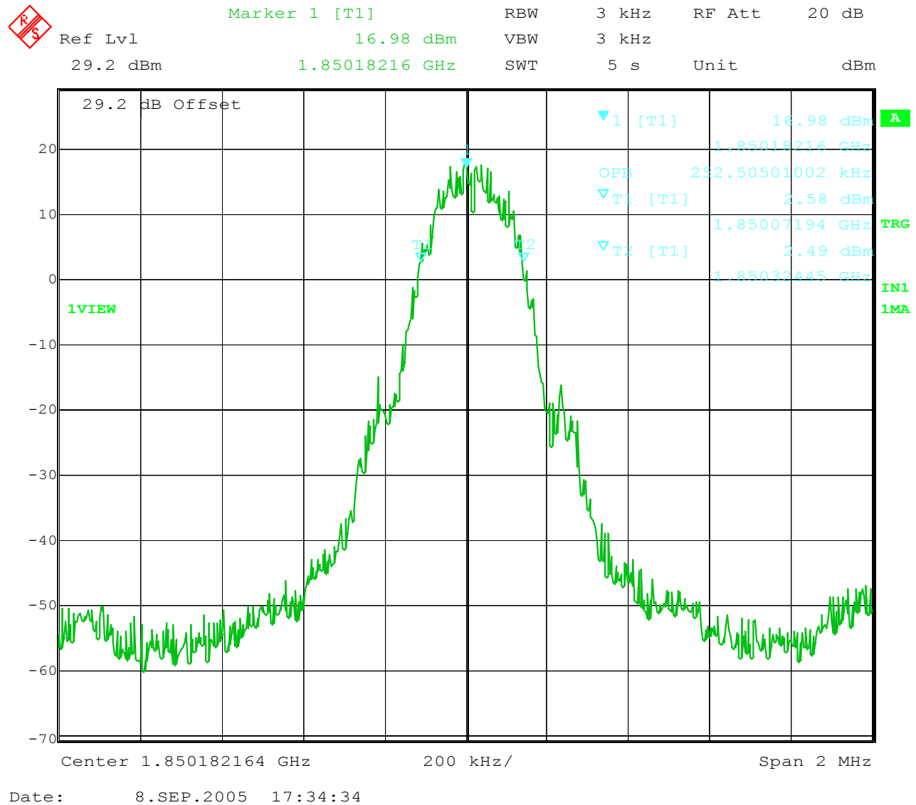
Figure 6-4: Occupied Bandwidth – GSM 512
