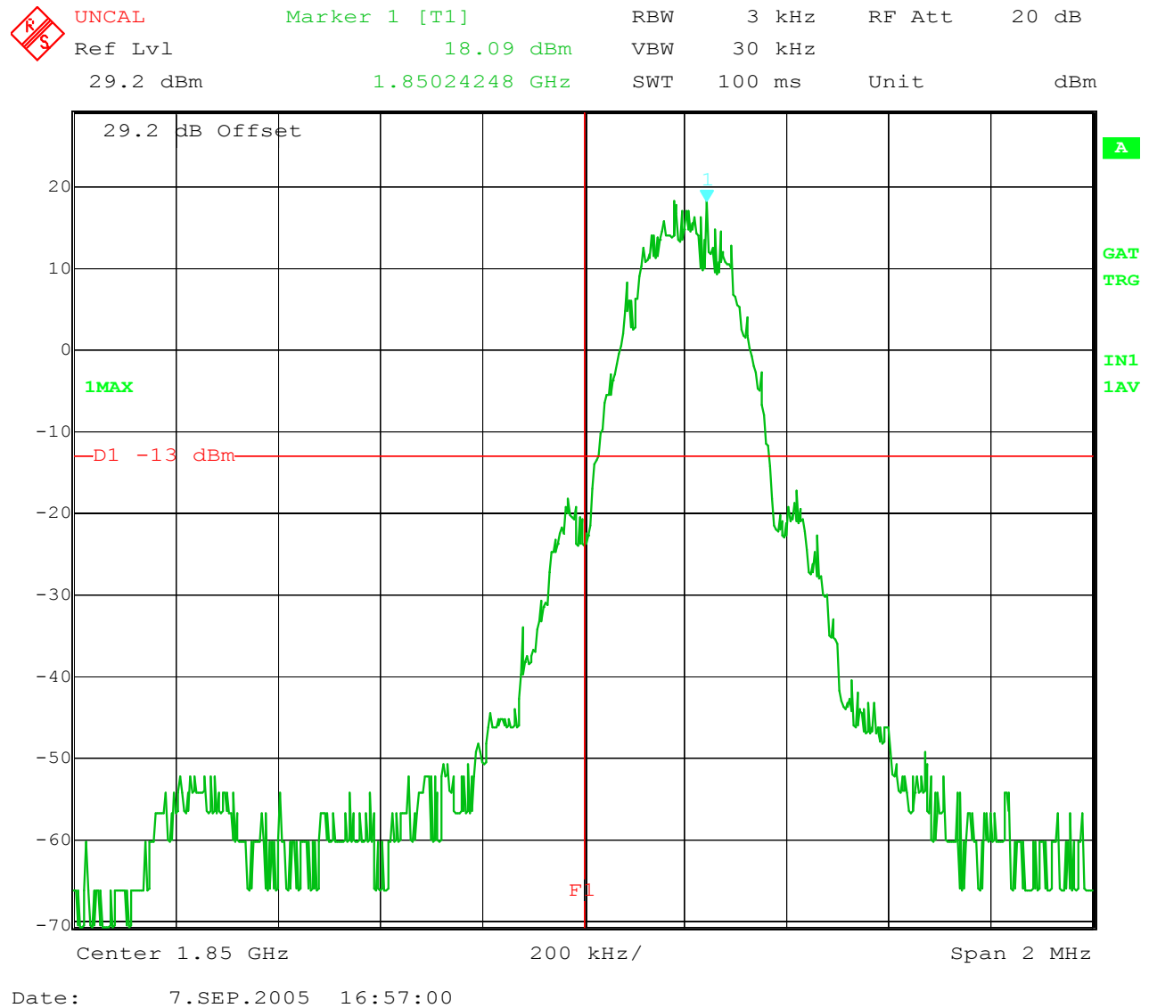
Figure 7-7: Emissions within 1 MHz of band edge, GSM 1900 Lower Band Edge
