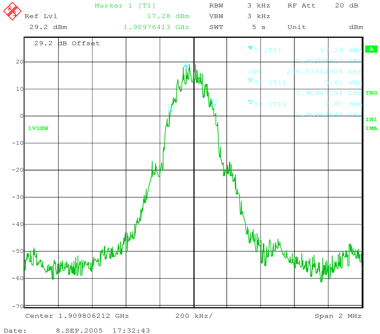
Figure 6-6: Occupied Bandwidth – GSM 810
