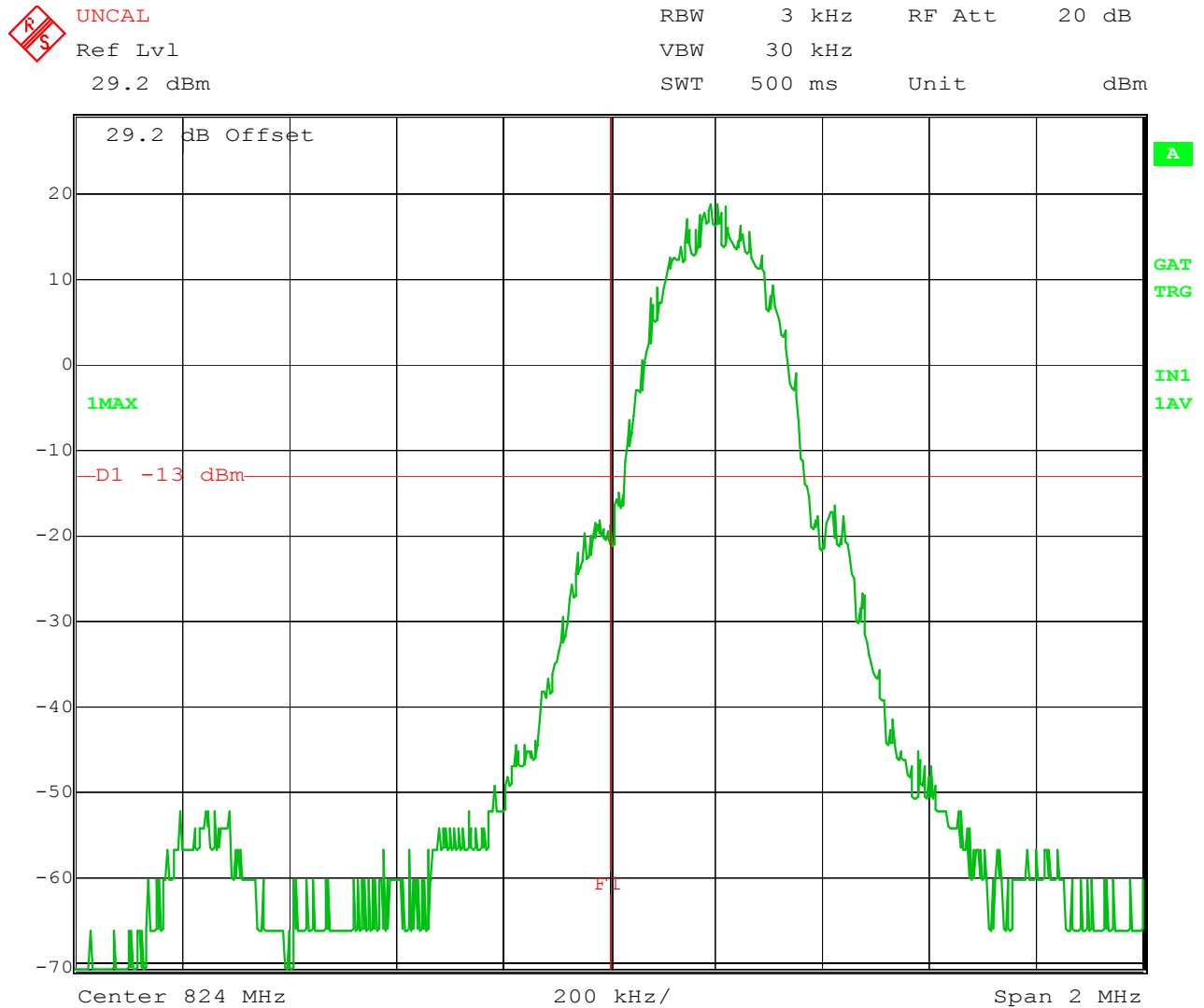
Figure 7-5: Emissions within 1 MHz of band edge, GSM 850 Lower Band Edge
