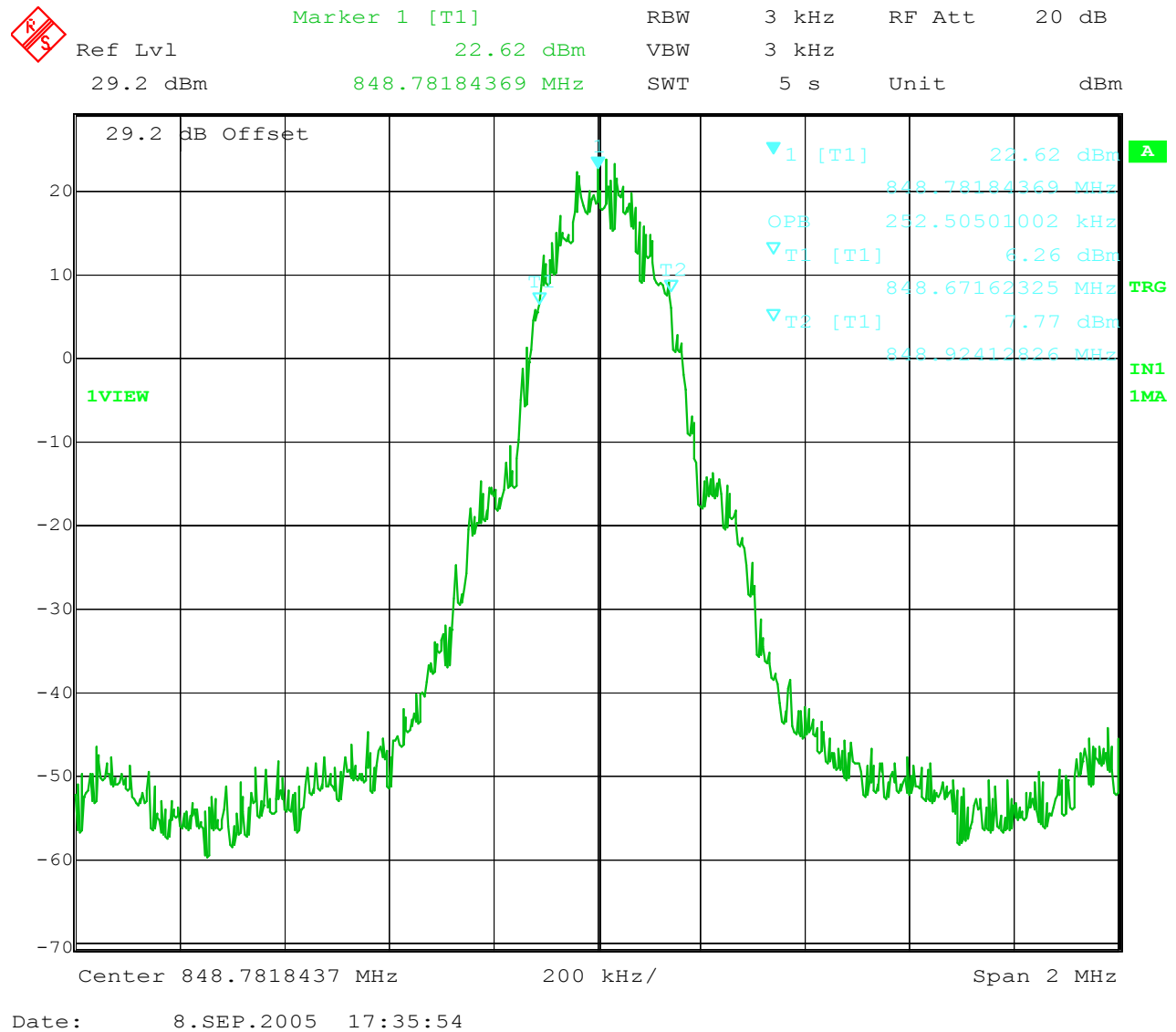
Figure 6-3: Occupied Bandwidth – GSM 251
