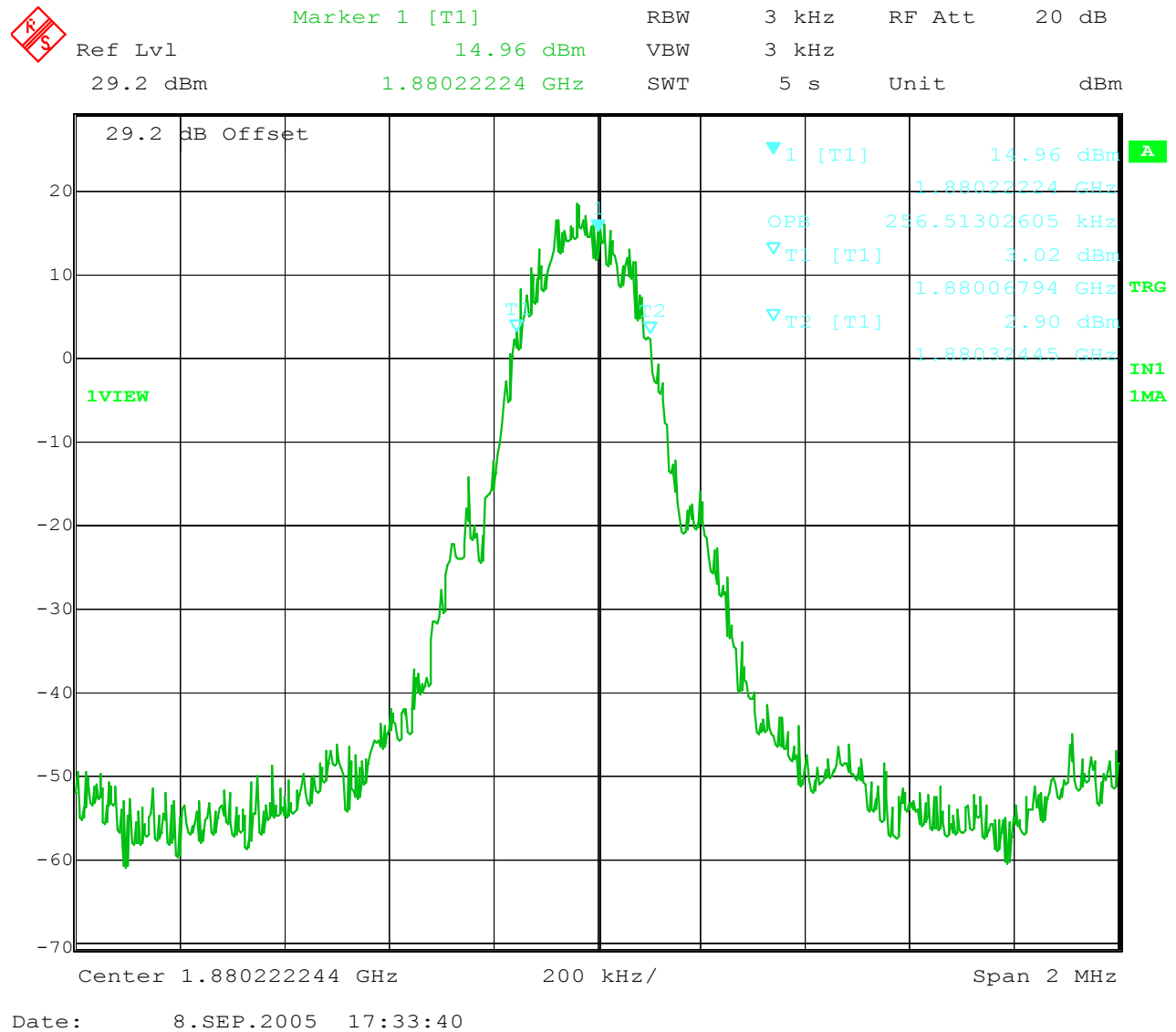
Figure 6-5: Occupied Bandwidth – GSM 662
