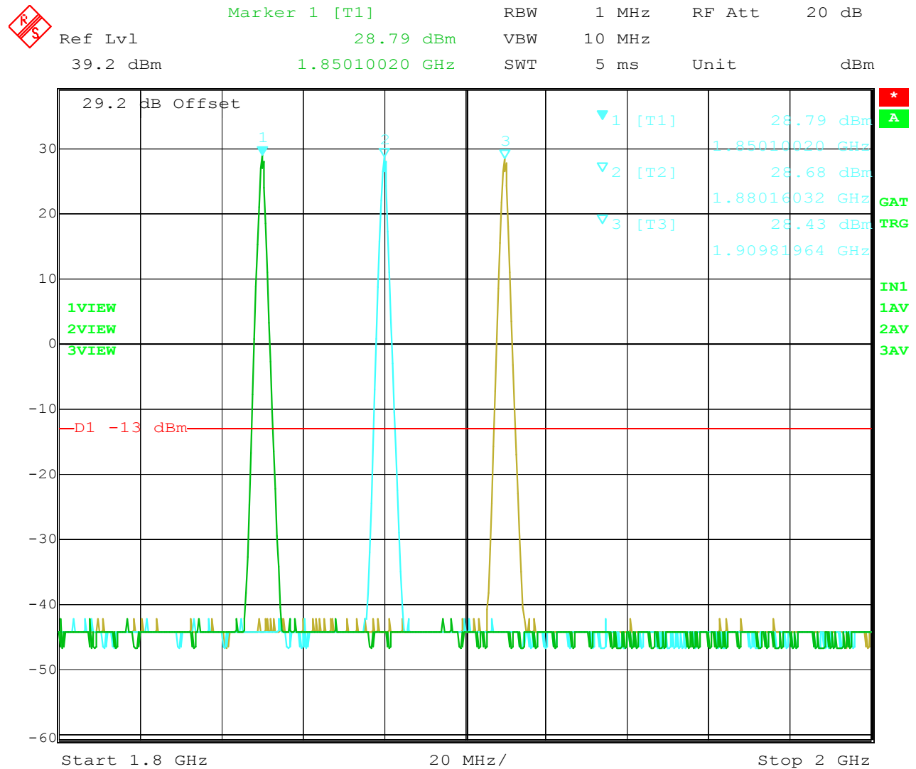
Figure 7-4: Out of band emissions at antenna terminals – GSM 1900 Channels 512, 662, 810 (Zoomed In on Carrier Frequencies)
