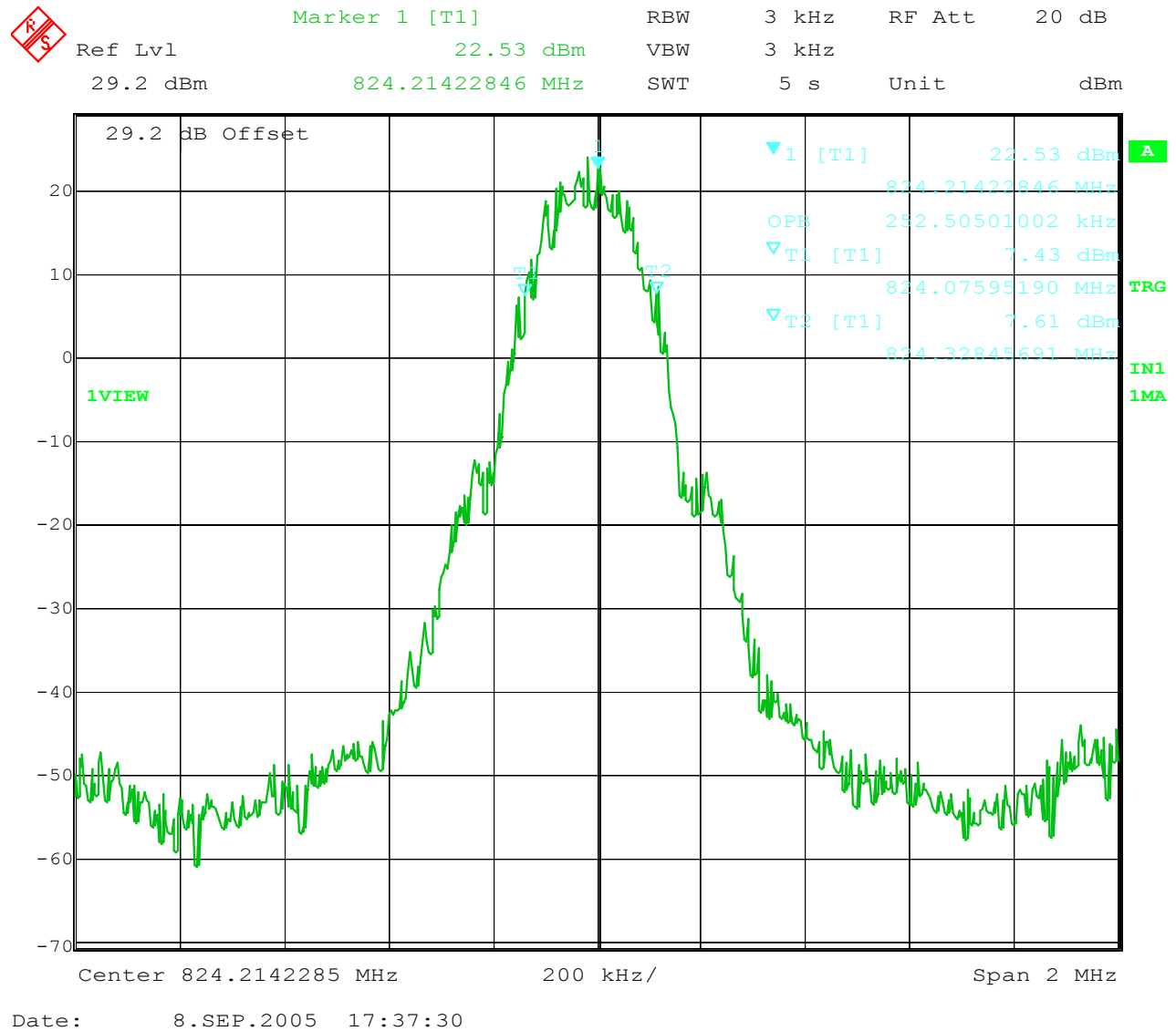
Figure 6-1: Occupied Bandwidth – GSM 128
