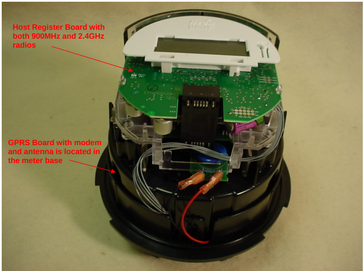
Figure 2: Internal Host Device – Antenna Location
