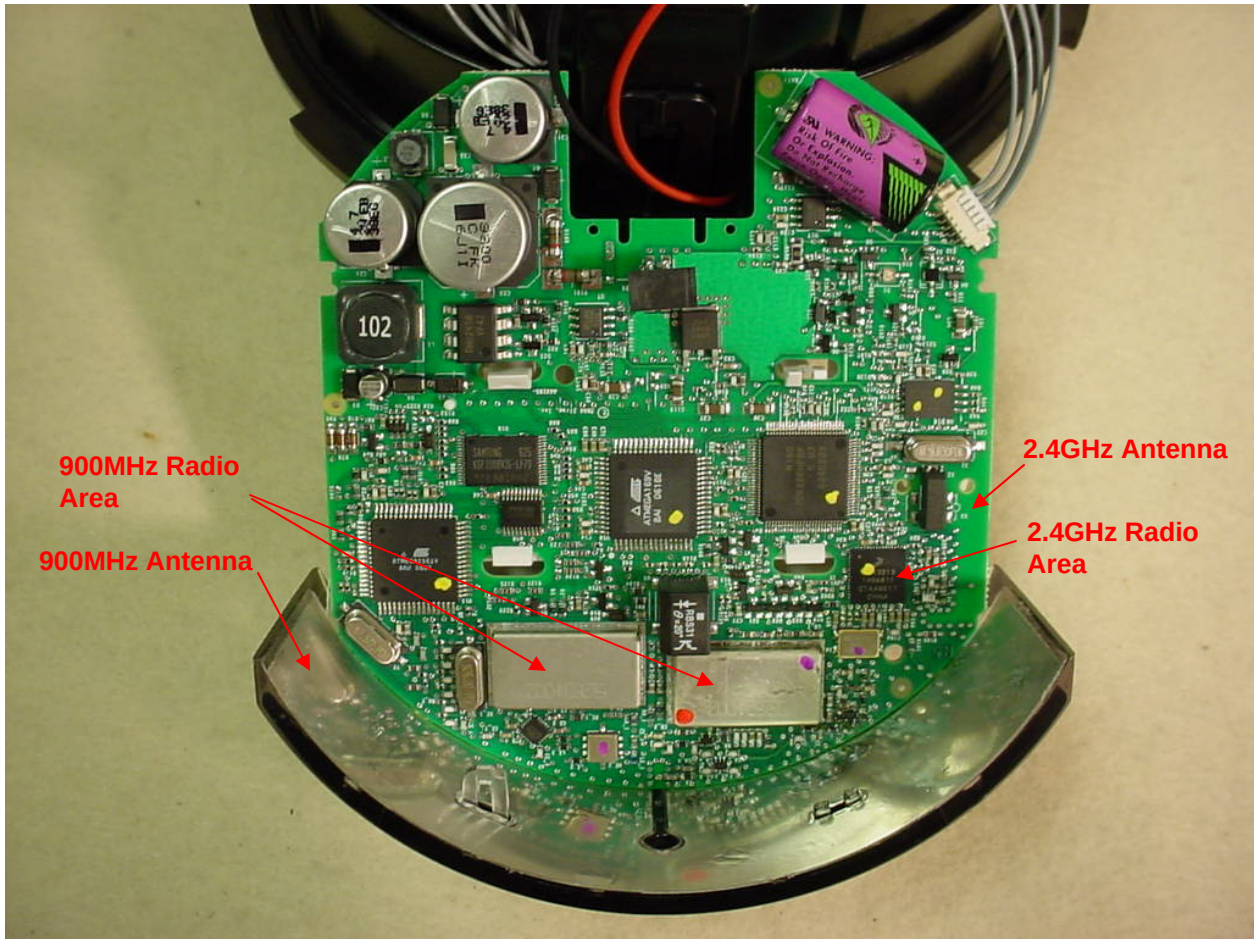
Figure 3: Internal Host Device – Antenna Location
