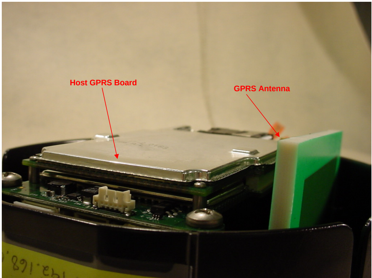
Figure 5: Internal Host Device – Host GPRS Board and Antenna
