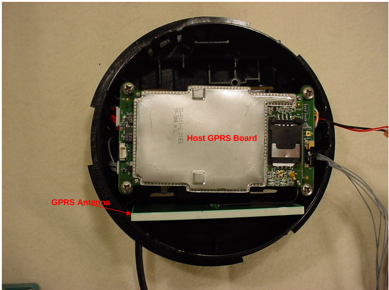
Figure 4: Internal Host Device – GPRS Board and Antenna
