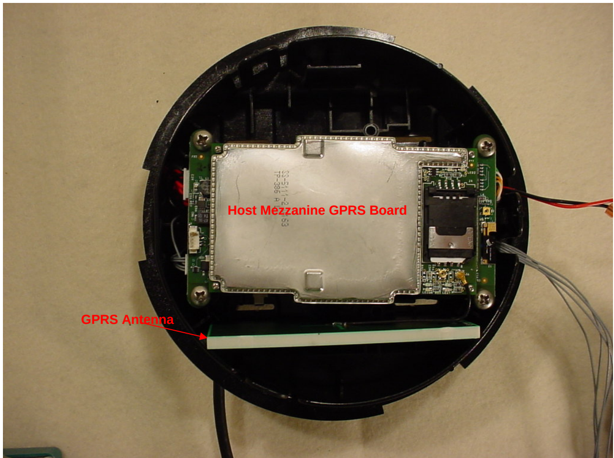
Figure 4: Internal – Host Mezzanine GPRS Board and Antenna
