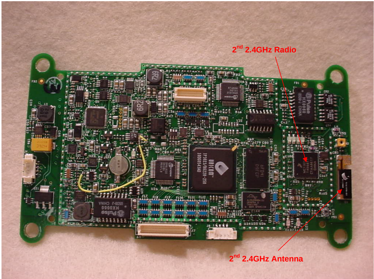
Figure 9: Internal – Host Cell Relay Core Board – 2.4GHz Radio and Antenna Location
