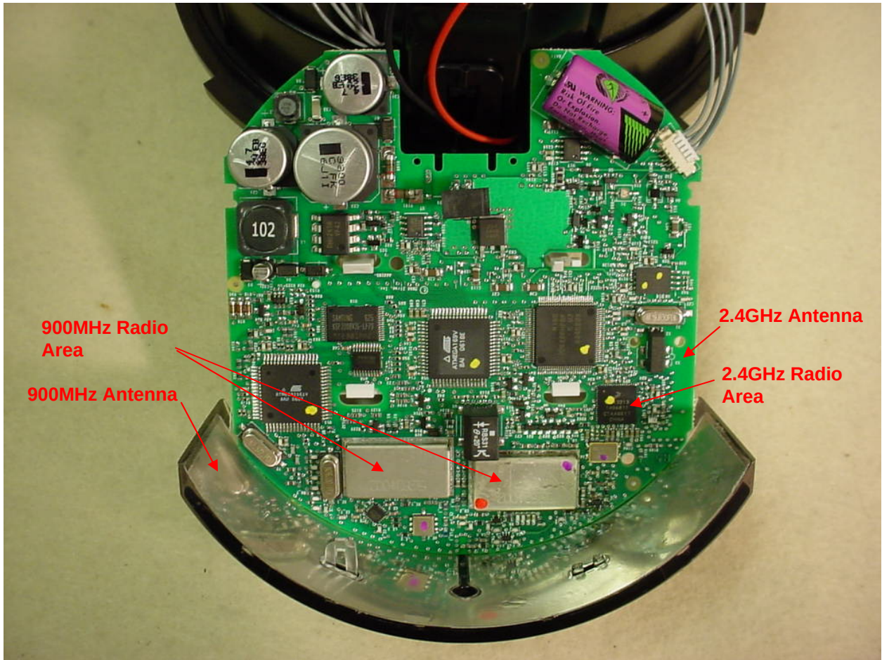
Figure 3: Internal – Host Register Board Radio and Antenna Location
