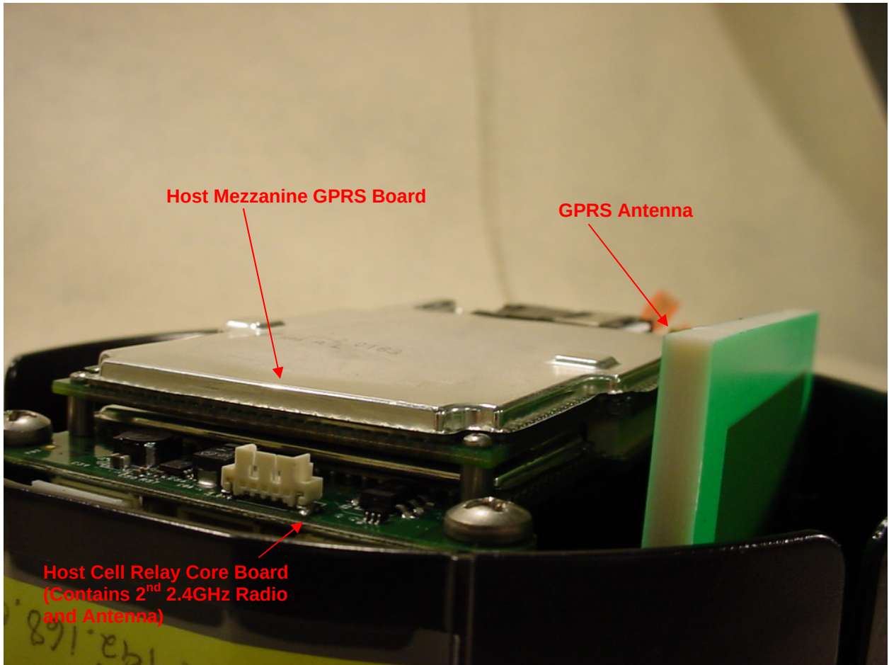
Figure 5: Internal – Host Mezzanine GPRS Board and Host Cell Relay Core Board
