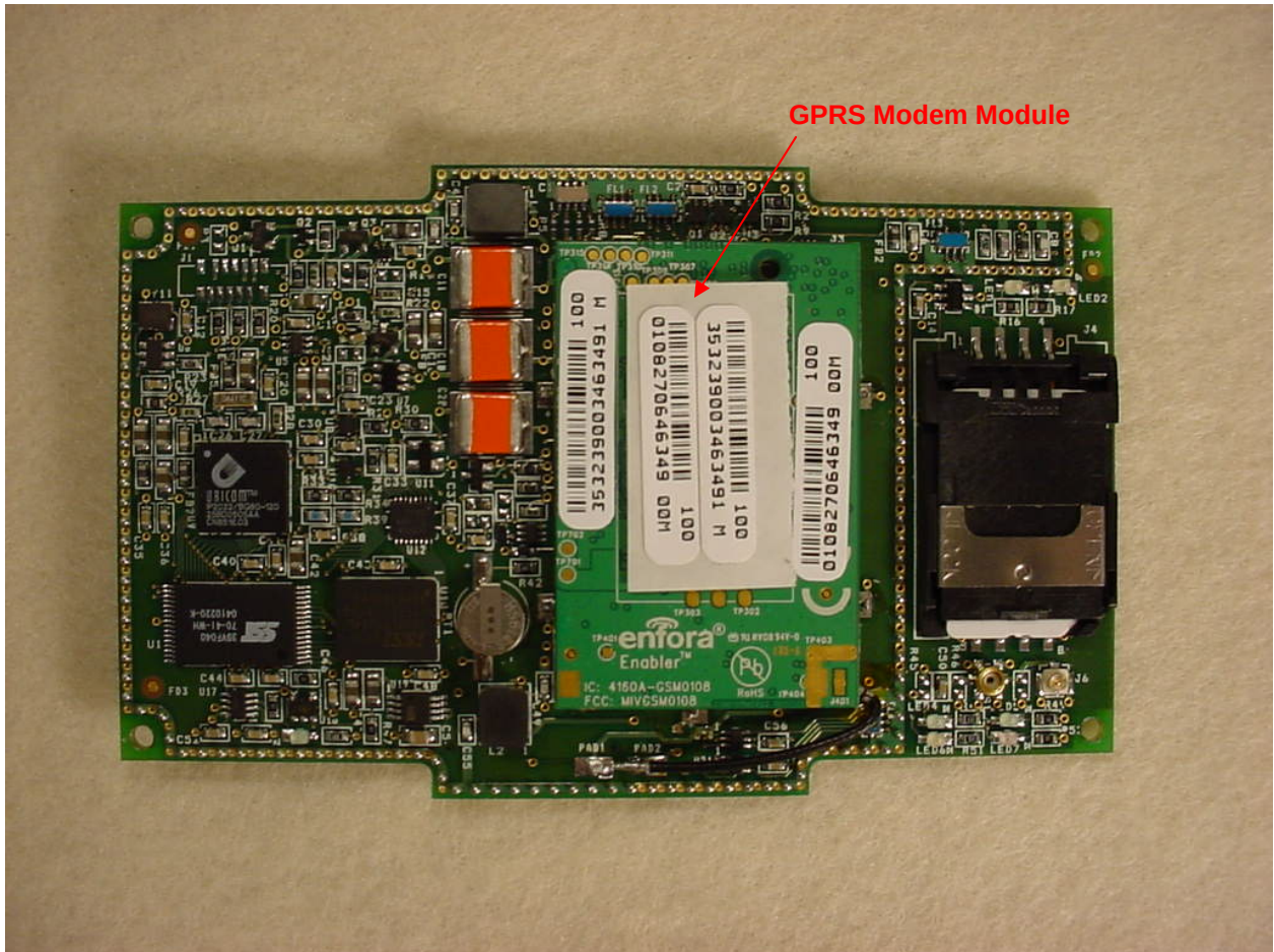
Figure 7: Internal – Host Mezzanine GPRS Board Front w/o Shields
