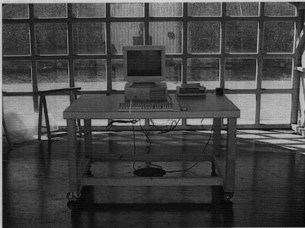
Front view of radiated measurement
