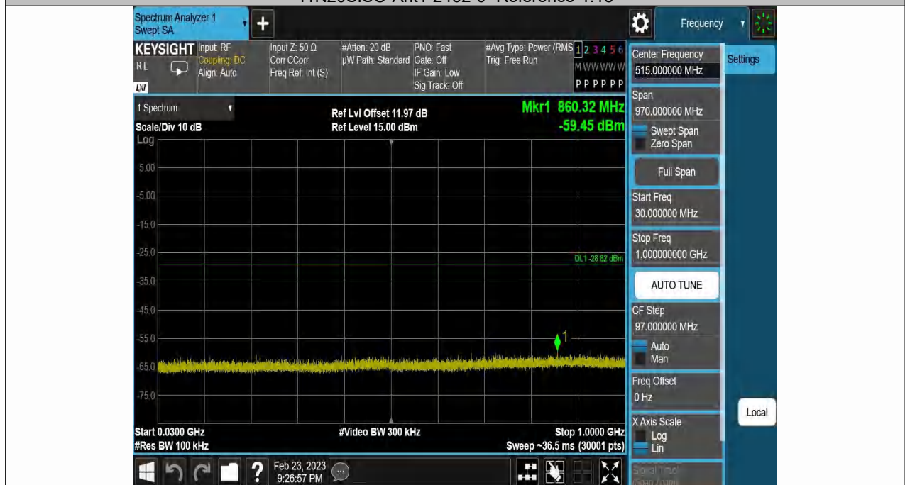
11N20SISO-Ant1-2462-30~1000-1.18
