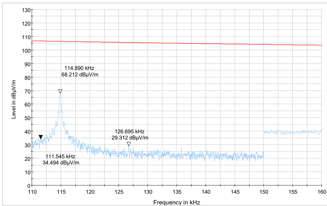
Band Edge from 110kHz to 160kHz
