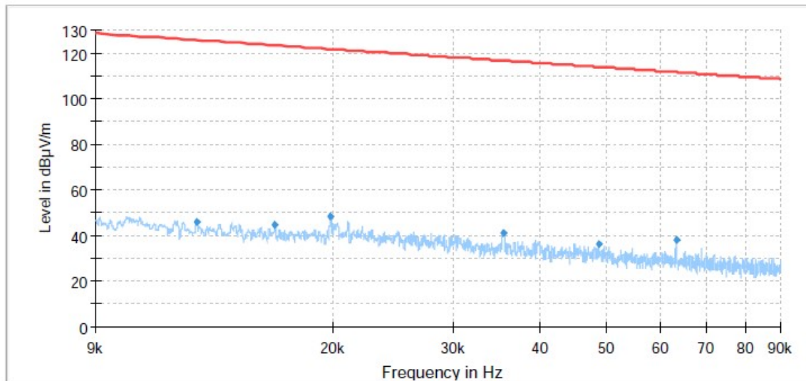
Band Edge from 9kHz to 90kHz
