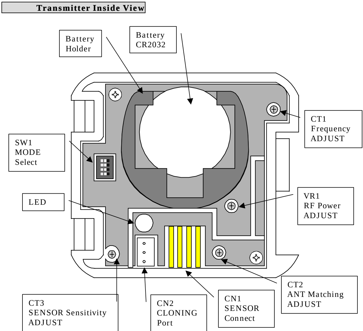
Fig.3-1 TRANSMITTER
