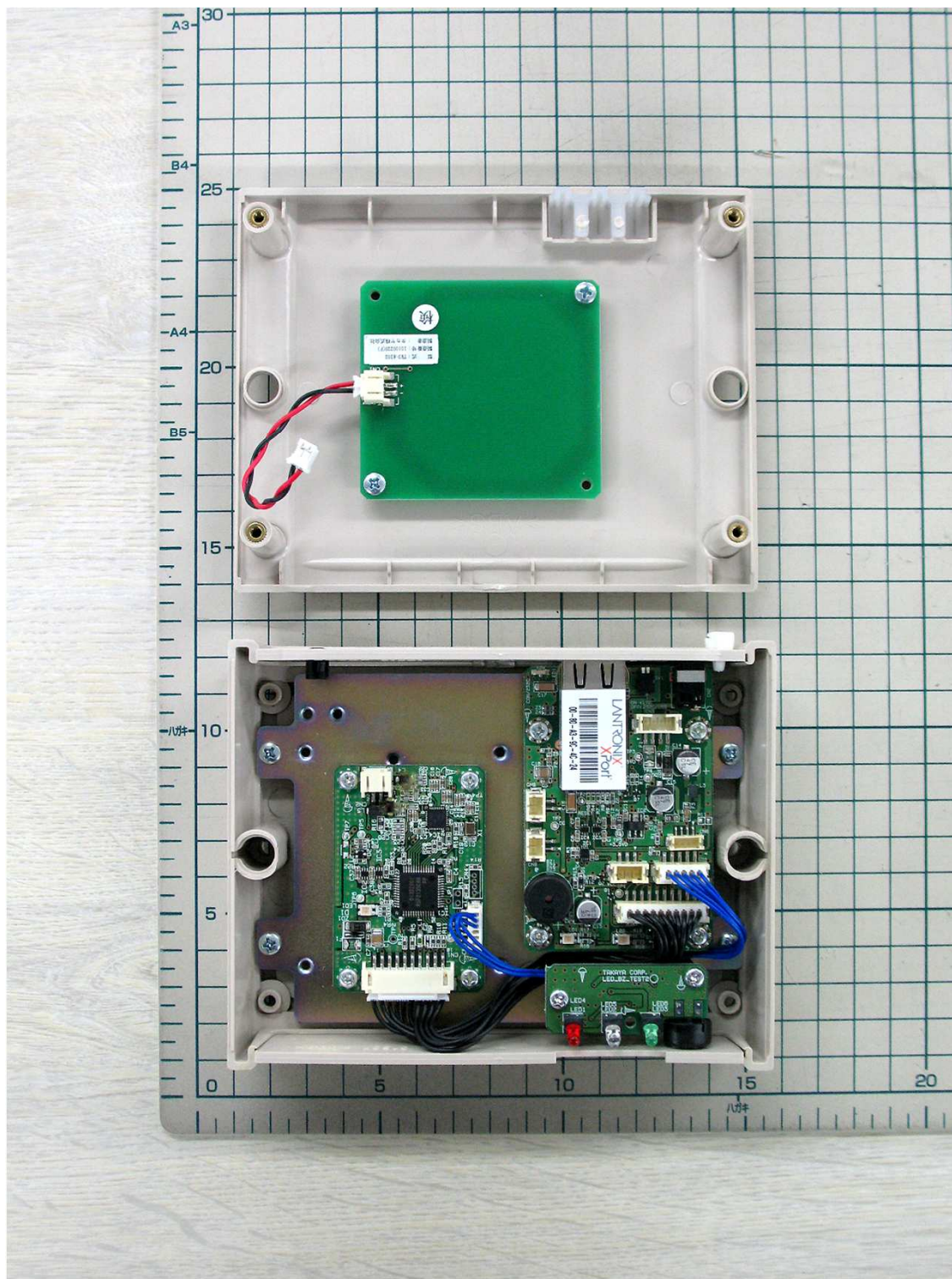
TR3XM-SN02 in Case
