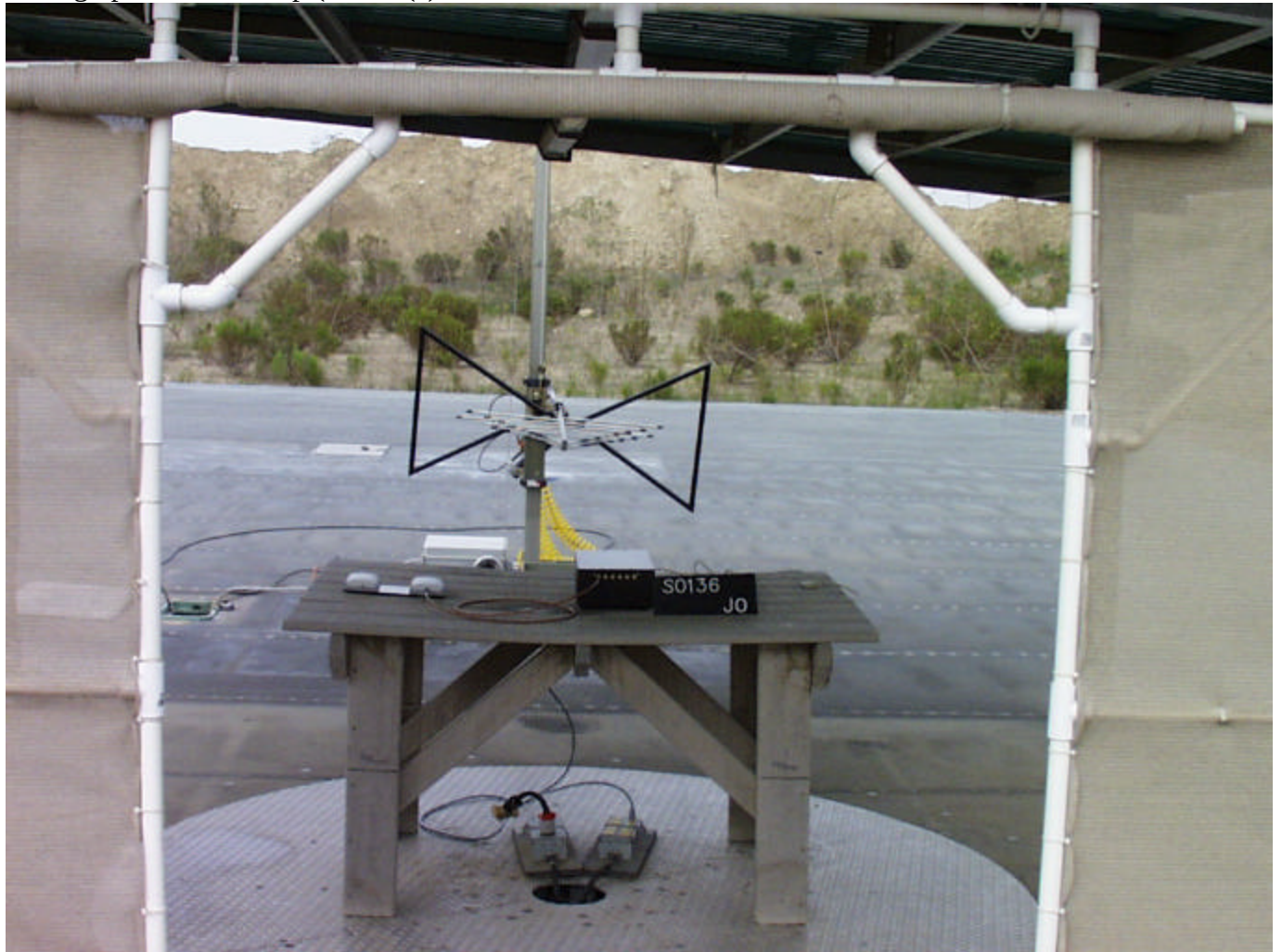
Photograph of Test Setup (15.209(a))
