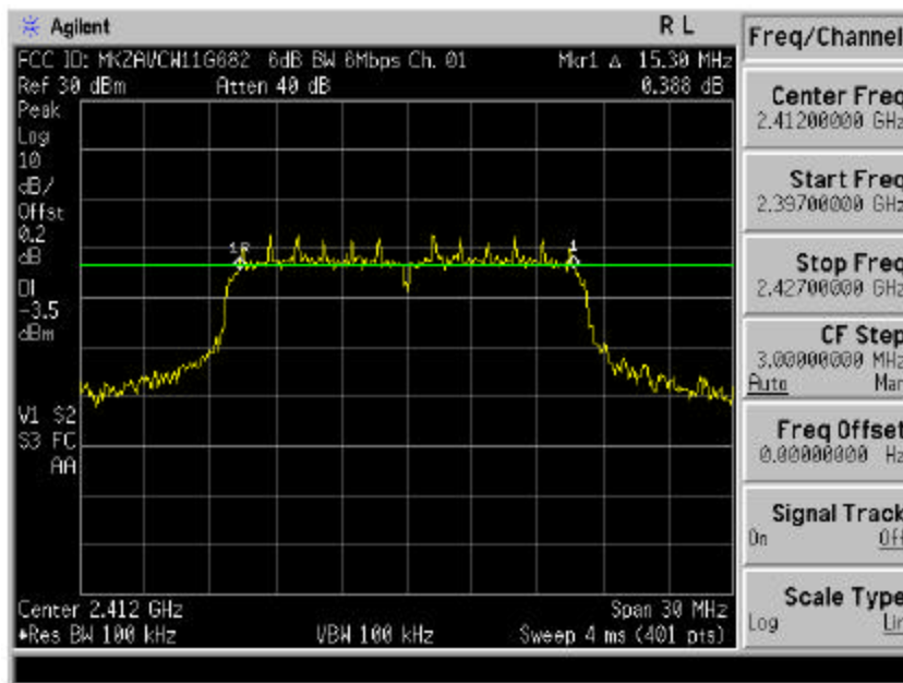
Plot A-1. 6dB 6Mbps Bandwidth Plot – Ch. 01
