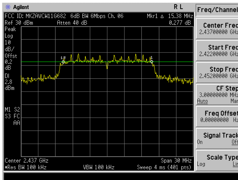
Plot A-2. 6dB 6Mbps Bandwidth Plot – Ch. 06
