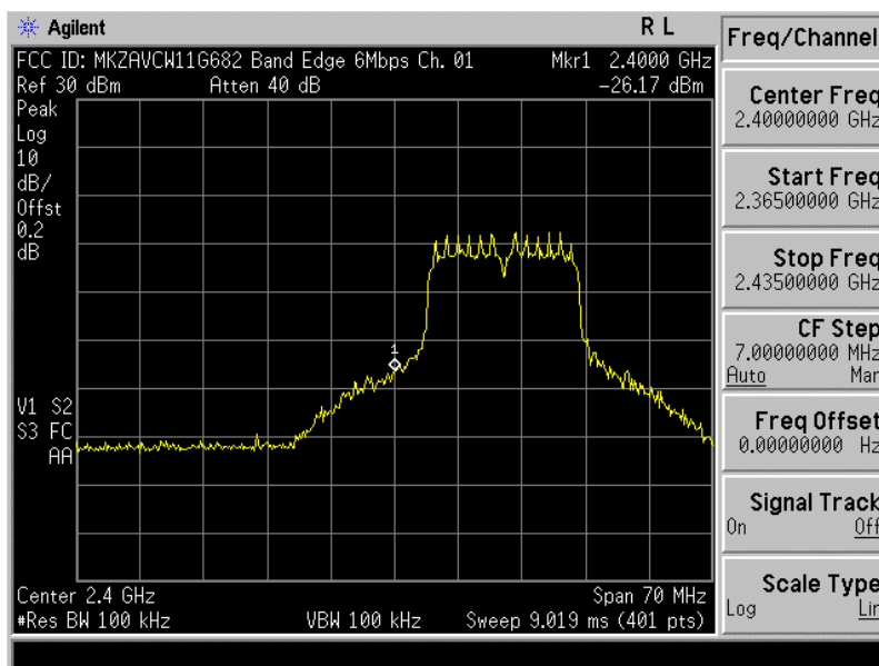
Plot A-10. Occupied Band Edge 6Mbps Plot – Ch. 01
