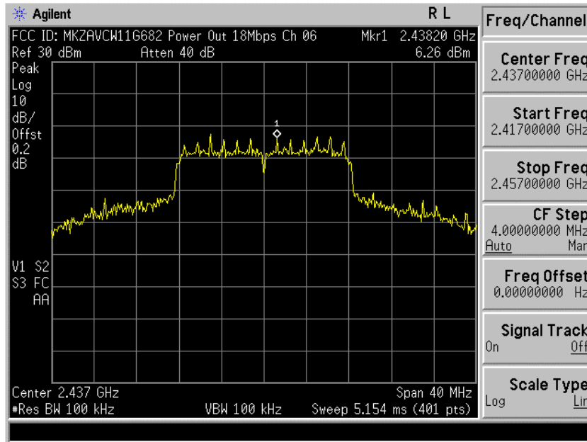
Plot A-5. Max. Output Power 18Mbps Plot – Ch. 06
