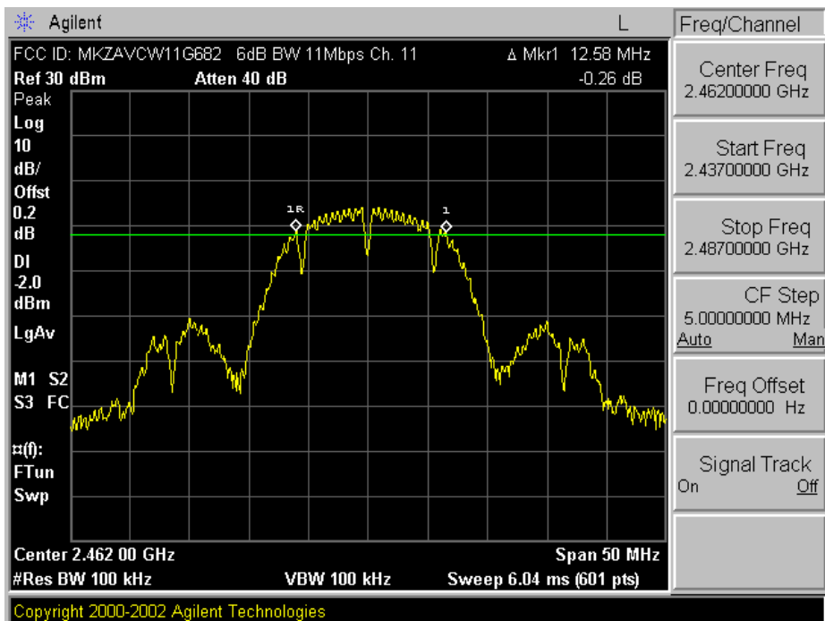
Plot A-3. 6dB 11Mbps Bandwidth Plot – Ch. 11
