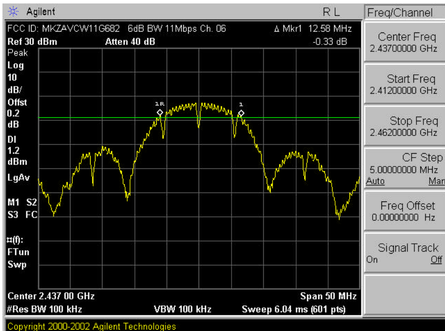
Plot A-2. 6dB 11Mbps Bandwidth Plot – Ch. 06
