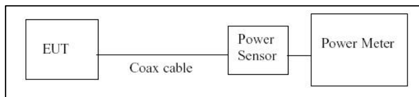
Figure A-3. Test Instrument & Measurement Setup
