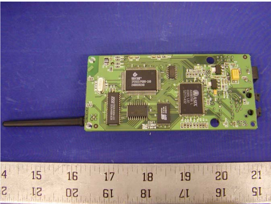
EUT – Component View with Antenna
