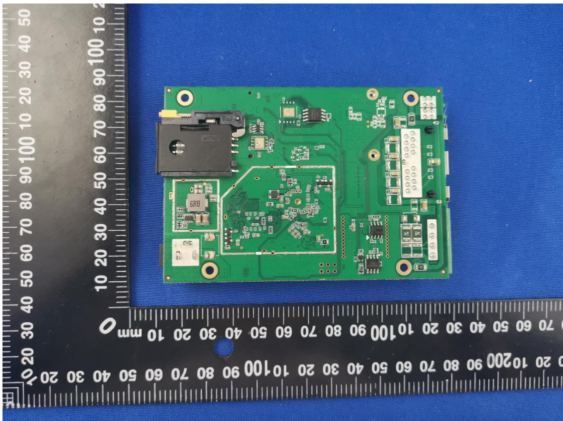
MAIN BOARD BACK VIEW (WITHOUT SHIELDING)
