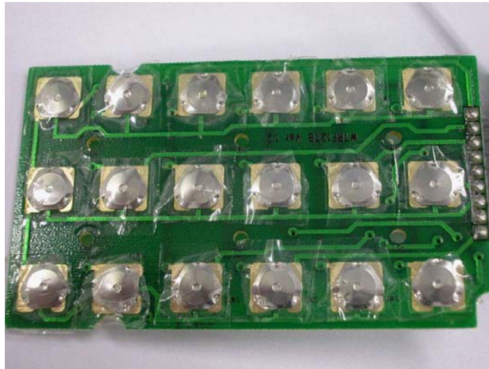
Internal Photo - 5
