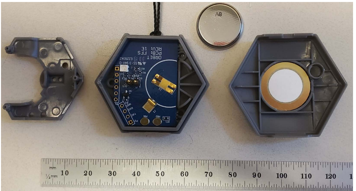
PCBA Cover Removed
