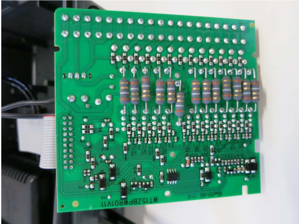
Switch Board bottom side
