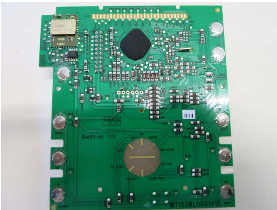
Base unit Main PCB top side
